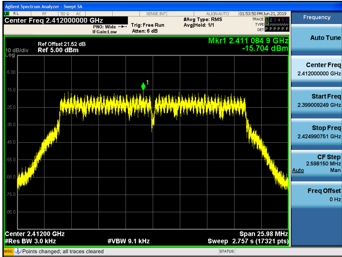
Power Spectral Density (802.11n_HT20 -CH 1)
