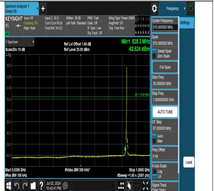
Band5-3MHz-QPSK-20525-1RB#14-30~1000-PASS
