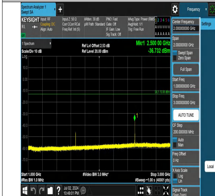
Band5-10MHz-QPSK-20450-1RB#49-1000~3000-PASS
