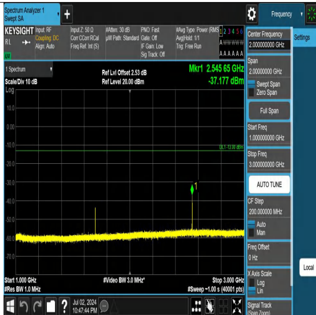
Band5-5MHz-QPSK-20625-1RB#24-1000~3000-PASS
