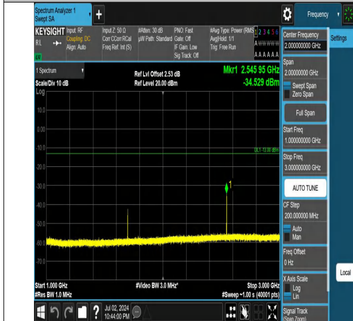
Band5-3MHz-QPSK-20635-1RB#14-1000~3000-PASS
