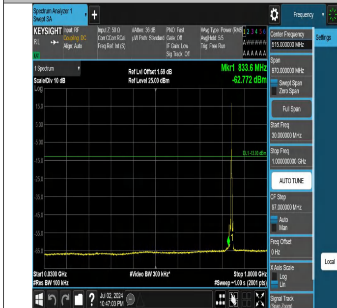
Band5-5MHz-QPSK-20625-1RB#0-30~1000-PASS
