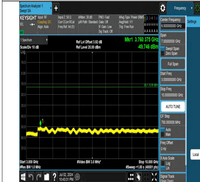
Band5-3MHz-QPSK-20635-1RB#0-3000~10000-PASS
