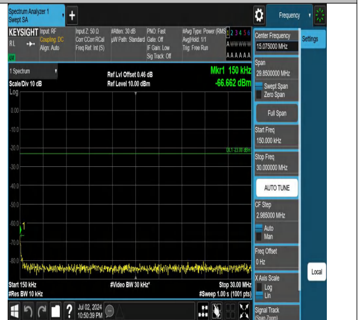
Band5-10MHz-QPSK-20600-1RB#0-0.15~30-PASS
