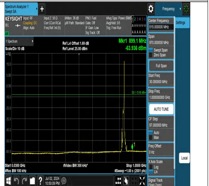
Band5-10MHz-QPSK-20525-1RB#49-30~1000-PASS
