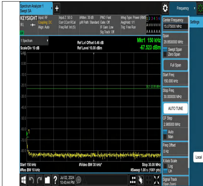
Band5-3MHz-QPSK-20635-1RB#14-0.15~30-PASS
