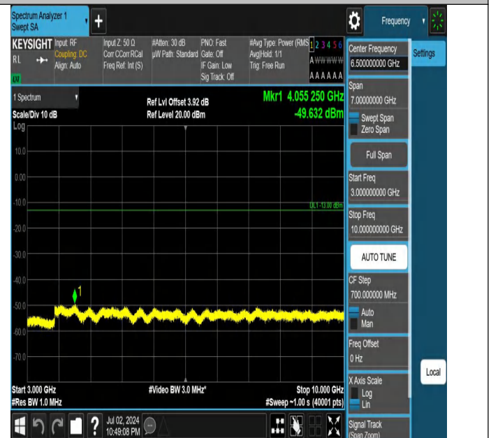
Band5-10MHz-QPSK-20450-1RB#49-3000~10000-PASS
