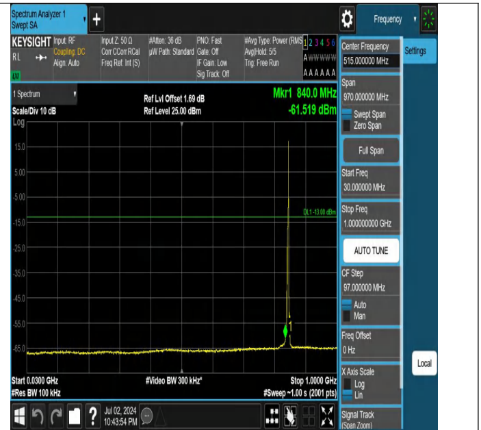
Band5-3MHz-QPSK-20635-1RB#14-30~1000-PASS
