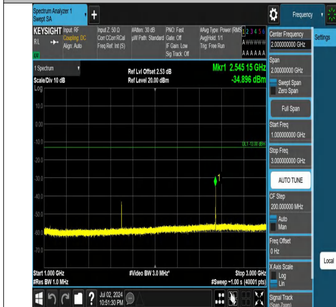
Band5-10MHz-QPSK-20600-1RB#49-1000~3000-PASS
