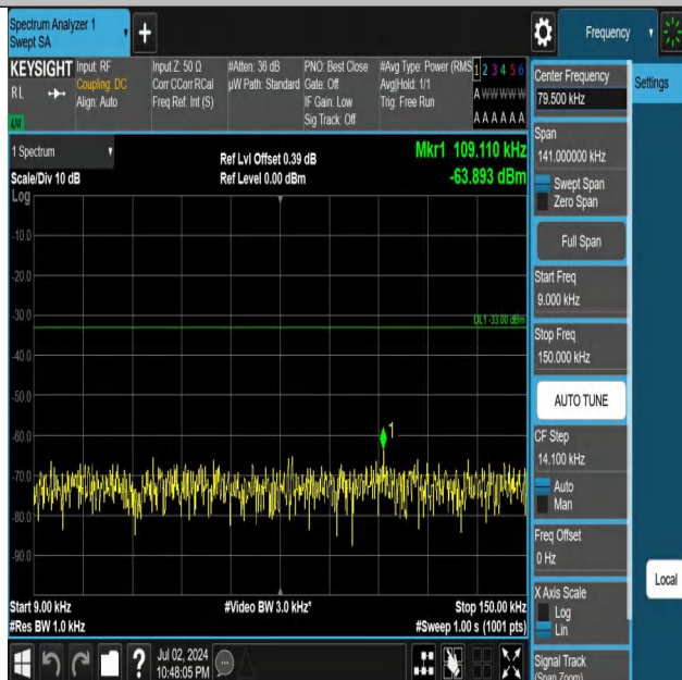
Band5-10MHz-QPSK-20450-1RB#0-0.009~0.15-PASS
