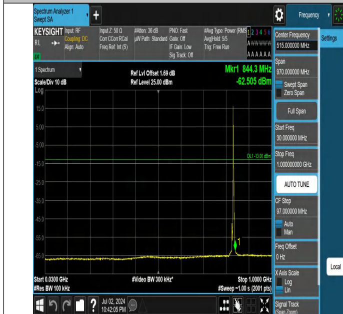
Band5-3MHz-QPSK-20525-1RB#0-30~1000-PASS
