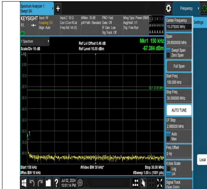
Band5-10MHz-QPSK-20600-1RB#49-0.15~30-PASS
