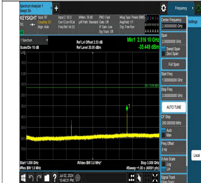
Band5-5MHz-QPSK-20525-1RB#24-1000~3000-PASS
