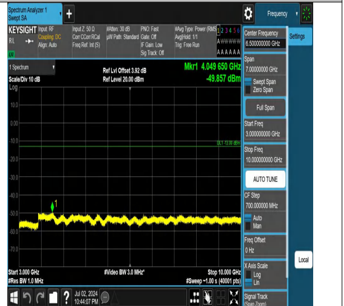
Band5-3MHz-QPSK-20635-1RB#14-3000~10000-PASS
