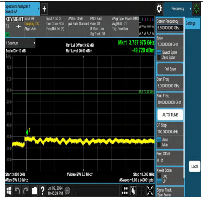
Band5-5MHz-QPSK-20425-1RB#24-3000~10000-PASS
