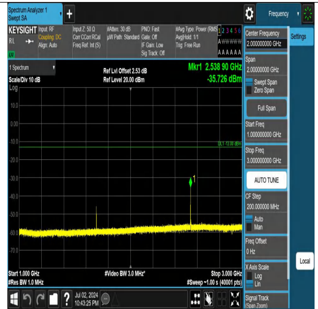
Band5-3MHz-QPSK-20635-1RB#0-1000~3000-PASS
