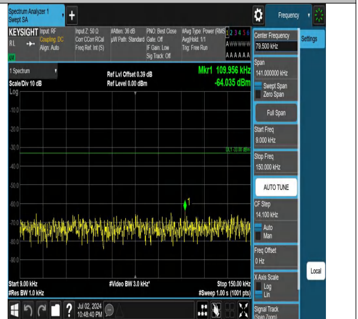
Band5-10MHz-QPSK-20450-1RB#49-0.009~0.15-PASS
