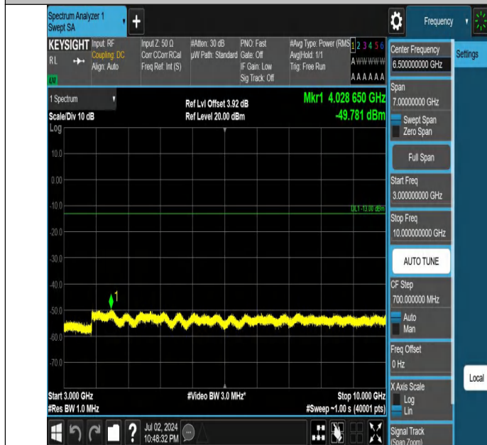
Band5-10MHz-QPSK-20450-1RB#0-3000~10000-PASS
