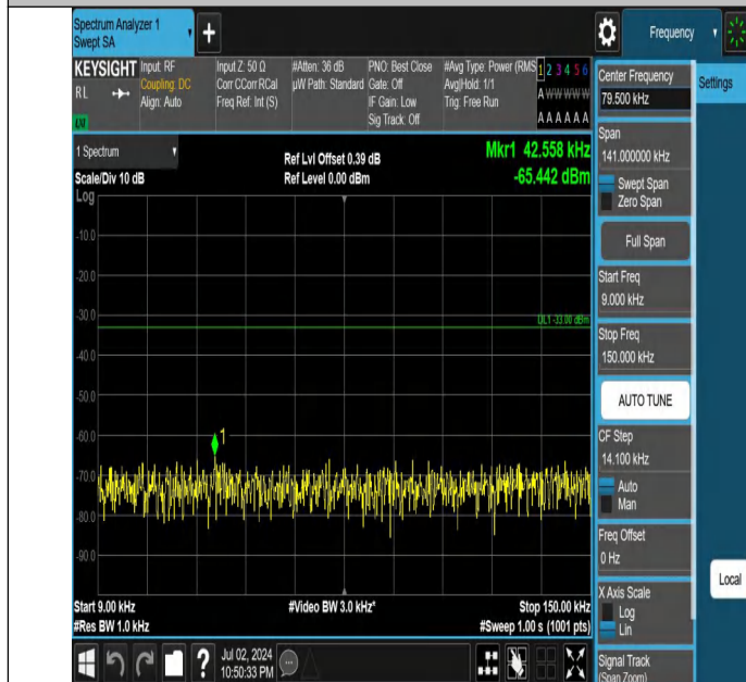
Band5-10MHz-QPSK-20600-1RB#0-0.009~0.15-PASS
