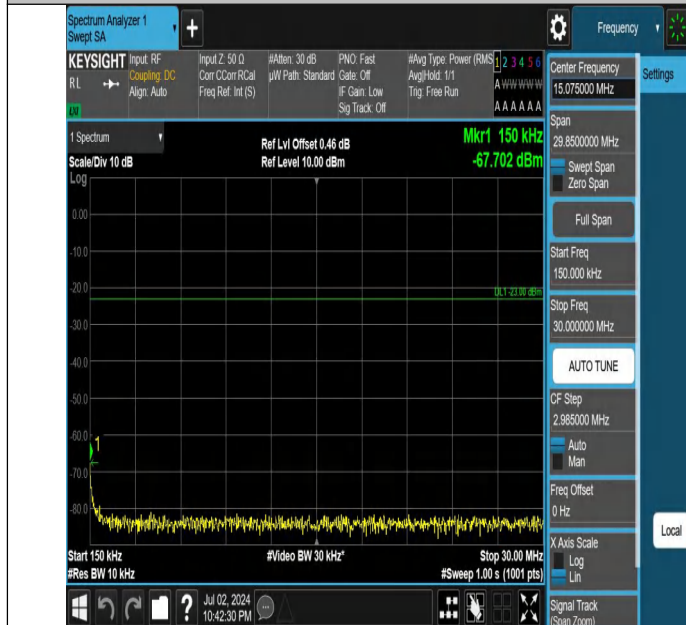
Band5-3MHz-QPSK-20525-1RB#14-0.15~30-PASS
