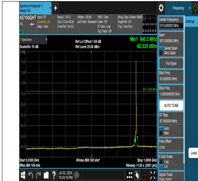
Band5-3MHz-QPSK-20635-1RB#0-30~1000-PASS
