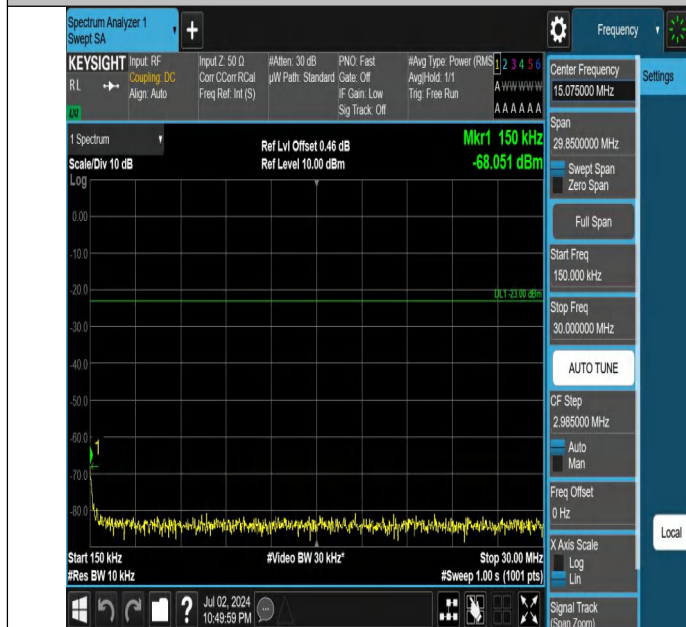
Band5-10MHz-QPSK-20525-1RB#49-0.15~30-PASS
