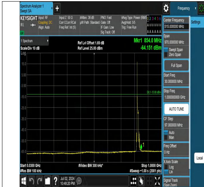
Band5-10MHz-QPSK-20450-1RB#0-30~1000-PASS
