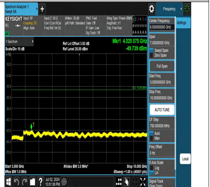
Band5-10MHz-QPSK-20600-1RB#49-3000~10000-PASS
