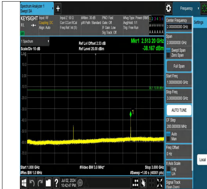
Band5-3MHz-QPSK-20525-1RB#14-1000~3000-PASS
