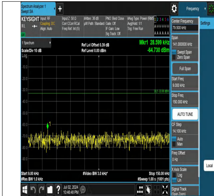
Band5-5MHz-QPSK-20625-1RB#0-0.009~0.15-PASS
