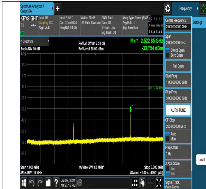
Band5-10MHz-QPSK-20525-1RB#49-1000~3000-PASS
