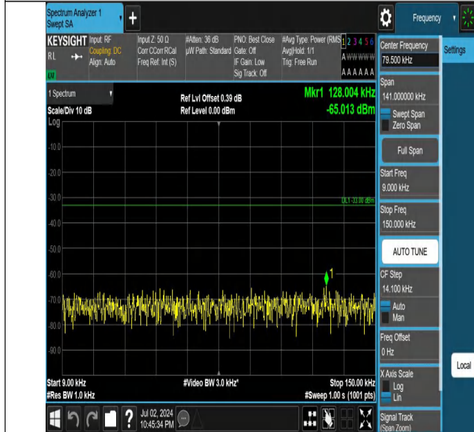
Band5-5MHz-QPSK-20525-1RB#0-0.009~0.15-PASS
