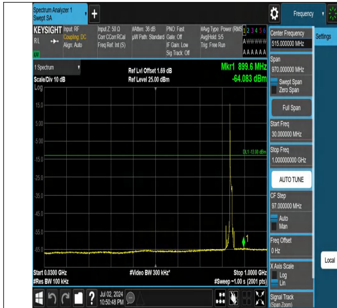
Band5-10MHz-QPSK-20600-1RB#0-30~1000-PASS
