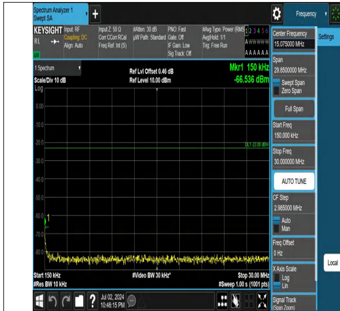
Band5-5MHz-QPSK-20525-1RB#24-0.15~30-PASS
