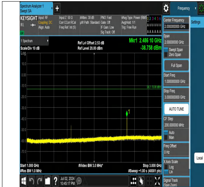
Band5-5MHz-QPSK-20425-1RB#24-1000~3000-PASS
