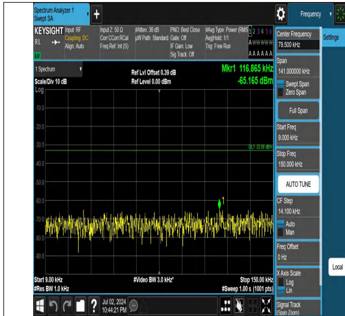
Band5-5MHz-QPSK-20425-1RB#0-0.009~0.15-PASS
