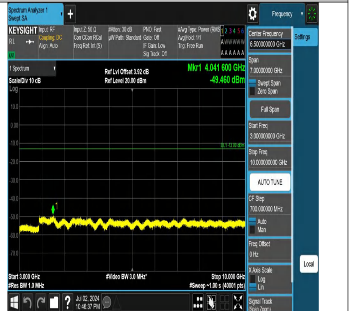
Band5-5MHz-QPSK-20525-1RB#24-3000~10000-PASS
