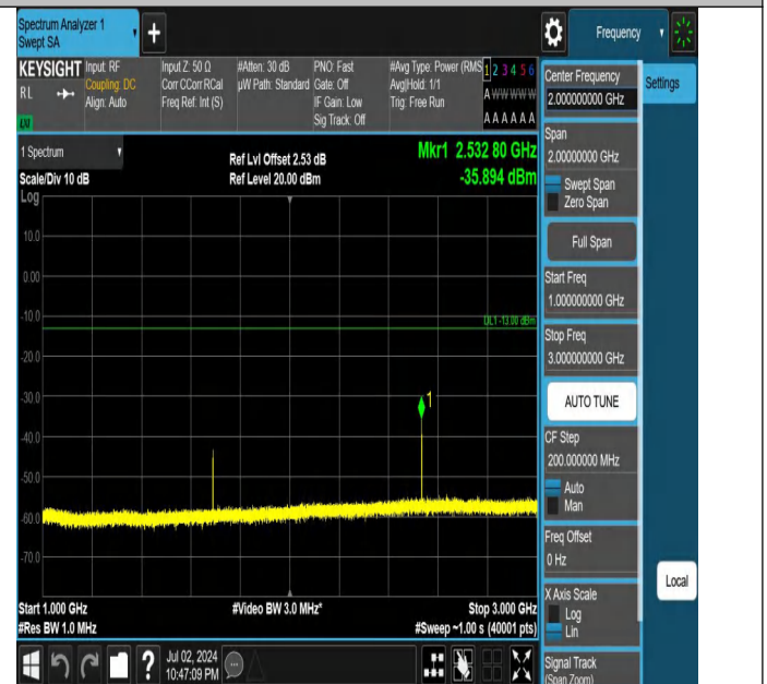
Band5-5MHz-QPSK-20625-1RB#0-1000~3000-PASS
