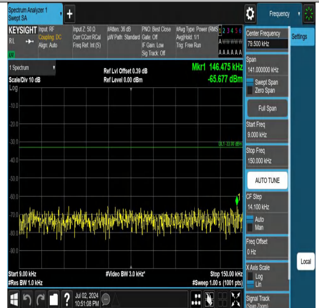
Band5-10MHz-QPSK-20600-1RB#49-0.009~0.15-PASS
