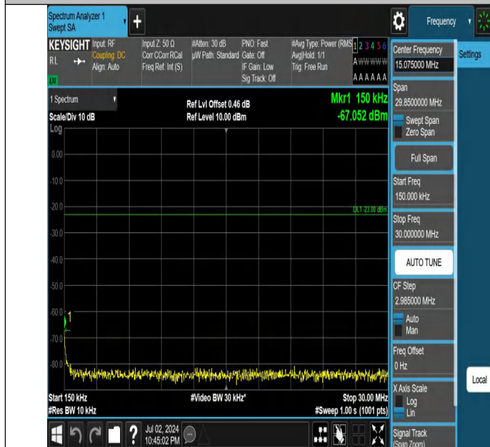
Band5-5MHz-QPSK-20425-1RB#24-0.15~30-PASS
