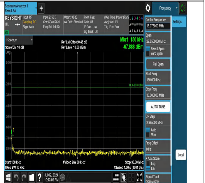
Band5-3MHz-QPSK-20635-1RB#0-0.15~30-PASS
