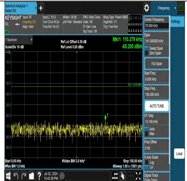
Band5-3MHz-QPSK-20635-1RB#14-0.009~0.15-PASS
