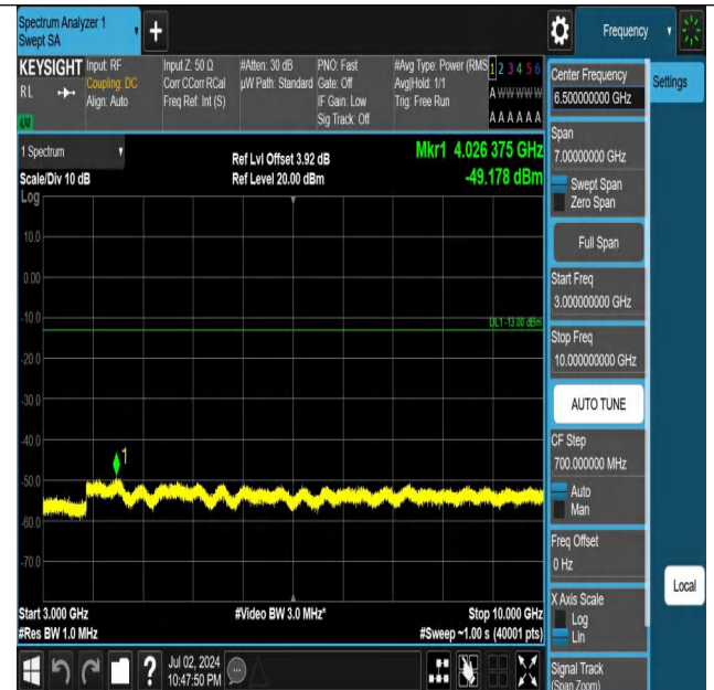
Band5-5MHz-QPSK-20625-1RB#24-3000~10000-PASS
