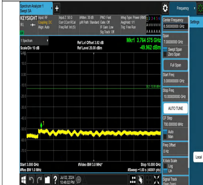
Band5-5MHz-QPSK-20525-1RB#0-3000~10000-PASS
