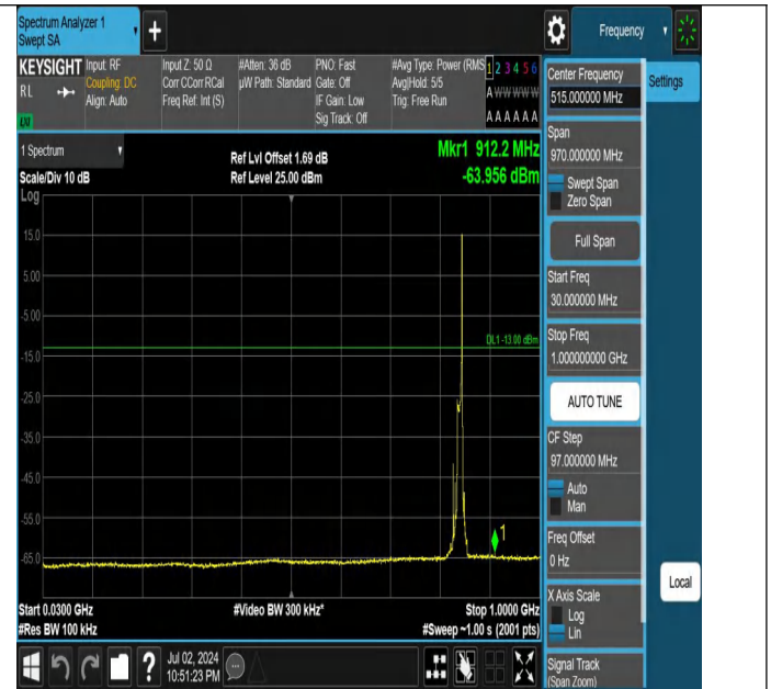
Band5-10MHz-QPSK-20600-1RB#49-30~1000-PASS
