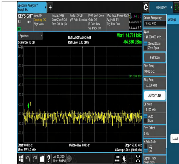
Band5-3MHz-QPSK-20525-1RB#0-0.009~0.15-PASS
