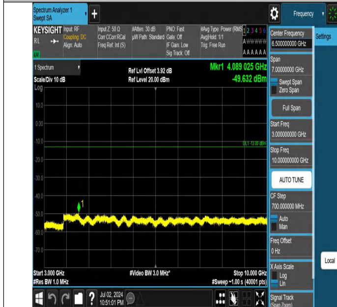
Band5-10MHz-QPSK-20600-1RB#0-3000~10000-PASS
