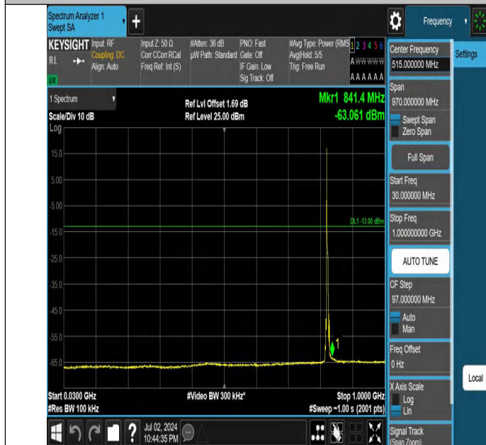
Band5-5MHz-QPSK-20425-1RB#0-30~1000-PASS
