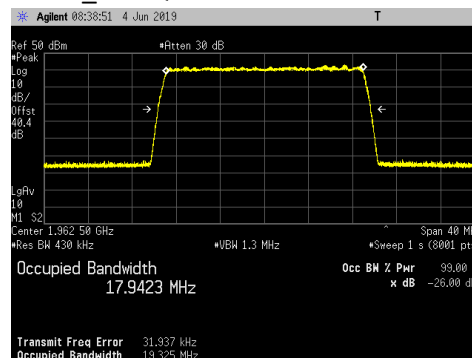
LTE20_256QAM
