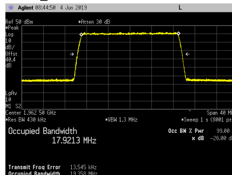
LTE20_QPSK
