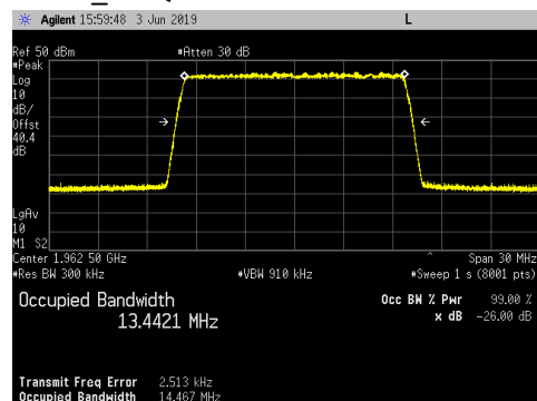
LTE15_64QAM
