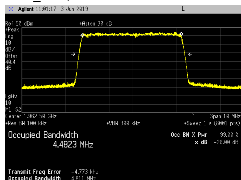
LTE5_16QAM
