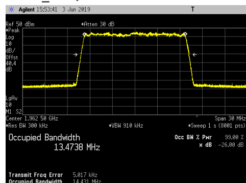
LTE15_16QAM
