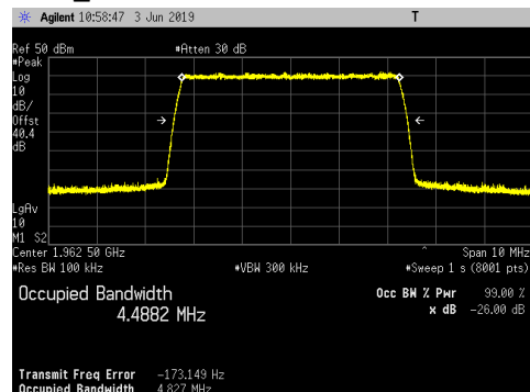
LTE5_QPSK
