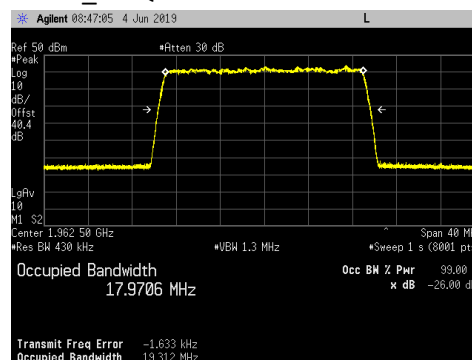
LTE20_16QAM
