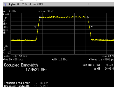
LTE20_64QAM
