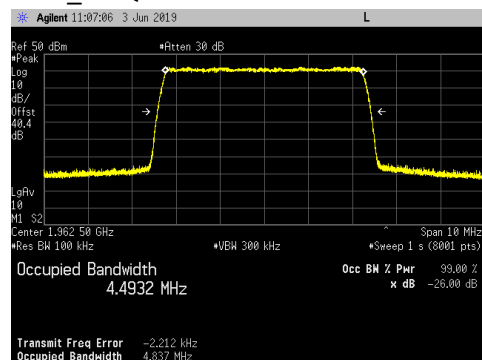
LTE5_64QAM
