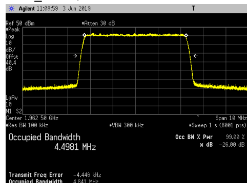
LTE5_256QAM
