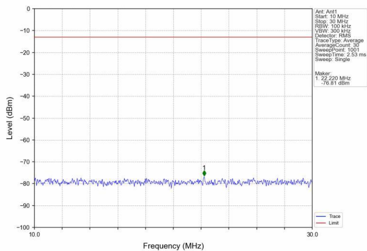
Band26a_5MHz_QPSK_HCH_821.5MHz_RB_1_0_NTNV
