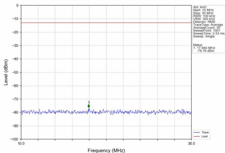
Band26a 3MHz 16QAM MCH 819MHz RB 1 0 NTNV
