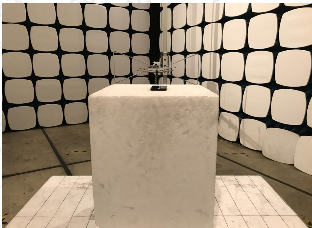
RADIATED EMISSION TEST SETUP
