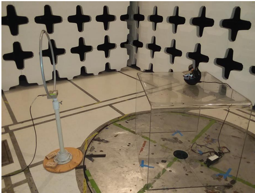
Figure 2: Radiated Emissions Setup Below 30 MHz-parallel
