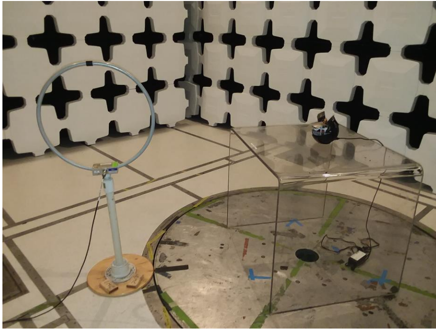
Figure 3: Radiated Emissions Setup Below 30MHz-perpendicular
