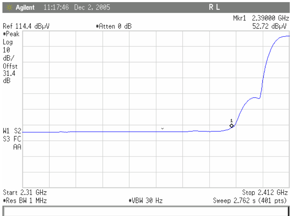
Plot 2. 802.11/b radiated restricted band 2310- 2390 MHz Avg
