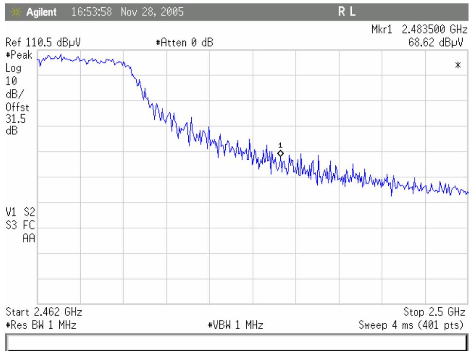
Plot 7. 802.11/g radiated restricted band 2483.5 – 2500MHz Peak
