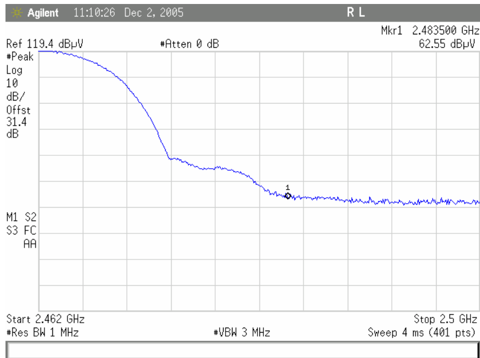
Plot 3. 802.11/b radiated restricted band 2483.5 – 2500MHz Peak
