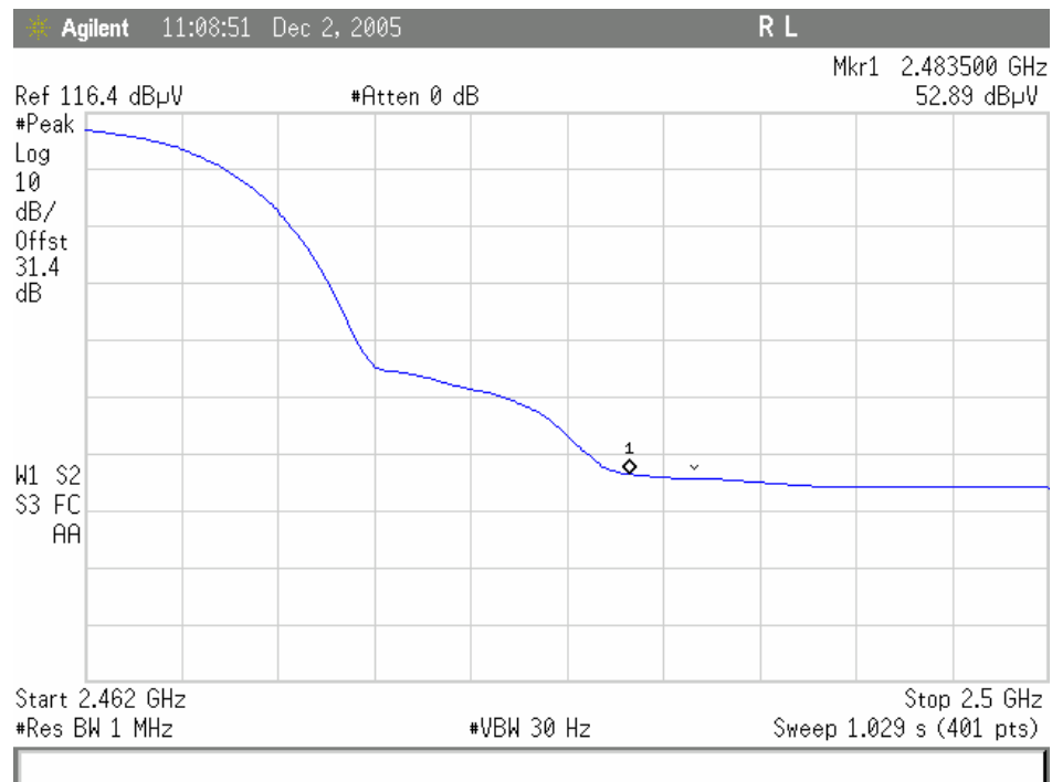
Plot 4. 802.11/b radiated restricted band 2483.5 – 2500MHz Avg
