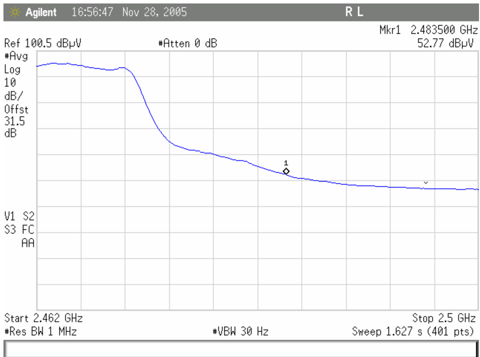
Plot 8. 802.11/g radiated restricted band 2483.5 – 2500MHz Avg
