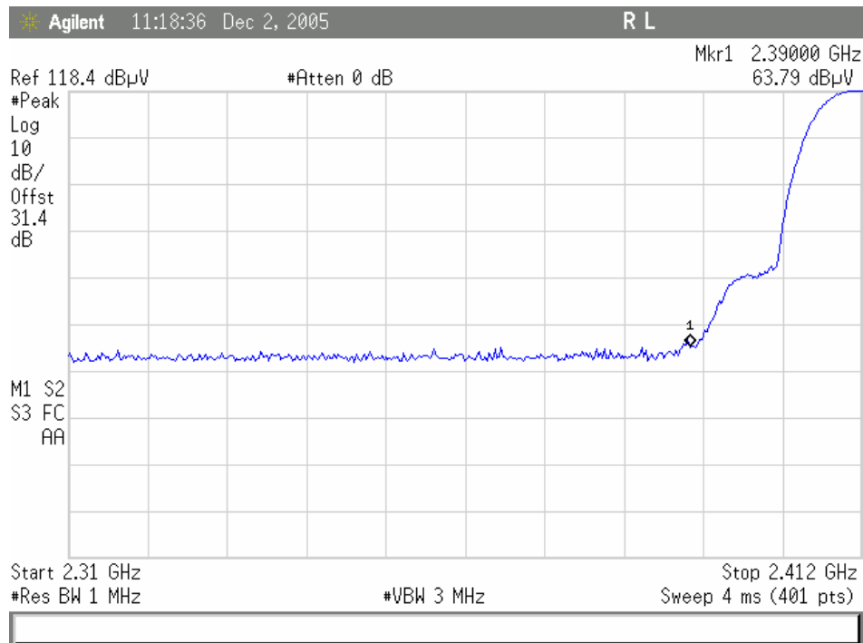
Plot 1. 802.11/b radiated restricted band 2310- 2390 MHz Peak
