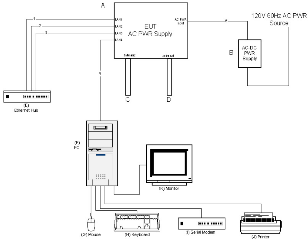
Figure 1. Block Diagram of Test Configuration (Radiated Emissions)
