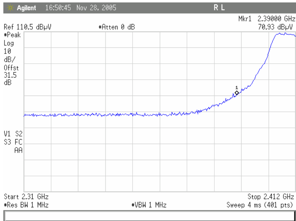
Plot 5. 802.11/g radiated restricted band 2310- 2390 MHz Peak
