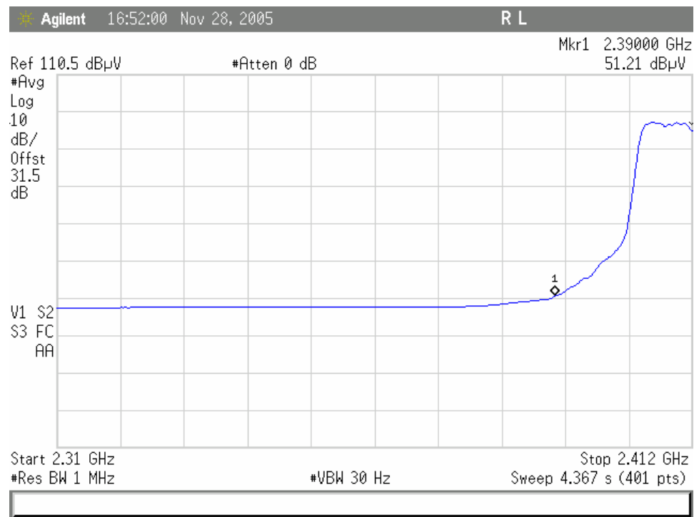
Plot 6. 802.11/g radiated restricted band 2310- 2390 MHz Avg
