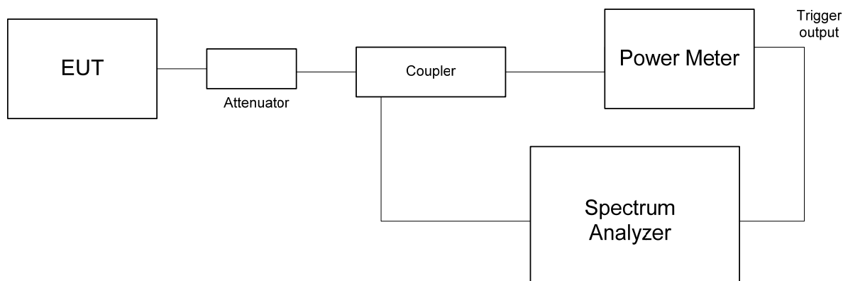
Figure 7.9.1 Spurious emission test setup for single output
