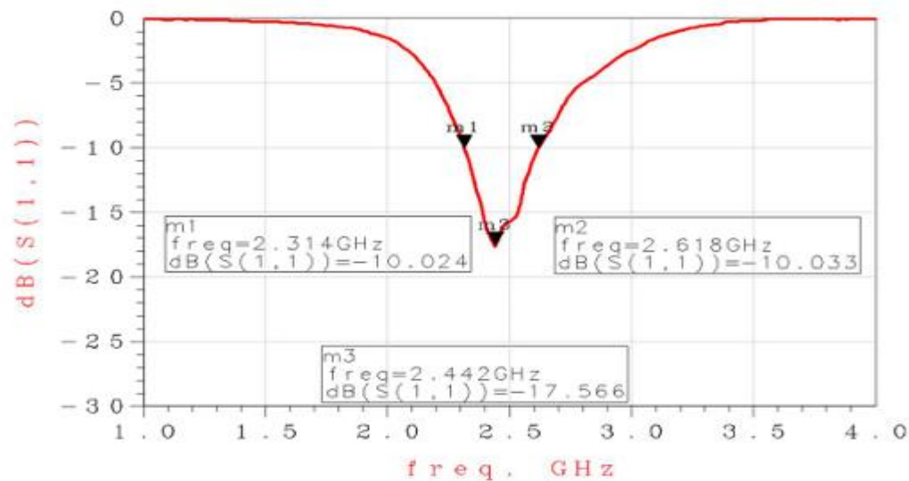
Return Loss
