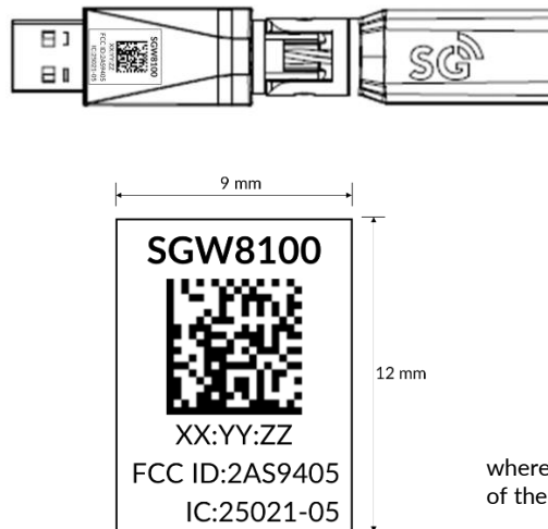
Figure 4: SGW8100 MAC Address Label
