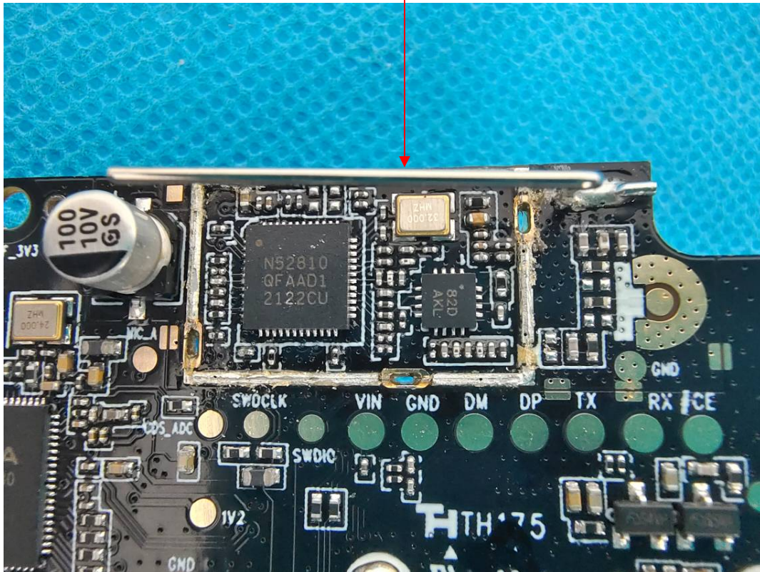
FHSS ANT
