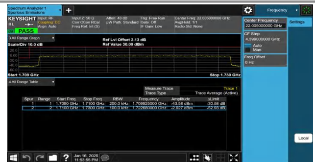
Band66-20MHz-QPSK-132072-100RB#0-PASS
