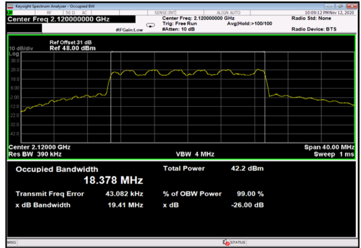
Figure 562: 16QAM 20MHz B.W.; 2120.0MHz, 30kHz - Output
