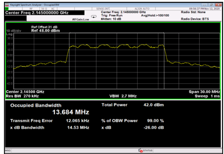
Figure 556: 16QAM 15MHz B.W.; 2145.0MHz, 30kHz - Output
