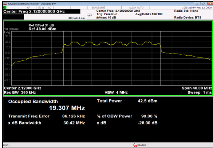
Figure 561: 16QAM 20MHz B.W.; 2120.0MHz, 15kHz - Output
