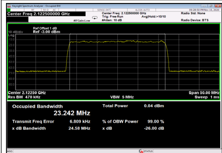
Figure 505: QPSK 25MHz B.W.; 2122.5MHz, 30kHz - Input
