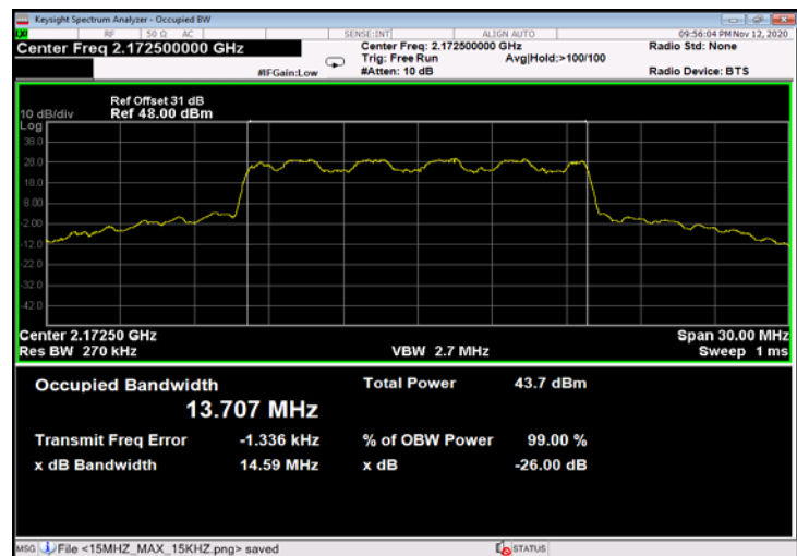
Figure 559: 16QAM 15MHz B.W.; 2172.5MHz, 30kHz - Output
