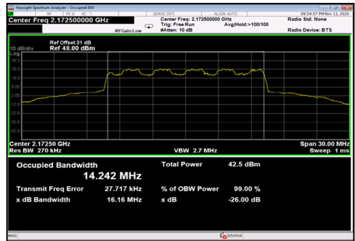
Figure 558: 16QAM 15MHz B.W.; 2172.5MHz, 15kHz - Output
