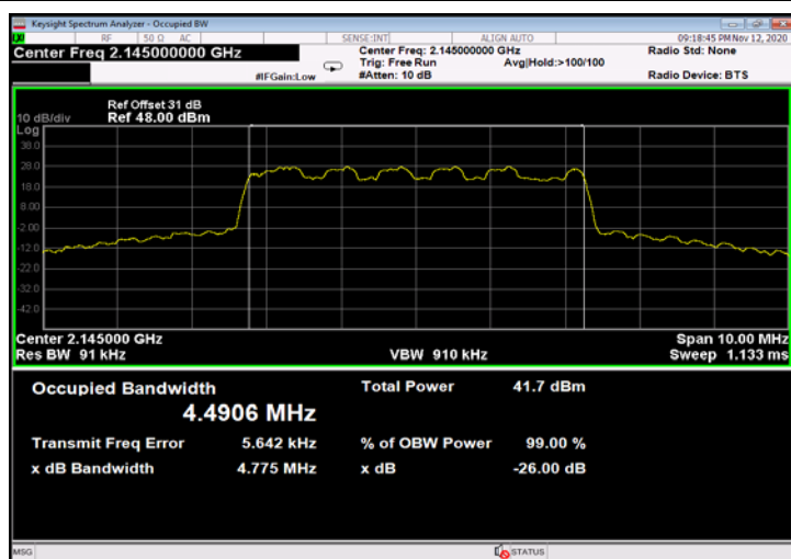
Figure 539: 16QAM 5MHz B.W.; 2145.0MHz, 15kHz - Output
