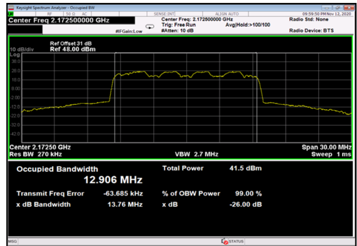
Figure 560: 16QAM 15MHz B.W.; 2172.5MHz, 60kHz - Output
