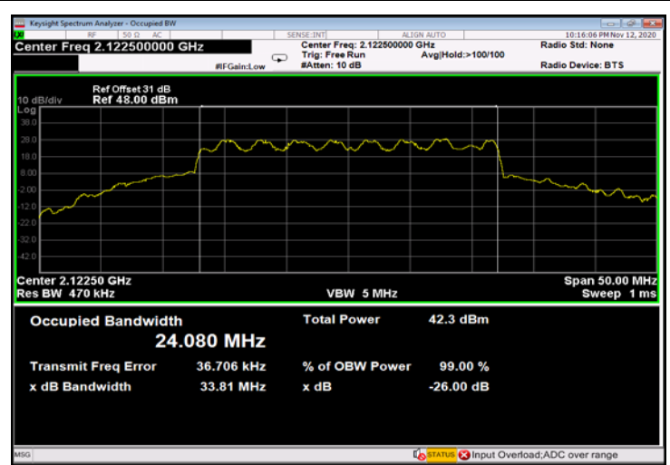
Figure 570: 16QAM 25MHz B.W.; 2122.5MHz, 15kHz - Output
