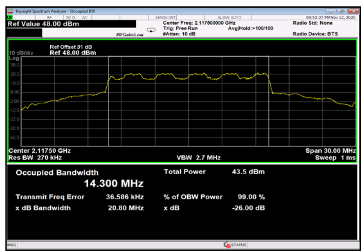
Figure 552: 16QAM 15MHz B.W.; 2117.5MHz, 15kHz - Output
