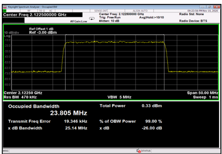
Figure 504: QPSK 25MHz B.W.; 2122.5MHz, 15kHz - Input
