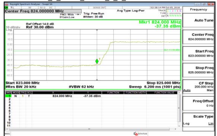
Band5_1_4MHz_QPSK_6_0_LowCH20407-824.7
