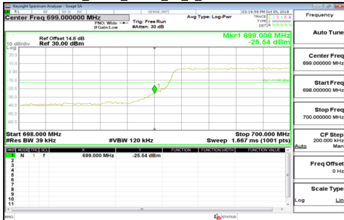
Band12_3MHz_QPSK_15_0_LowCH23025-700.5
