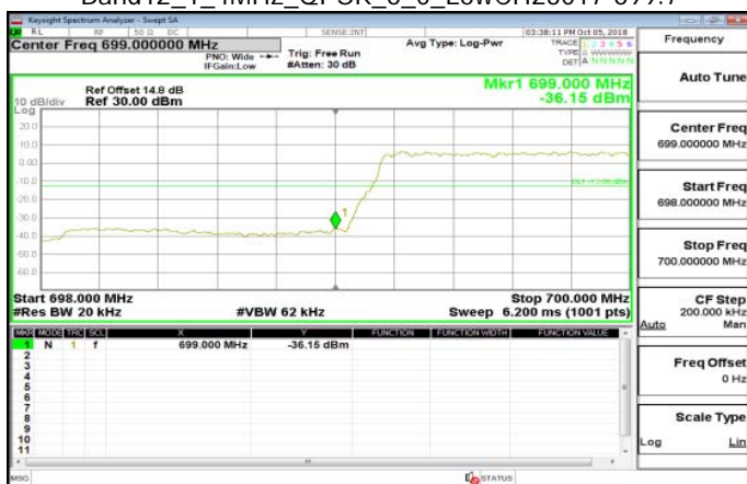
Band12_1_4MHz_QPSK_6_0_LowCH23017-699.7
