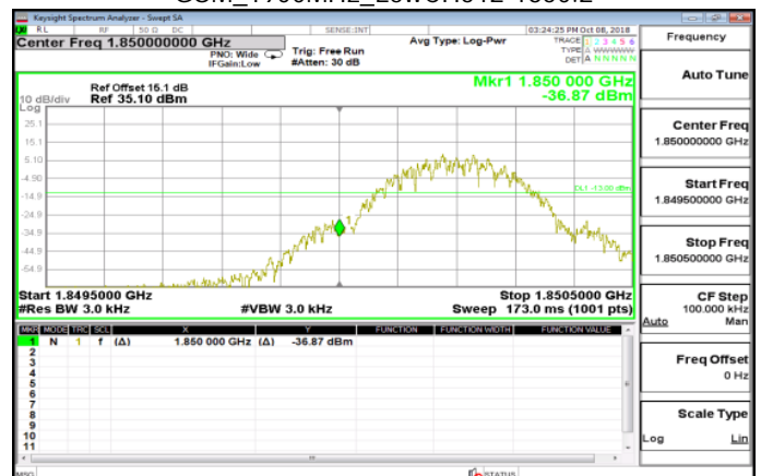
GSM_1900MHz_LowCH512-1850.2
