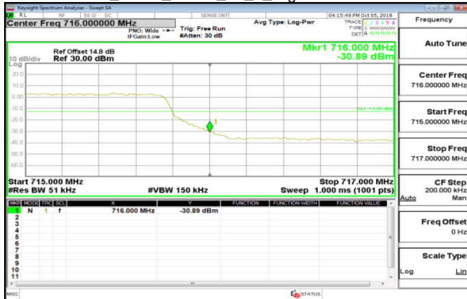
Band17_5MHz_QPSK_25_0_HighCH23825-713.5
