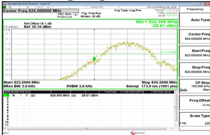
GSM_850MHz_LowCH128-824.2
