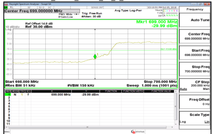
Band12_5MHz_QPSK_25_0_LowCH23035-701.5
