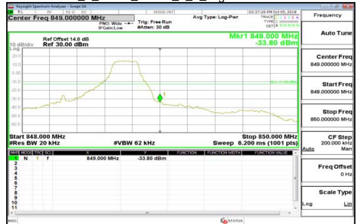
Band5_1_4MHz_QPSK_1_5_HighCH20643-848.3
