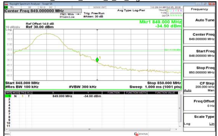
Band5_10MHz_QPSK_1_49_HighCH20600-844
