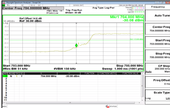
Band17_5MHz_QPSK_25_0_LowCH23755-706.5
