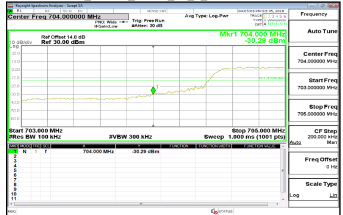
Band17_10MHz_QPSK_50_0_LowCH23780-709
