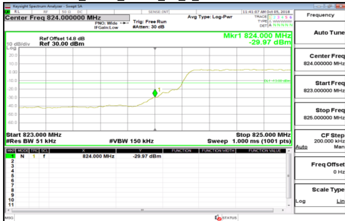
Band5_5MHz_QPSK_25_0_LowCH20425-826.5
