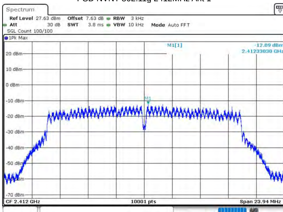
PSD NVNT 802.11g 2412MHz Ant 1
