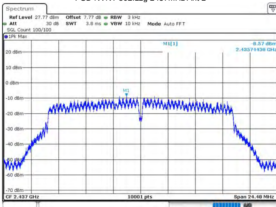
PSD NVNT 802.11g 2437MHz Ant 2
