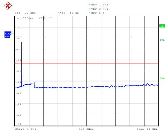
NB-IOT Band 2 CH-High 1GHz-20GHz
