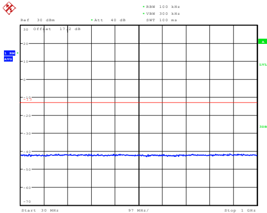
NB-IOT Band 2 CH-Middle 30MHz-1GHz
