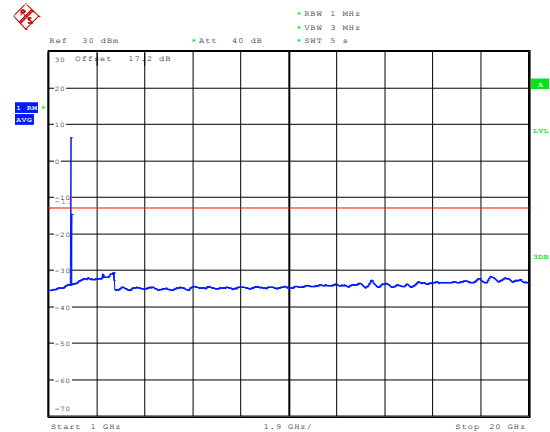
NB-IOT Band 2 CH-Middle 1GHz-20GHz
