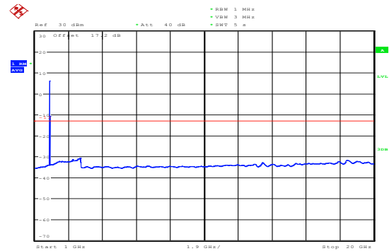
NB-IOT Band 2 CH-Low 1GHz-20GHz
