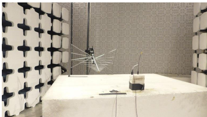
Figure B 1: ULXD1 Transmitter Test Setup
