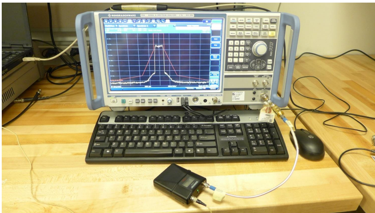
Figure A-1 - Test Setup for Minimum Bandwidth
