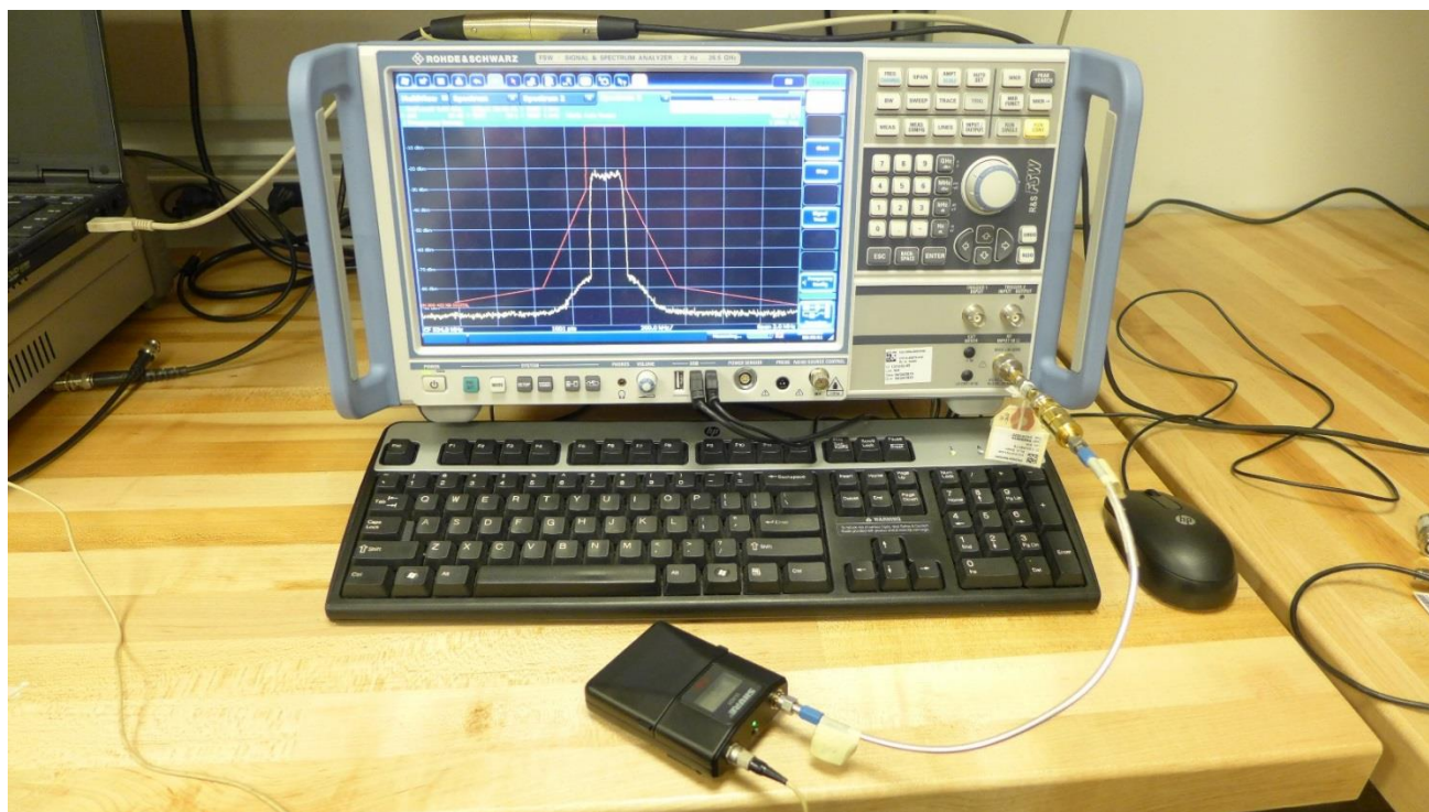
Figures E-1 - Test Setup for Spurious Emissions on Antenna Port
