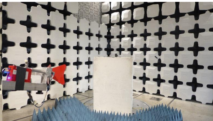
Figure B 2: ULXD1 Transmitter Test Setup
