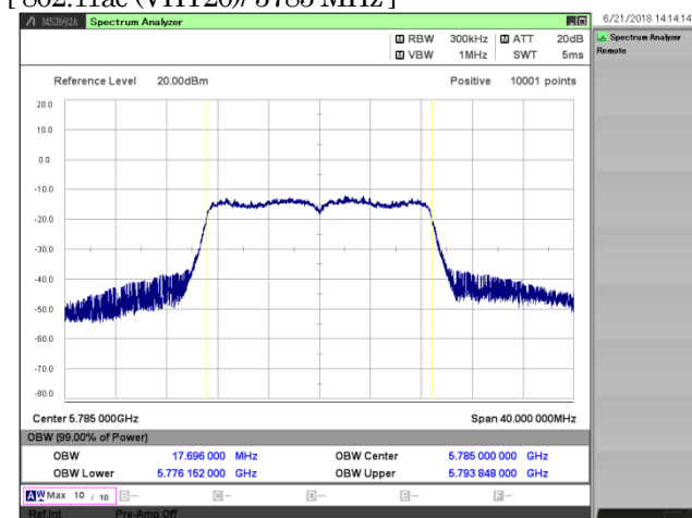
[ 802.11ac (VHT20)/ 5785 MHz ]
