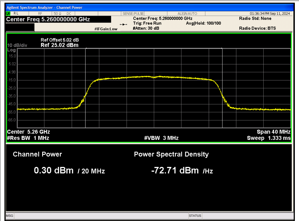
Power NVNT ac20 5260MHz Ant2
