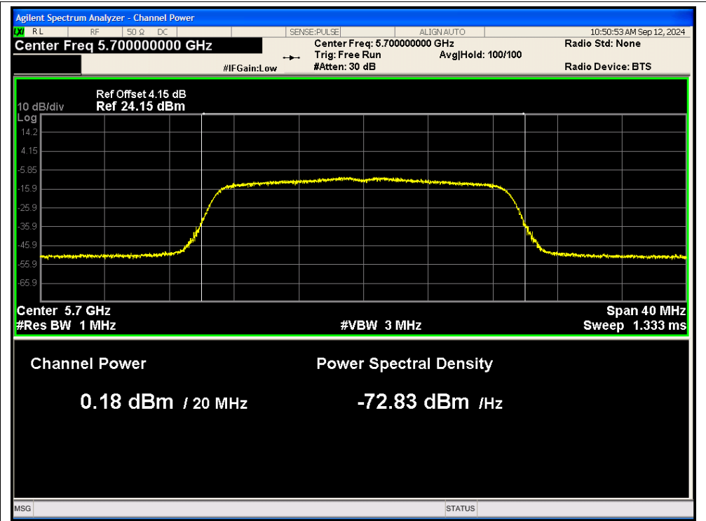
Power NVNT ac20 5700MHz Ant2
