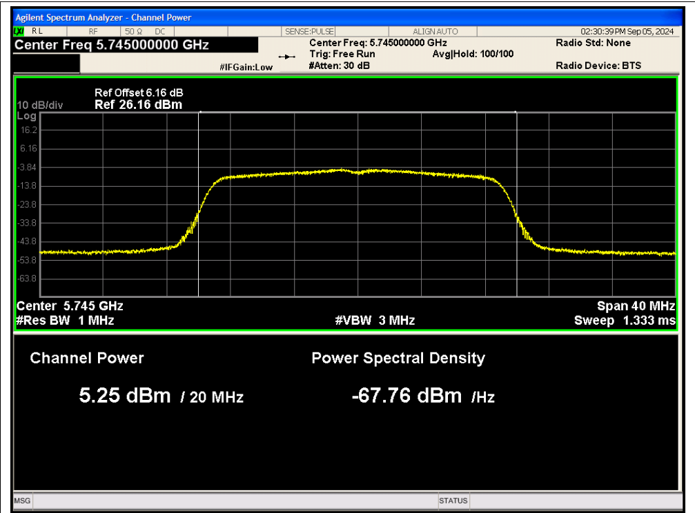
Power NVNT ac20 5745MHz Ant2
