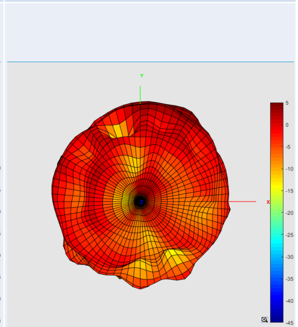
Z-axis View
