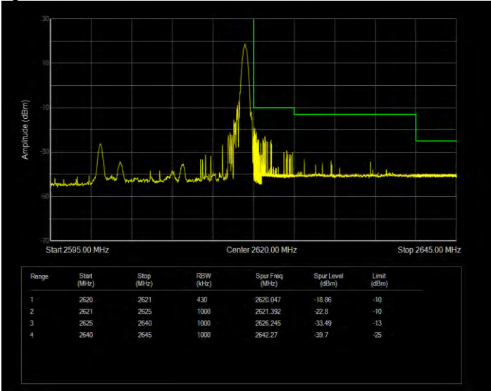
Band38 QPSK BW=20MHz Channel=38150 RB Size=100 Position=#0 Extended
