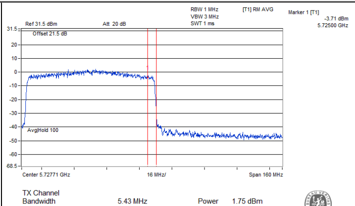
802.11ax (HE80) CDD / Chain 2 : CH 138 (U-NII-3)
