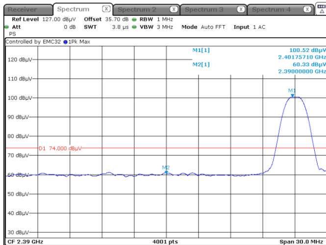
Figure 7.7-10: Band edge spurious emissions at 2390 MHz Peak
