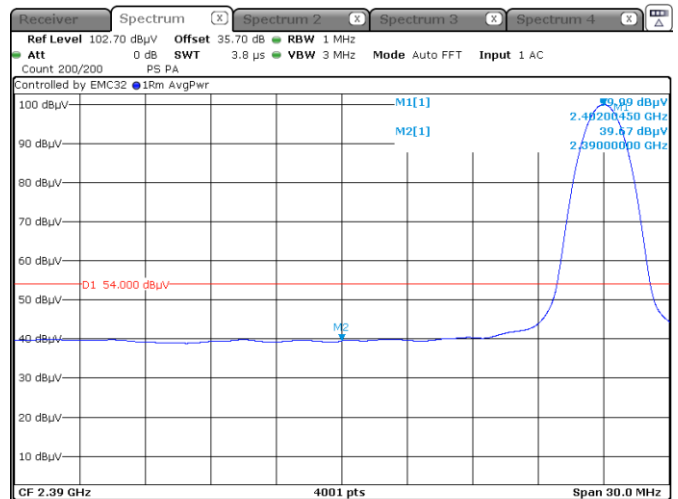
Figure 7.7-11: Band edge spurious emissions at 2390 MHz Average
