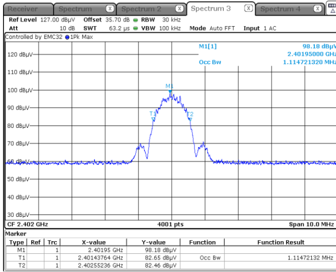
Figure 7.5-4: 99% occupied bandwidth on low ch.
