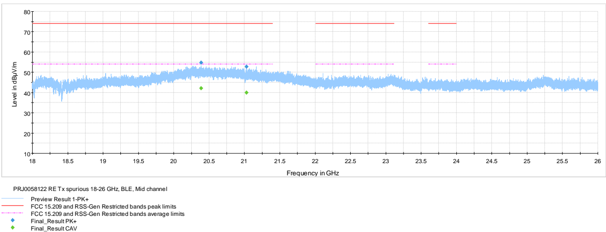
Figure 7.7-8: Radiated spurious emissions 18-26 GHz mid channel
