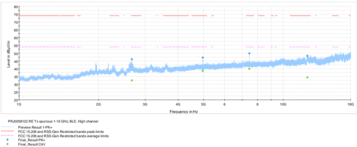
Figure 7.7-6: Radiated spurious emissions 1-18 GHz high channel
