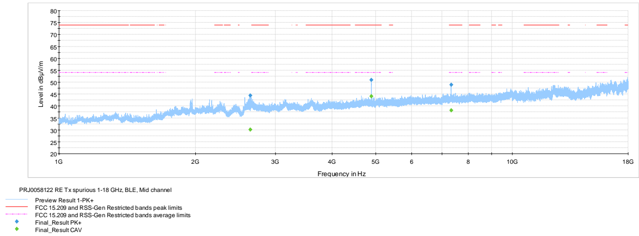
Figure 7.7-5: Radiated spurious emissions 1-18 GHz mid channel
