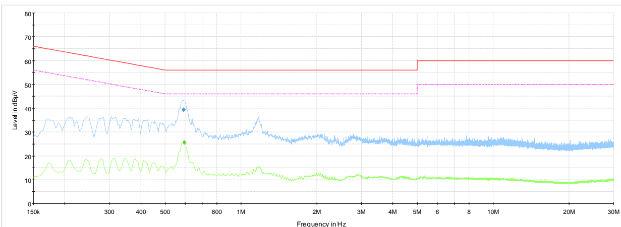
Plot 7.4-1: Conducted emissions on phase line
