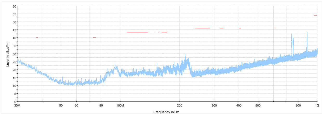
Figure 7.7-1: Radiated spurious emissions 30-1000 MHz low channel
