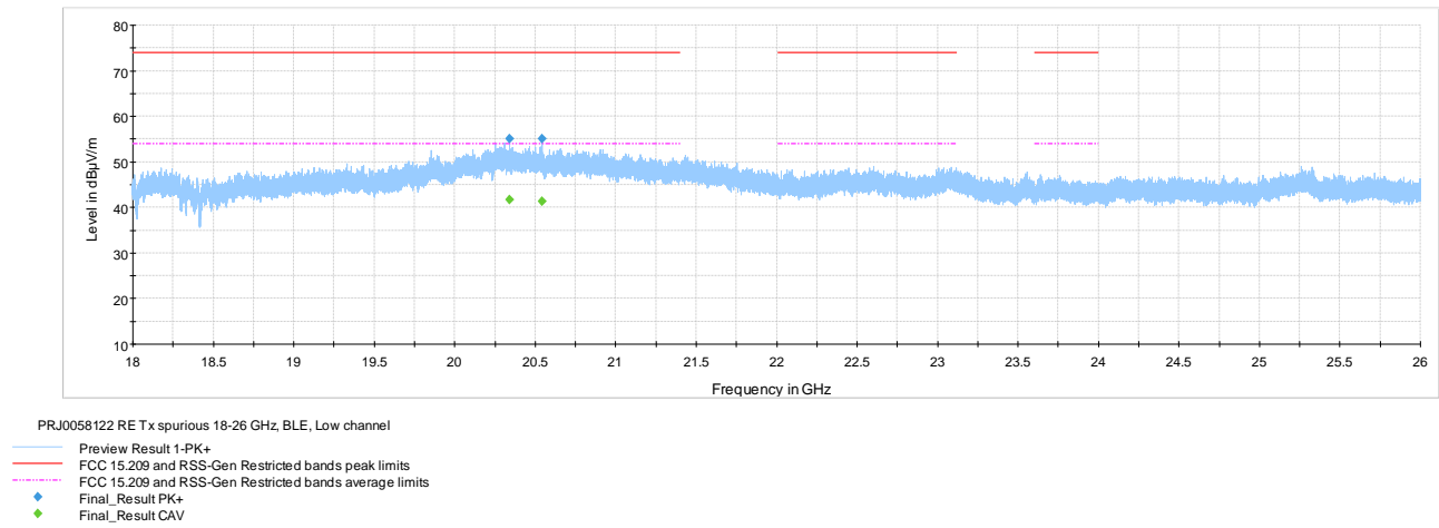
Figure 7.7-7: Radiated spurious emissions 18-26 GHz low channel
