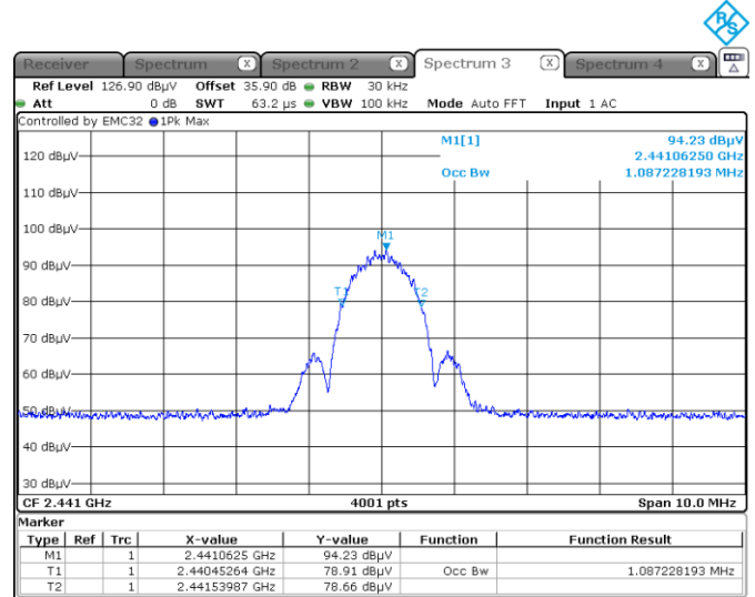
Figure 7.5-5: 99% occupied bandwidth on mid ch.
