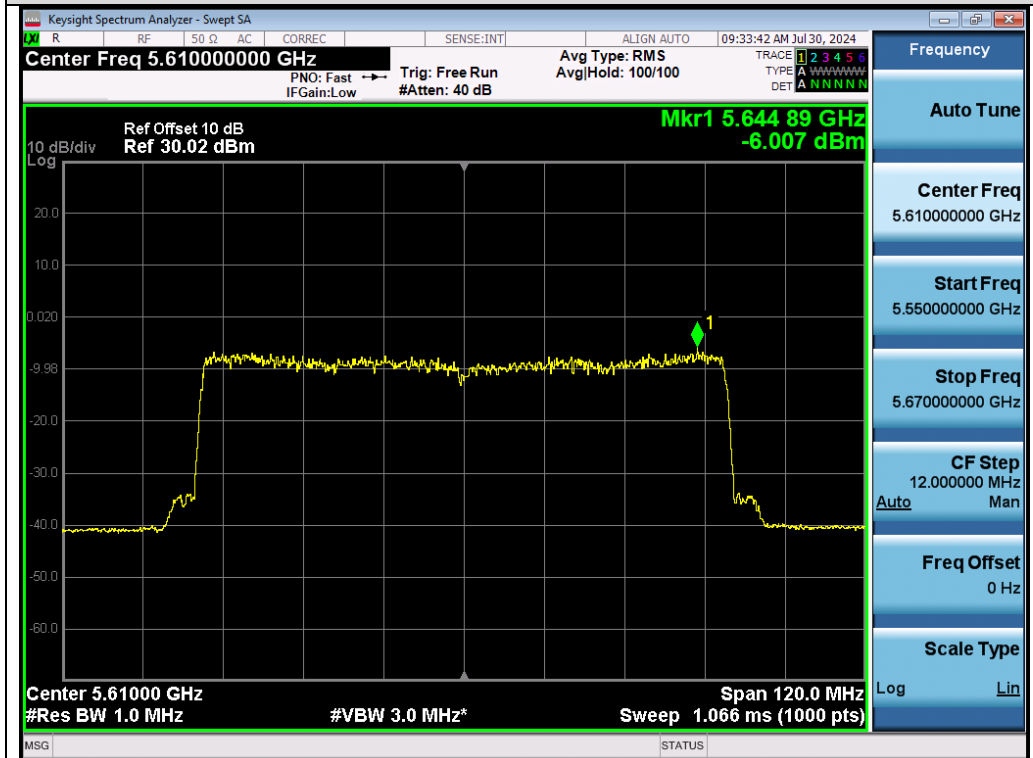
Test_Graph_802.11ax80_Chain B_5610_MCS0_PSD
