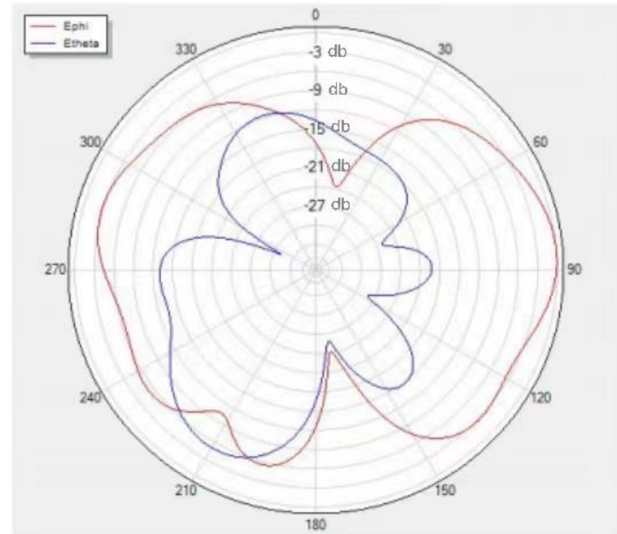
Phi=90 freq=2450MHz
