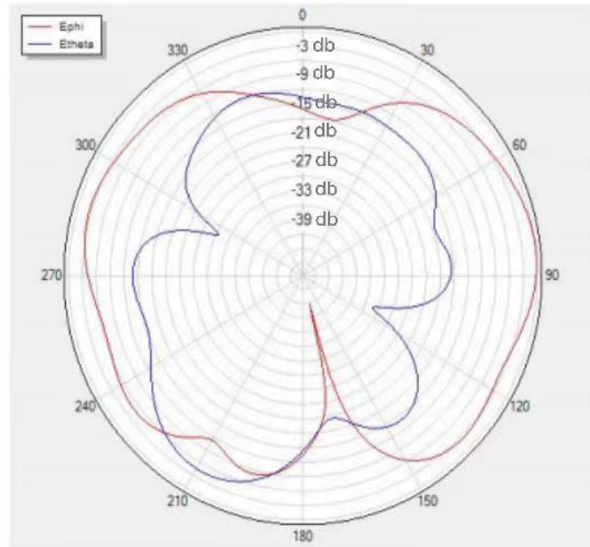
Phi=90 freq=2400MHz
