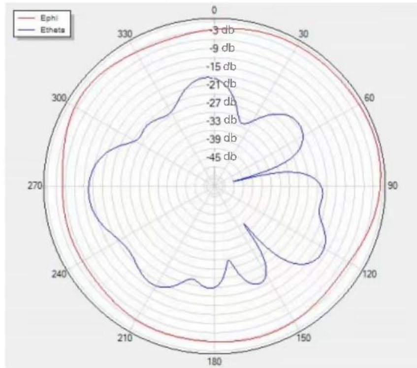
Theta=90 freq=2450MHz
