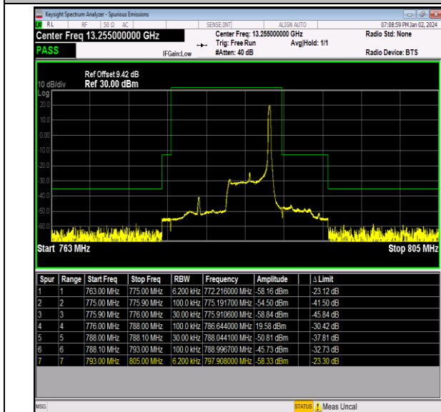
Band13_5MHz_16QAM_23255_1RB#24
