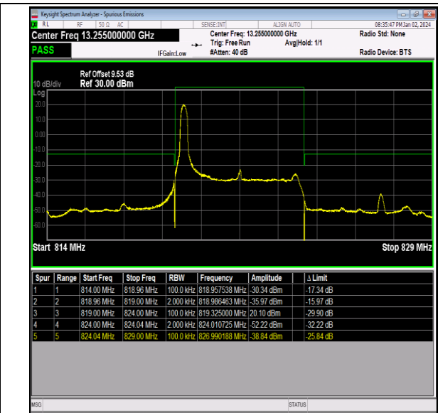
Band26_5MHz_QPSK_26765_1RB#0
