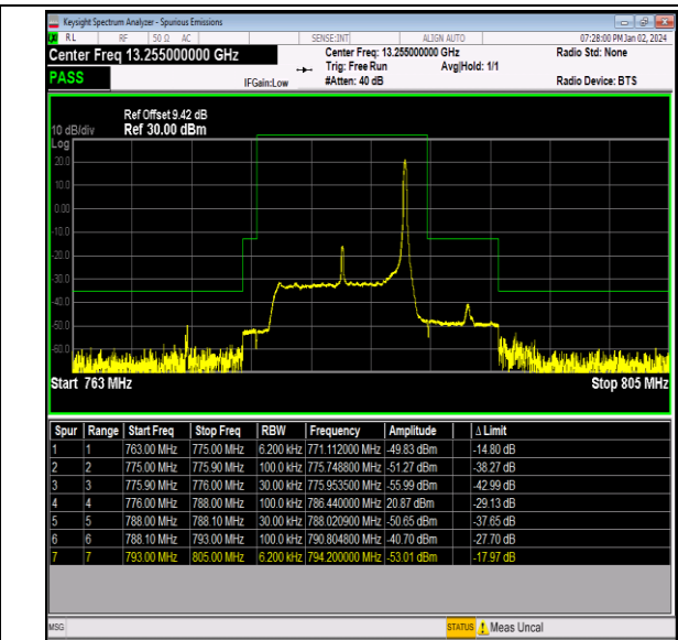
Band13_10MHz_QPSK_23230_1RB#49
