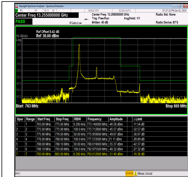
Band13_10MHz_QPSK_23230_1RB#0
