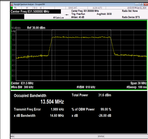
26(824-849)-15MHz-16QAM-26865-75RB#0-PASS
