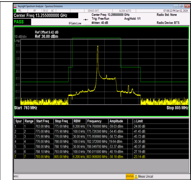
Band13_5MHz_16QAM_23255_1RB#0
