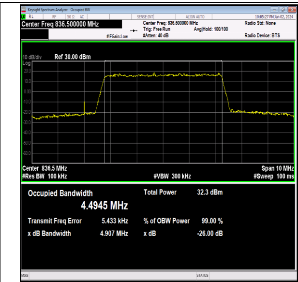
26(824-849)-5MHz-QPSK-26915-25RB#0-PASS
