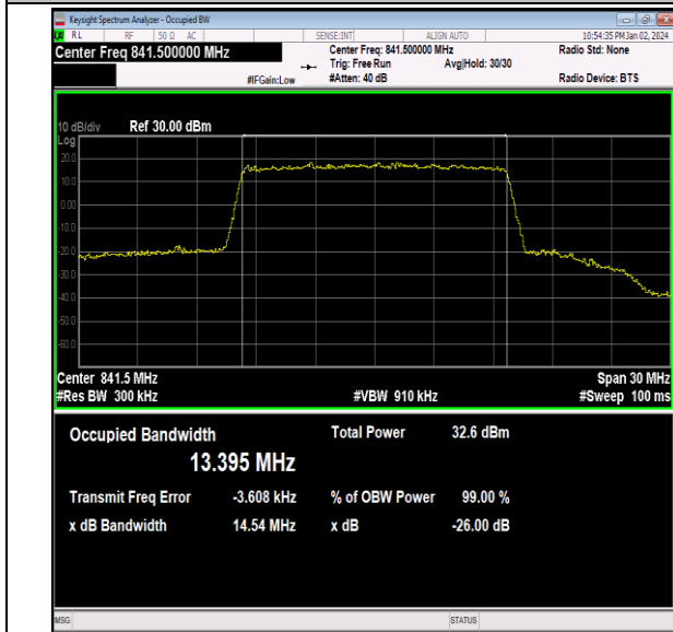
26(824-849)-15MHz-QPSK-26965-75RB#0-PASS
