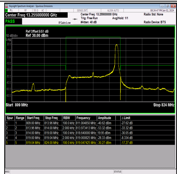
Band26_5MHz_QPSK_26715_1RB#24
