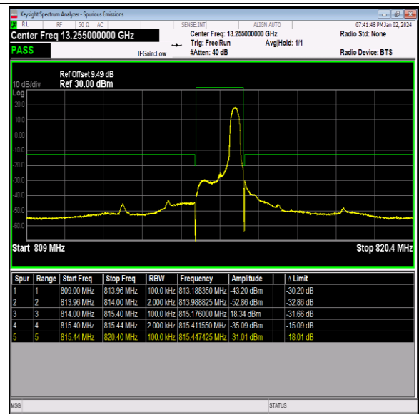
Band26_1.4MHz_16QAM_26697_1RB#5
