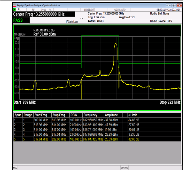
Band26_3MHz_QPSK_26705_1RB#14
