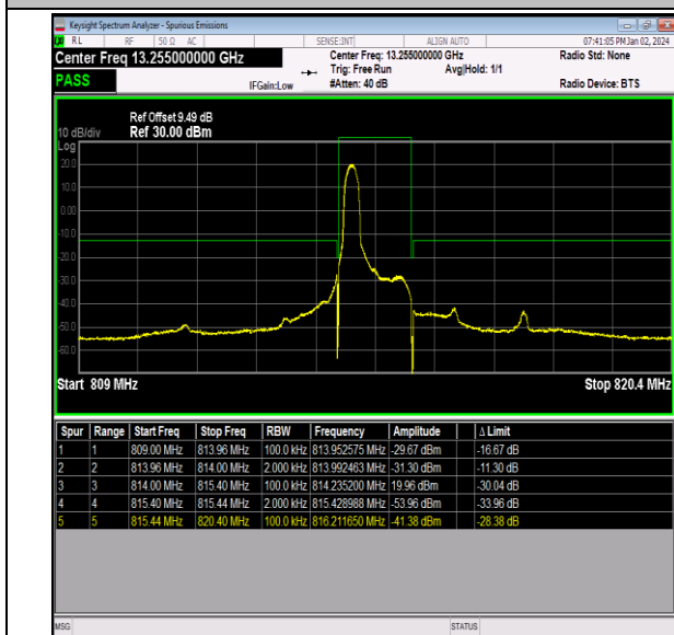
Band26_1.4MHz_QPSK_26697_1RB#0
