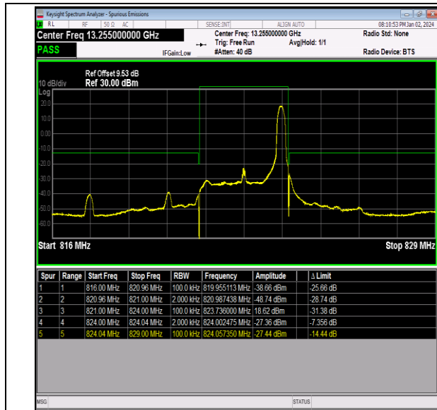
Band26_3MHz_16QAM_26775_1RB#14
