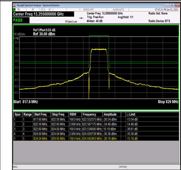
Band26_1.4MHz_QPSK_26783_6RB#0
