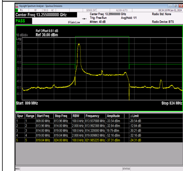
Band26_5MHz_QPSK_26715_1RB#0
