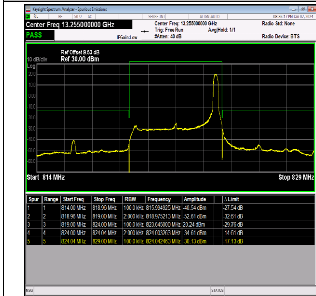
Band26_5MHz_QPSK_26765_1RB#24
