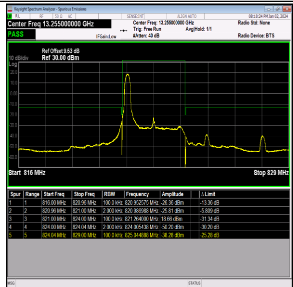
Band26_3MHz_16QAM_26775_1RB#0
