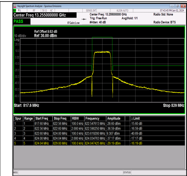
Band26_1.4MHz_16QAM_26783_6RB#0
