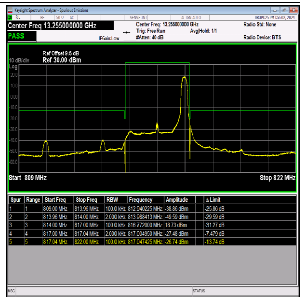
Band26_3MHz_16QAM_26705_1RB#14
