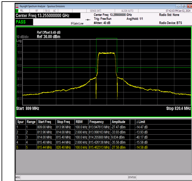
Band26_1.4MHz_QPSK_26697_6RB#0
