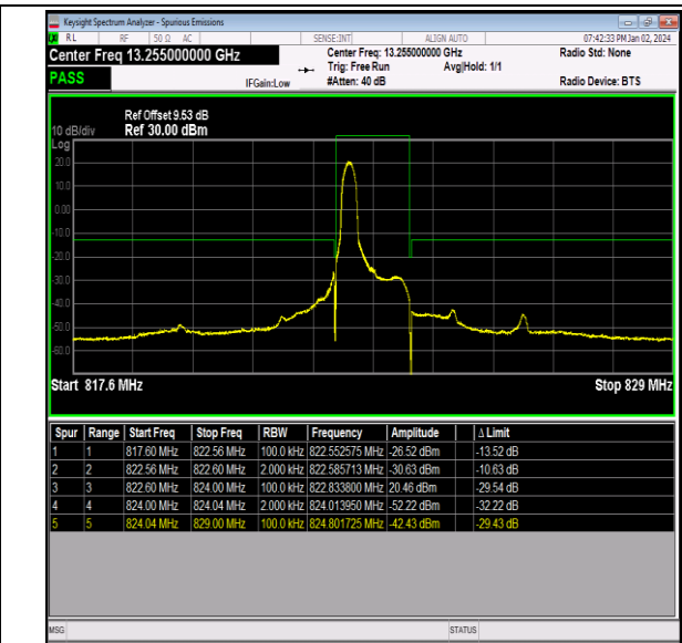
Band26_1.4MHz_QPSK_26783_1RB#0
