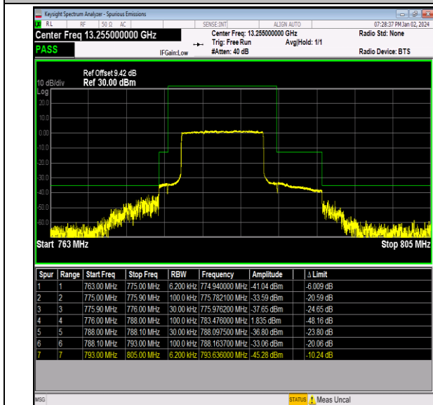
Band13_10MHz_QPSK_23230_50RB#0
