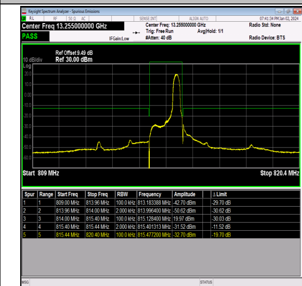
Band26_1.4MHz_QPSK_26697_1RB#5
