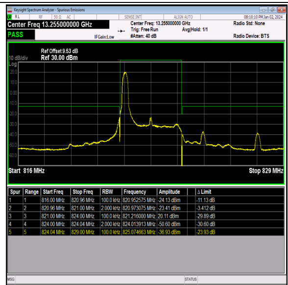
Band26_3MHz_QPSK_26775_1RB#0
