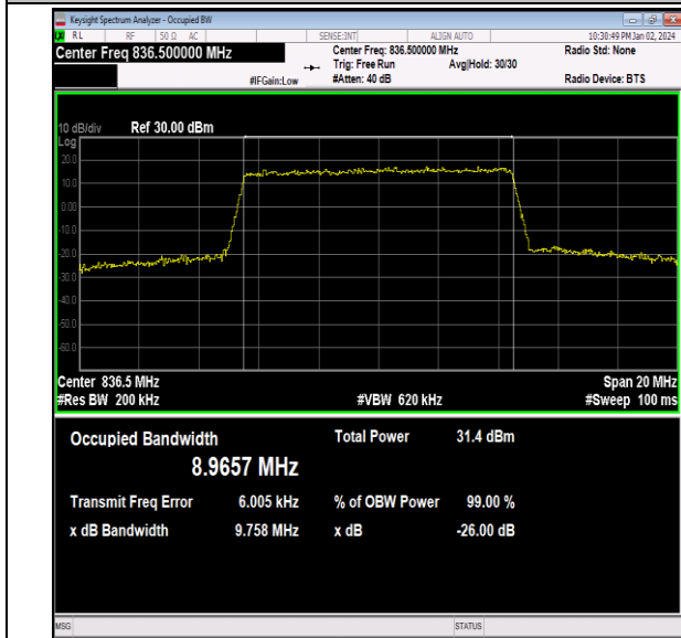
26(824-849)-10MHz-16QAM-26915-50RB#0-PASS
