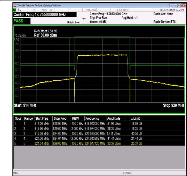
Band26_5MHz_QPSK_26765_25RB#0
