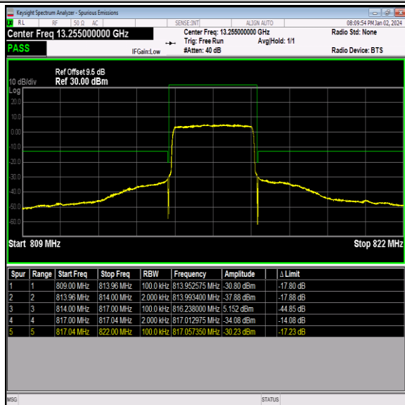
Band26_3MHz_16QAM_26705_15RB#0
