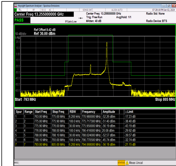
Band13_10MHz_16QAM_23230_1RB#49
