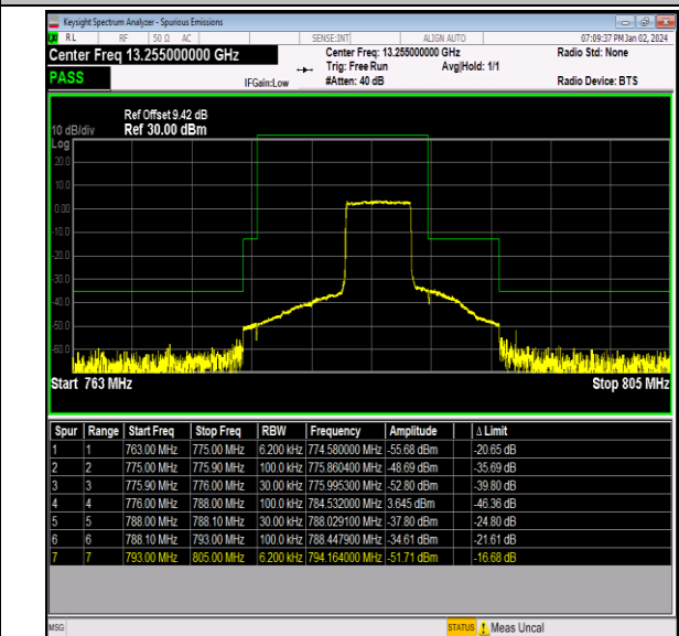
Band13_5MHz_16QAM_23255_25RB#0
