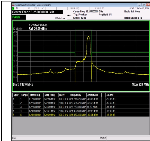
Band26_1.4MHz_16QAM_26783_1RB#5
