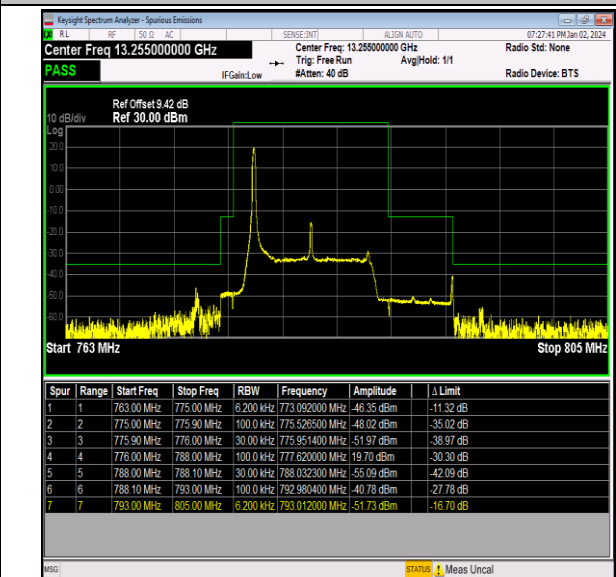
Band13_10MHz_16QAM_23230_1RB#0
