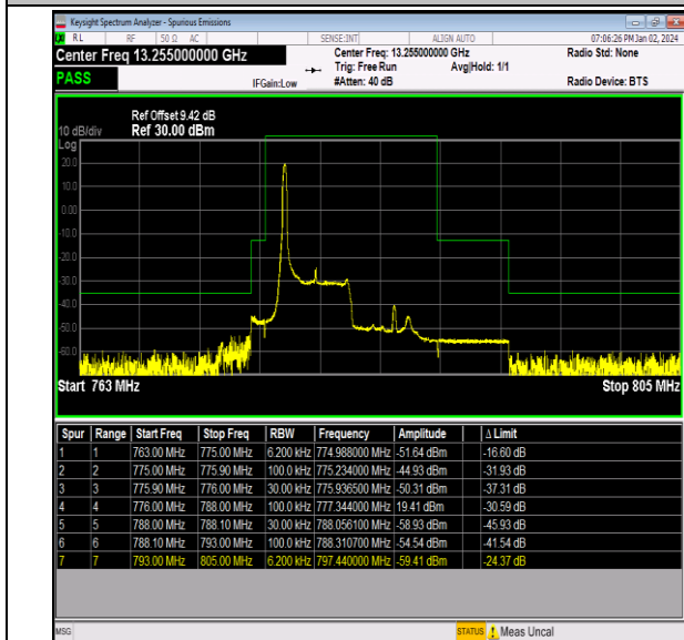
Band13_5MHz_16QAM_23205_1RB#0
