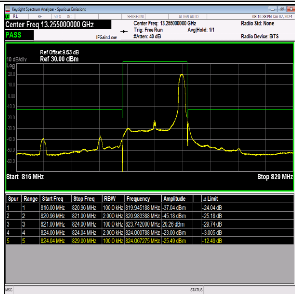
Band26_3MHz_QPSK_26775_1RB#14
