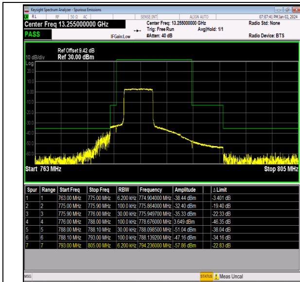
Band13_5MHz_16QAM_23205_25RB#0
