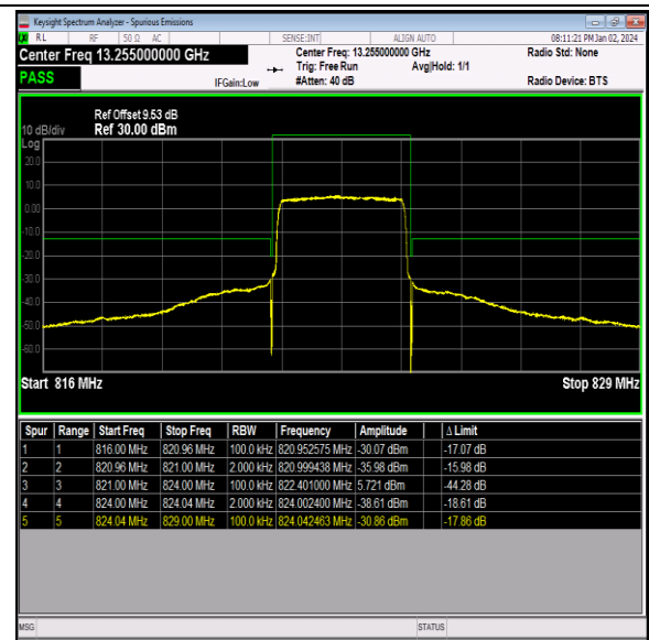
Band26_3MHz_16QAM_26775_15RB#0
