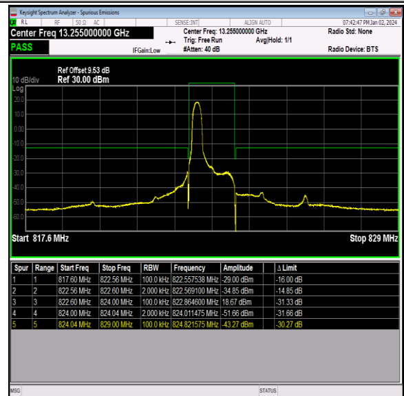
Band26_1.4MHz_16QAM_26783_1RB#0
