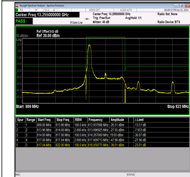
Band26_3MHz_QPSK_26705_1RB#0
