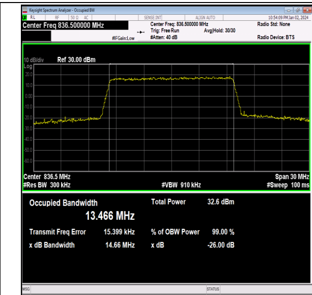
26(824-849)-15MHz-QPSK-26915-75RB#0-PASS
