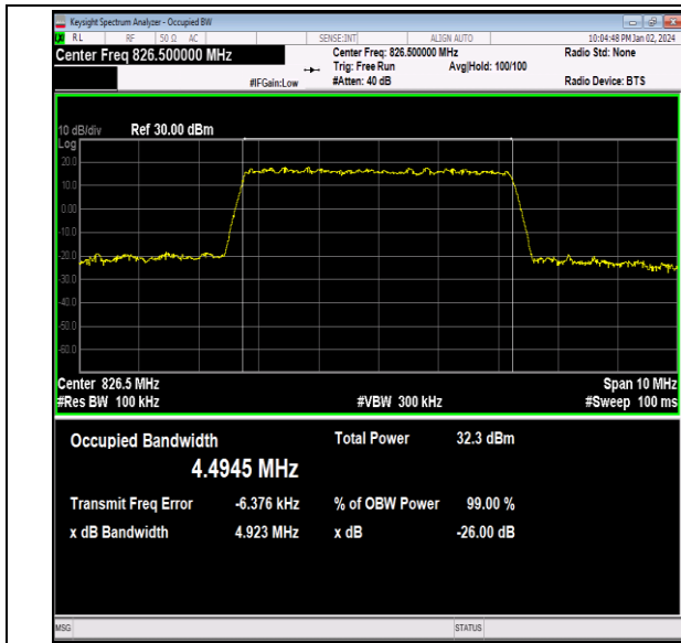
26(824-849)-5MHz-QPSK-26815-25RB#0-PASS
