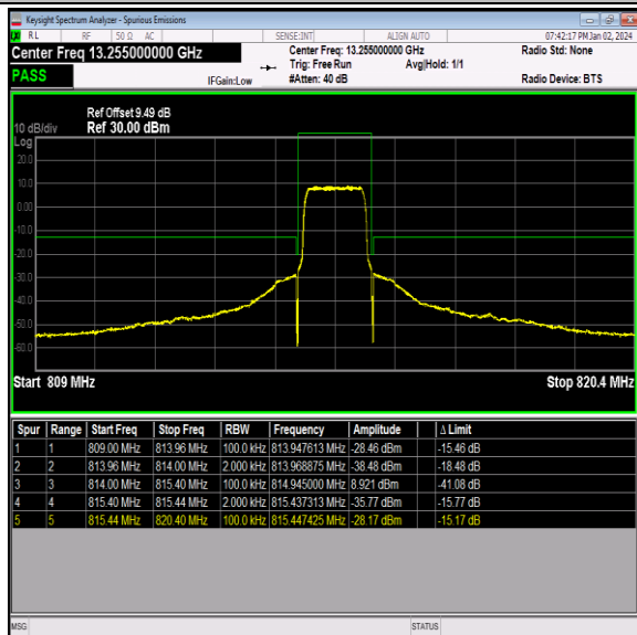
Band26_1.4MHz_16QAM_26697_6RB#0
