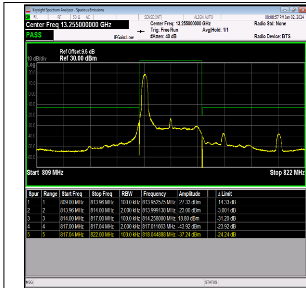
Band26_3MHz_16QAM_26705_1RB#0
