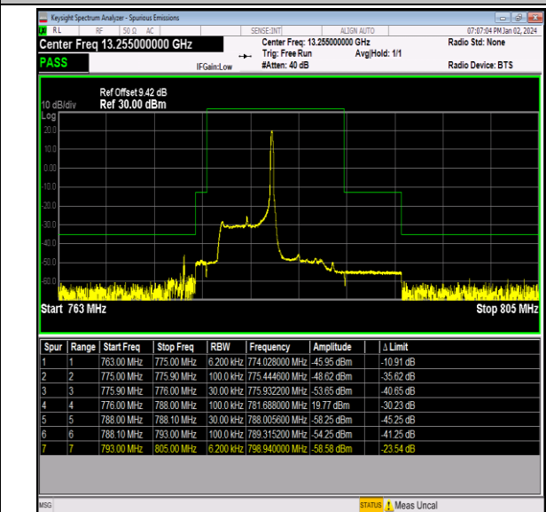
Band13_5MHz_16QAM_23205_1RB#24
