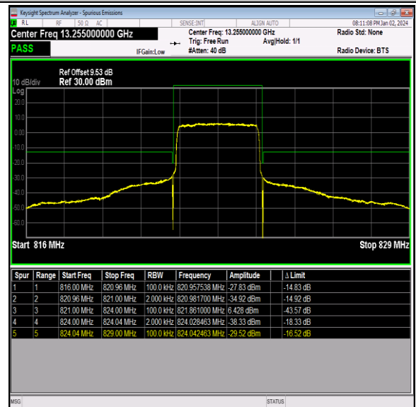
Band26_3MHz_QPSK_26775_15RB#0
