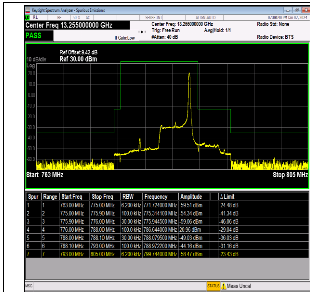
Band13_5MHz_QPSK_23255_1RB#24
