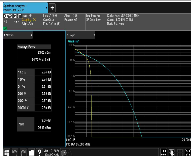
Band13-10MHz-QPSK-23230-50RB#0
