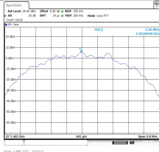
BLE_2M-Ant1-2402-0~Reference-PASS
