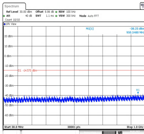
BLE_1M-Ant1-2402-30~1000-PASS
