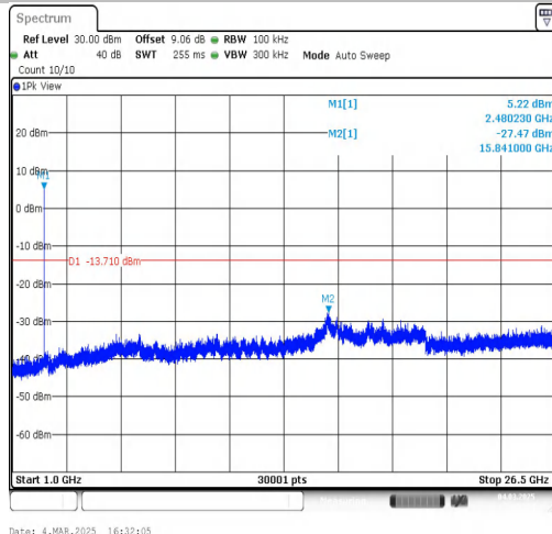
BLE_1M-Ant1-2480-1000~26500-PASS
