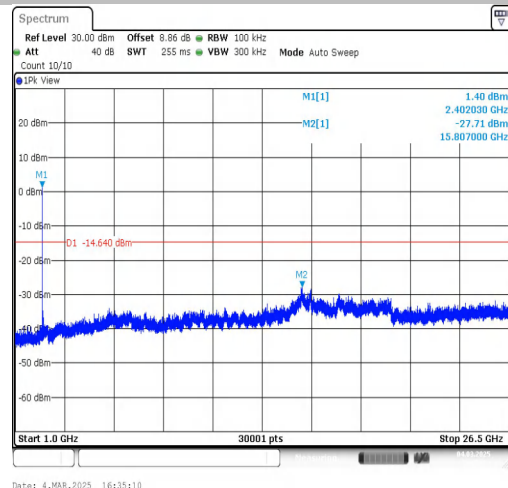
BLE_2M-Ant1-2402-1000~26500-PASS
