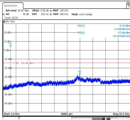
BLE_1M-Ant1-2440-0~Reference-PASS
