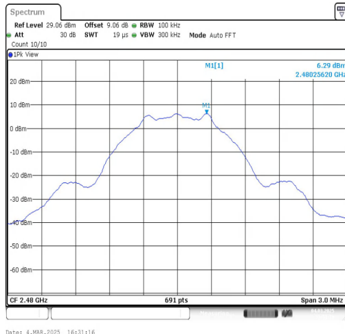
BLE_1M-Ant1-2480-0~Reference-PASS
