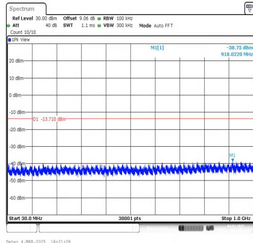
BLE_1M-Ant1-2480-30~1000-PASS
