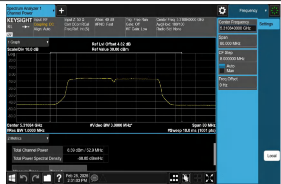
11N40MIMO-Ant2-5310-TPC_H-PASS
