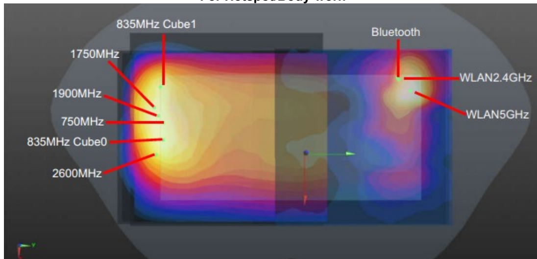
WWAN + WLAN 5GHz/2.4GHz + Bluetooth Back_5mm
