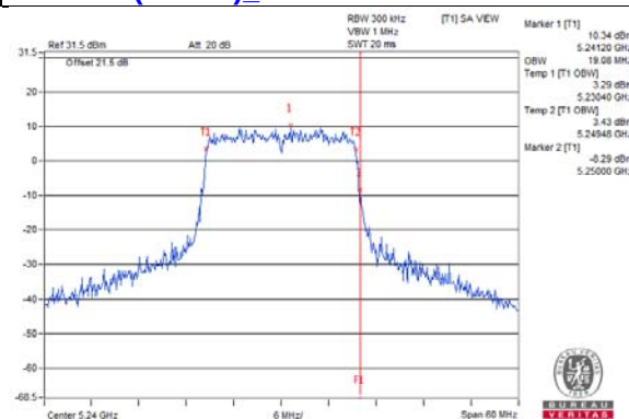
802.11ax (VHT20)_Chain 7 / CH48
