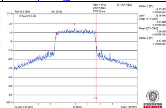
802.11ax (VHT40) Chain 7 / CH46
