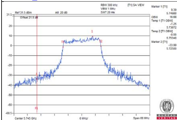
802.11a_Chain 4 / CH149
