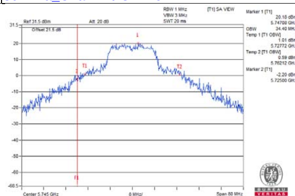
802.11ax (VHT20)_Chain 5 / CH149
