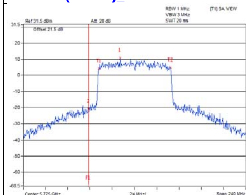
802.11ax (VHT80) Chain 6 / CH155
