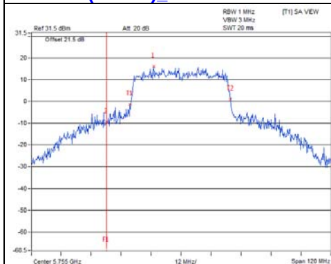
802.11ax (VHT40) Chain 6 / CH151
