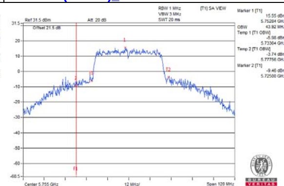
802.11ax (VHT40) Chain 7 / CH151
