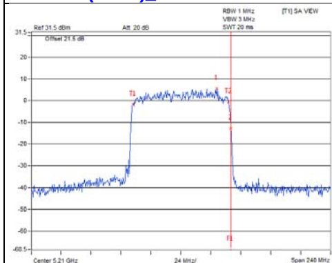
802.11ax (HE80) Chain 6 / CH42
