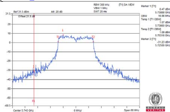
802.11a_Chain 5 / CH149
