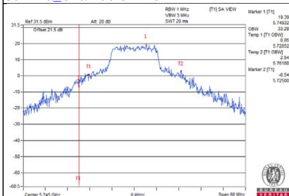
802.11ax (VHT20)_Chain0 / CH149
