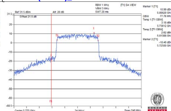
802.11ax (VHT80) Chain 7 / CH155
