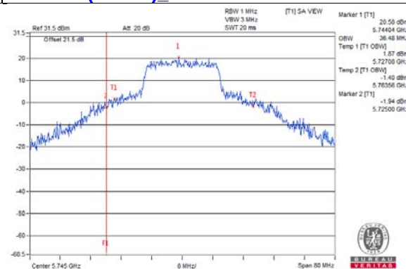
802.11ax (VHT20)_Chain 7 / CH149
