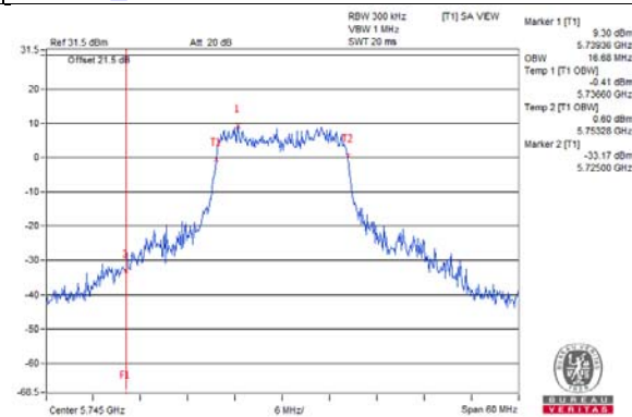
802.11a_Chain 7 / CH149
