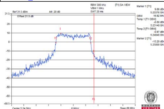
802.11ax (VHT20)_Chain 5 / CH48
