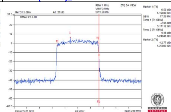
802.11ax (VHT80) Chain 7 / CH42
