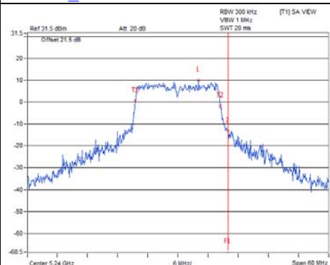
802.11ax (VHT20)_Chain 4 / CH48
