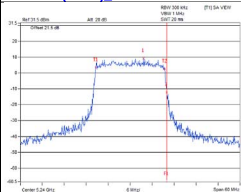
802.11ax (HE20) Chain 4 / CH48
