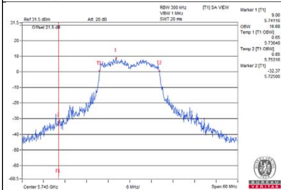
802.11a_Chain 6 / CH149
