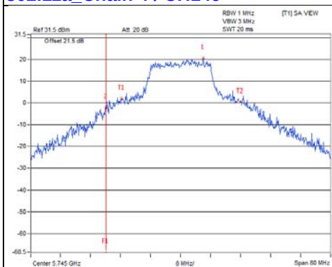
802.11a_Chain 6 / CH149
