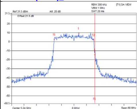
802.11ax (HE20) Chain 6 / CH48
