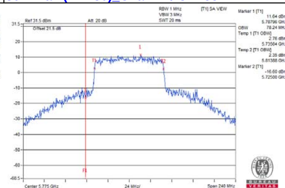
802.11ax (VHT80) Chain 7 / CH155
