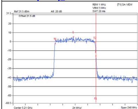
802.11ax (HE80) Chain 2 / CH42
