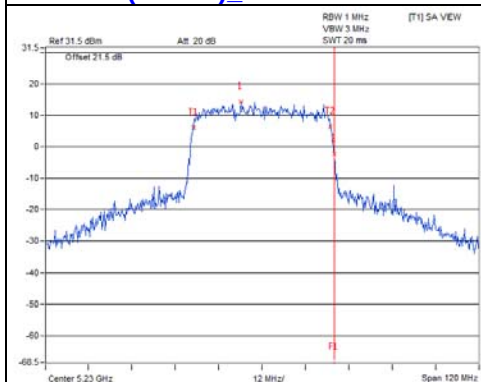
802.11ax (VHT40) Chain 6 / CH46
