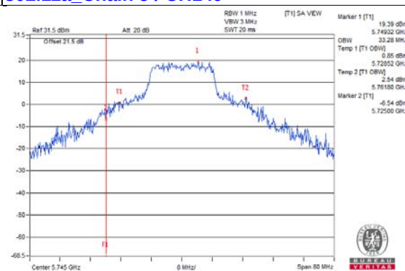
802.11a_Chain 7 / CH149
