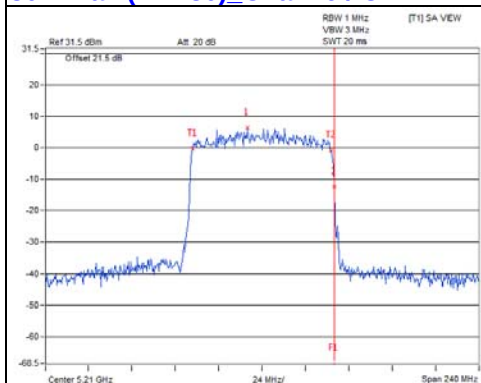
802.11ax (VHT80) Chain 6 / CH42
