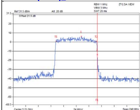
802.11ax (HE80) Chain 4 / CH42
