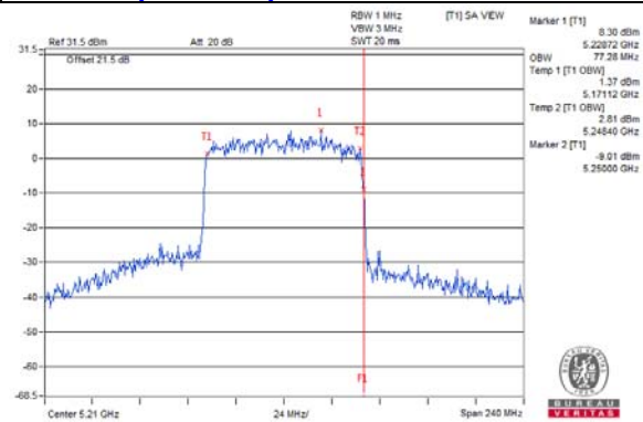
802.11ax (HE80+80) / Chain 3 : CH42
