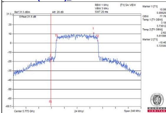
802.11ax (VHT80)_Chain0 / CH155
