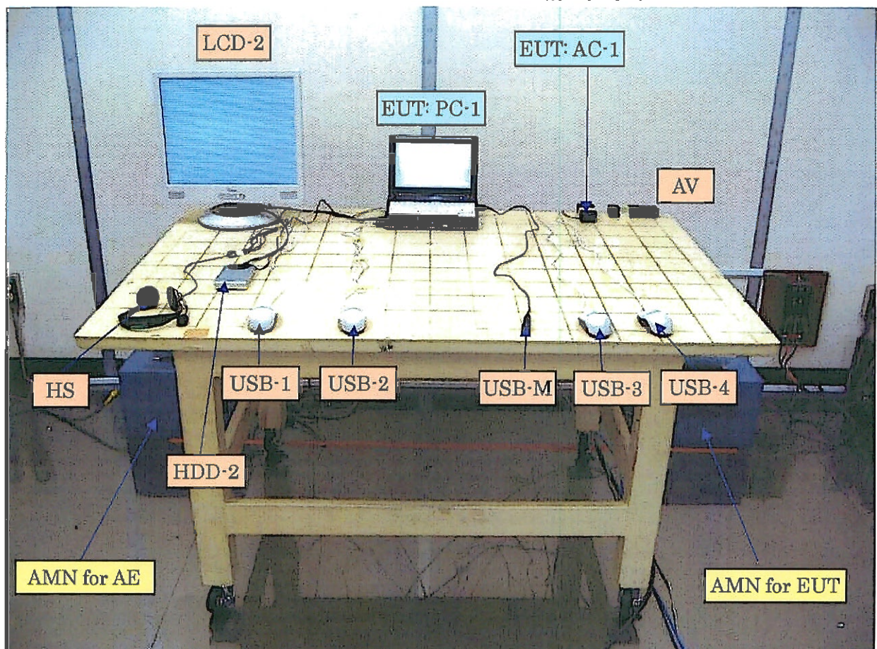
Photo-2 Conducted emission measurement
