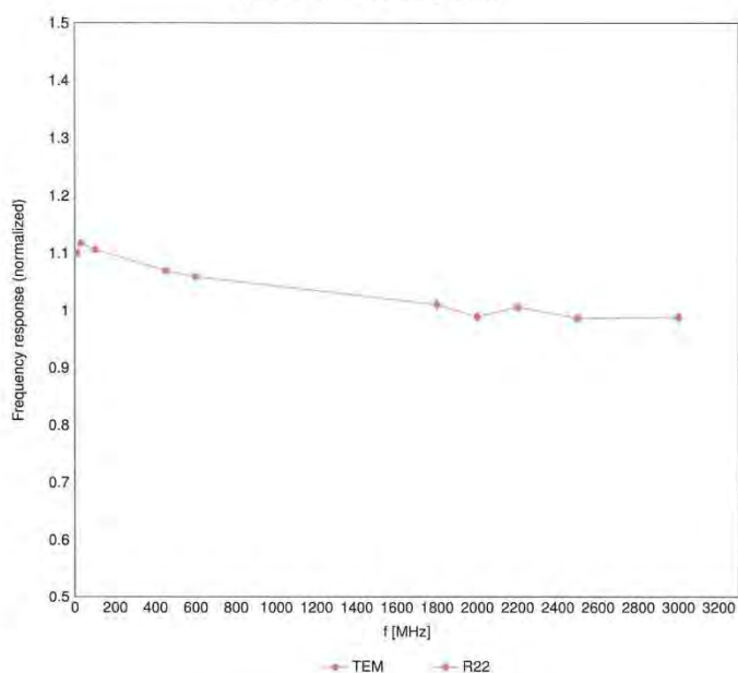
Frequency Response of E-Field (TEM-Cell:ifi110 EXX, Waveguide:R22)
