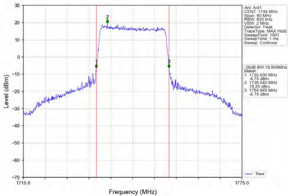
Band66_20MHz_16QAM_MCH_1745MHz_RB_100_0_NTN
