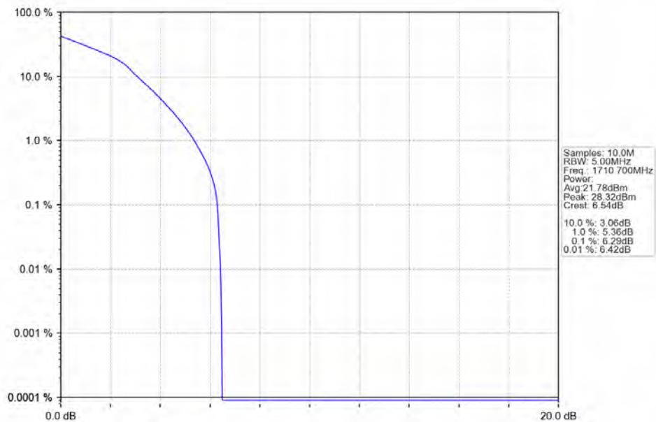
Band66_1.4MHz_16QAM_LCH_1710.7MHz_RB_6_0_NTN
