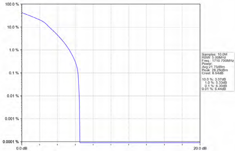
Band66 1.4MHz 64QAM LCH 1710.7MHz RB 6 0 NTN
