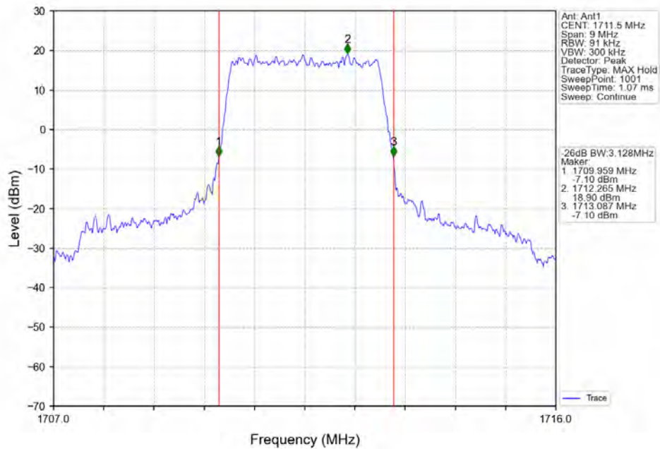
Band66_3MHz_QPSK_LCH_1711.5MHz_RB_15_0 NTN
