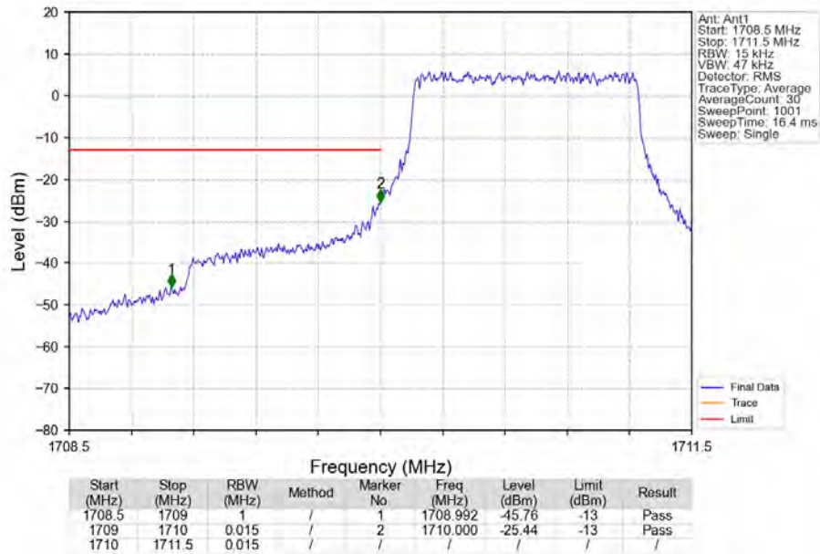
Band66_1.4MHz_QPSK_LCH_1710.7MHz_RB_6_0_NTNV
