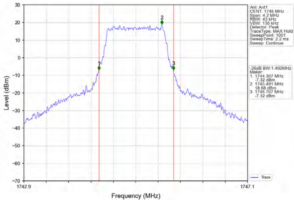
Band66_1.4MHz_64QAM_MCH_1745MHz_RB_6_0_NTN
