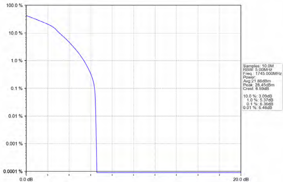
Band66_1.4MHz_64QAM_MCH_1745MHz_RB_6_0 NTN
