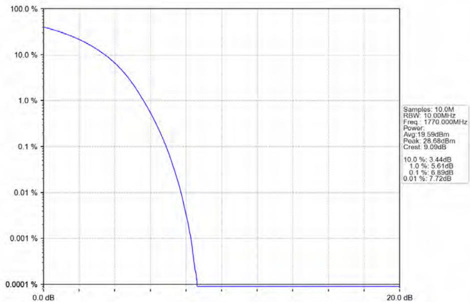
Band66_20MHz_16QAM_HCH_1770MHz_RB_100_0 NTN
