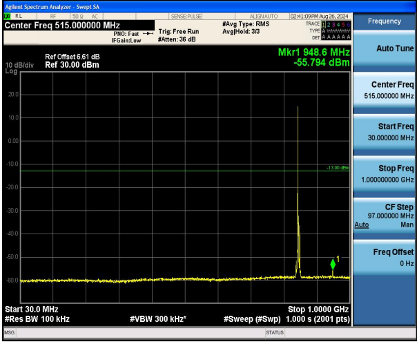
Band5_3MHz_QPSK_20635_1RB#0_30~1000_30~1000
