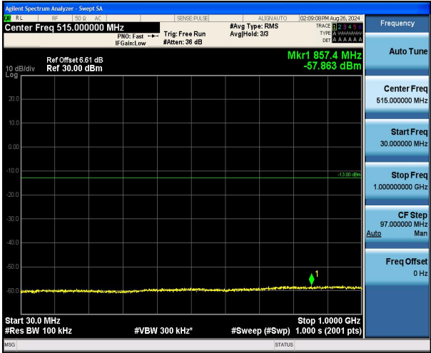
Band4_20MHz_QPSK_20300_1RB#0_30~1000_30~1000
