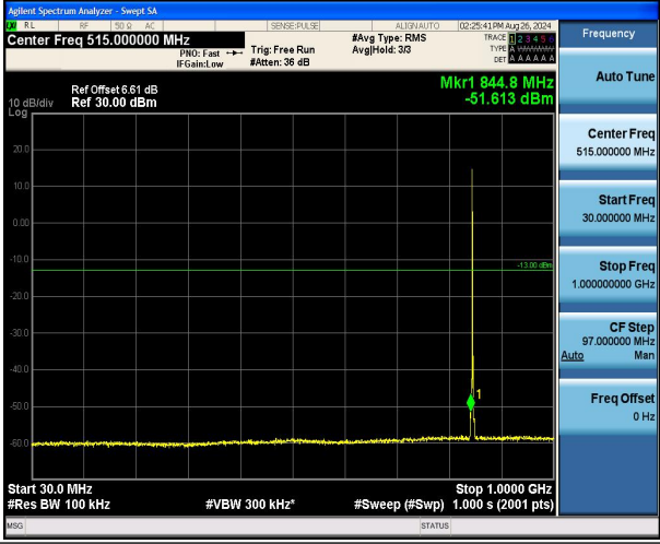
Band5_1.4MHz_QPSK_20643_1RB#0_30~1000_30~1000
