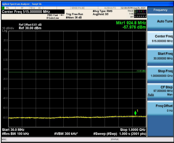
Band4_20MHz_QPSK_20175_1RB#0_30~1000_30~1000
