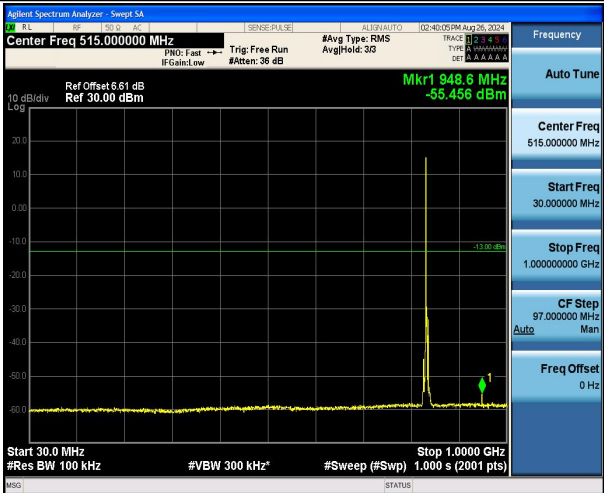
Band5_3MHz_QPSK_20525_1RB#0_30~1000_30~1000
