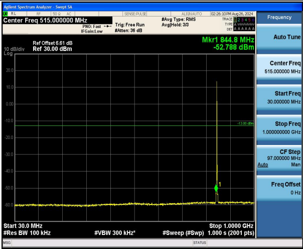
Band5_1.4MHz_16QAM_20643_1RB#0_30~1000_30~1000
