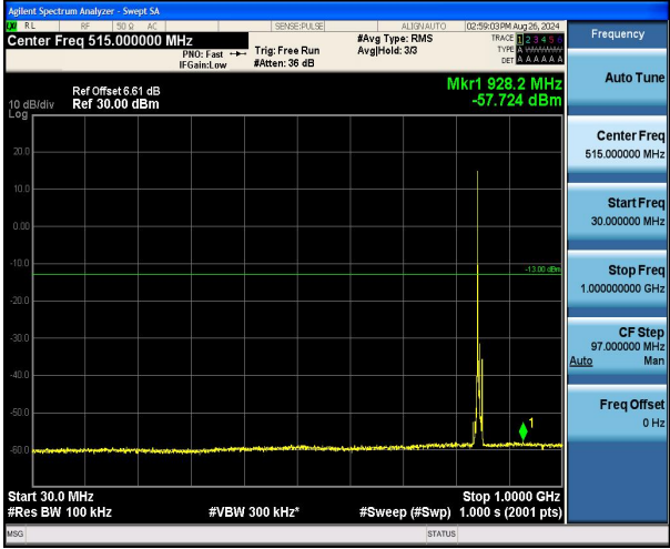
Band5_5MHz_QPSK_20625_1RB#0_30~1000_30~1000
