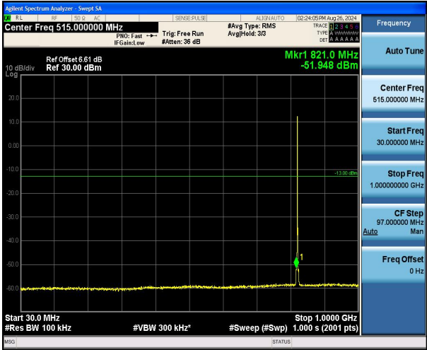
Band5_1.4MHz_16QAM_20407_1RB#0_30~1000_30~1000
