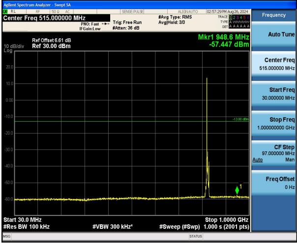
Band5_5MHz_16QAM_20425_1RB#0_30~1000_30~1000
