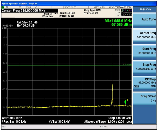
Band5_3MHz_16QAM_20635_1RB#0_30~1000_30~1000
