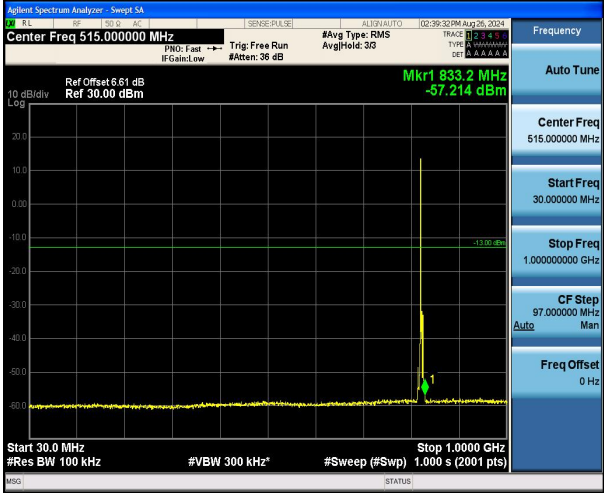
Band5_3MHz_16QAM_20415_1RB#0_30~1000_30~1000
