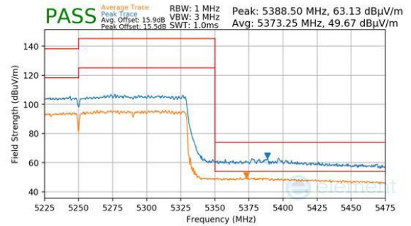
Plot 7-1208. CDD (Peak & Average, Ch.50, 802.11ax(SU), MCS4)
