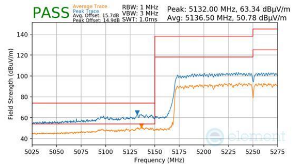
Plot 7-1209. CDD (Peak & Average, Ch.50, 802.11ax(SU), MCS11)
