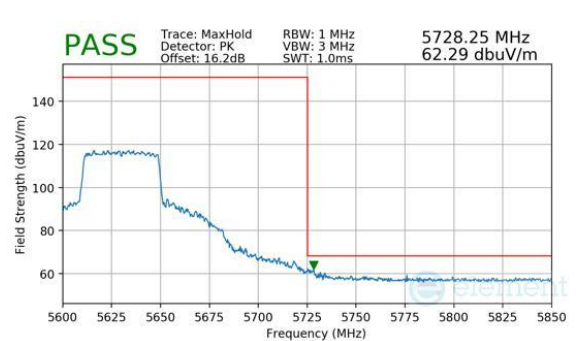
Plot 7-1141. SDM (Peak, Ch.126, 802.11ax(SU), MCS11) (FCC Only)
