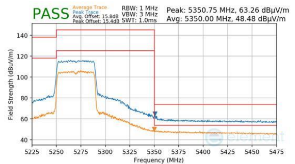
Plot 7-1129. SDM (Peak & Average, Ch.54, 802.11ax(SU), MCS4)
