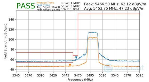
Plot 7-1082. CDD (Peak & Average, Ch.100, 802.11ax(SU), MCS11)
