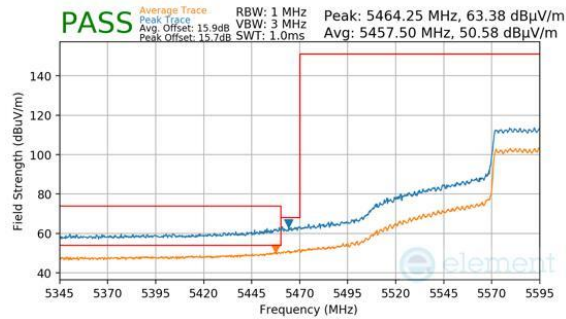
Plot 7-1181. CDD (Peak & Average, Ch.122, 802.11ax(SU), MCS2) (FCC Only)
