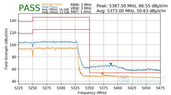
Plot 7-1210. CDD (Peak & Average, Ch.50, 802.11ax(SU), MCS11)
