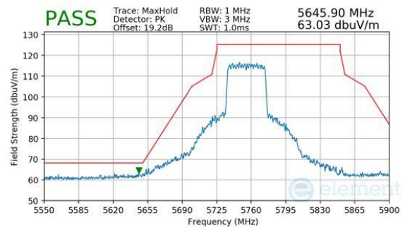
Plot 7-1147. CDD (Peak, Ch.151, 802.11ax(SU), MCS11)
