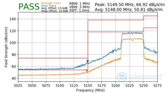
Plot 7-1127. CDD (Peak & Average, Ch.46, 802.11ax(SU), MCS11)
