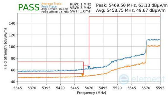
Plot 7-1183. CDD (Peak & Average, Ch.122, 802.11ax(SU), MCS4) (FCC Only)
