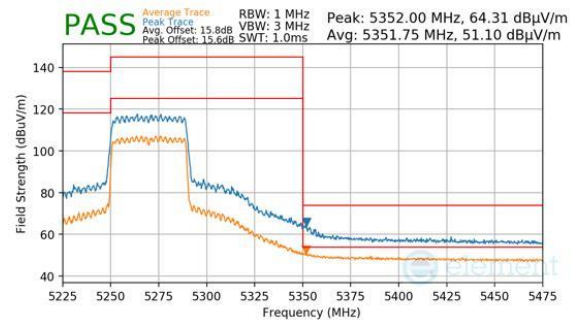
Plot 7-1128. SDM (Peak & Average, Ch.54, 802.11ax(SU), MCS2)
