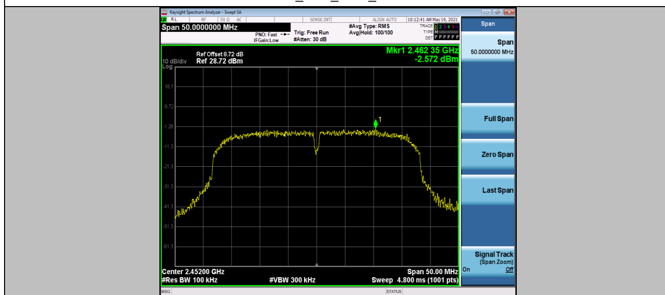
11N40SISO_Ant1_2452_0~Reference
