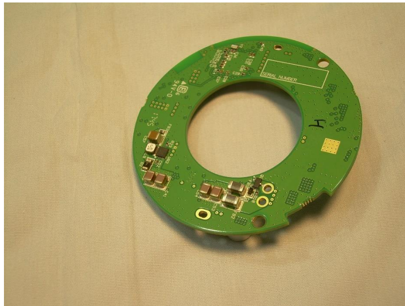
Photograph 14 – Back Side of the PCB
