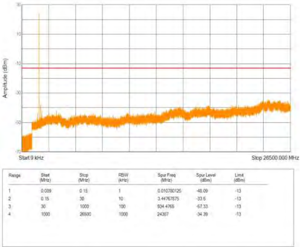
Band66 QPSK BW=10MHz Channel=132322 RB Size=1 Position=#0 NB Index=0
