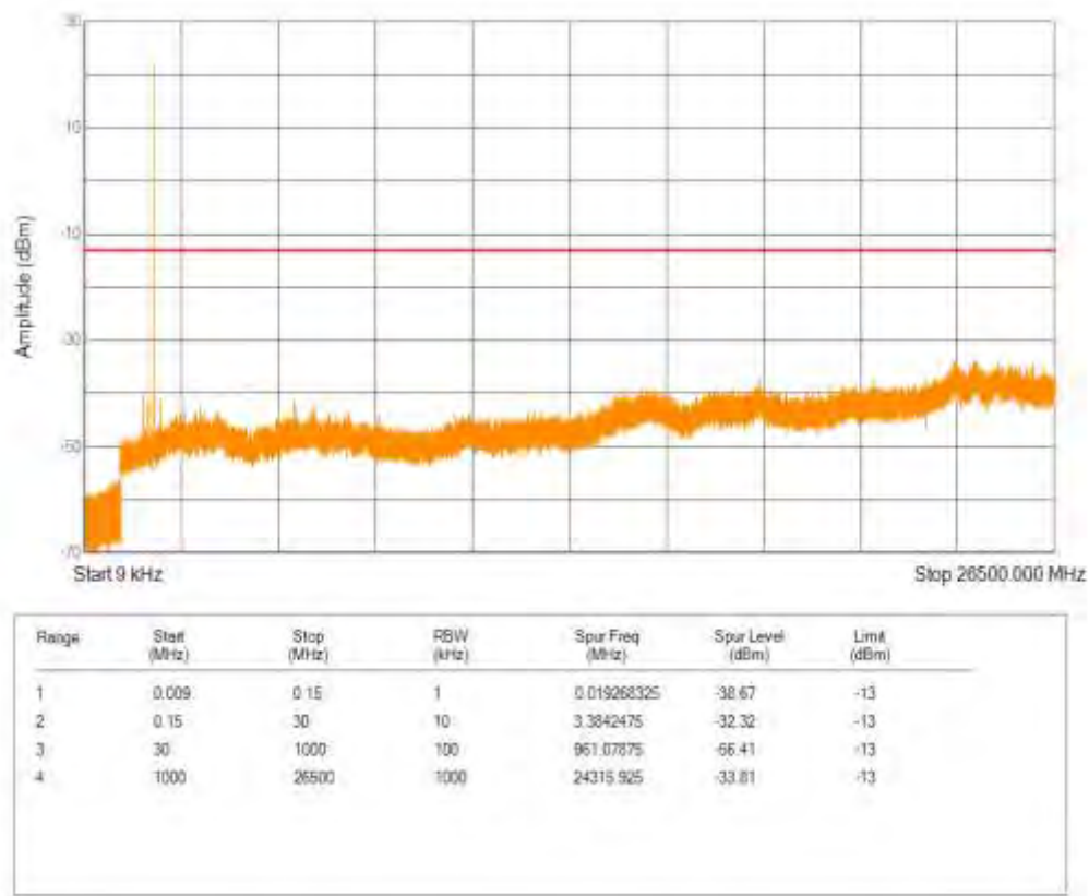
Band25 16QAM BW=1.4MHz Channel=26683 RB Size=1 Position=#0 NB Index=0
