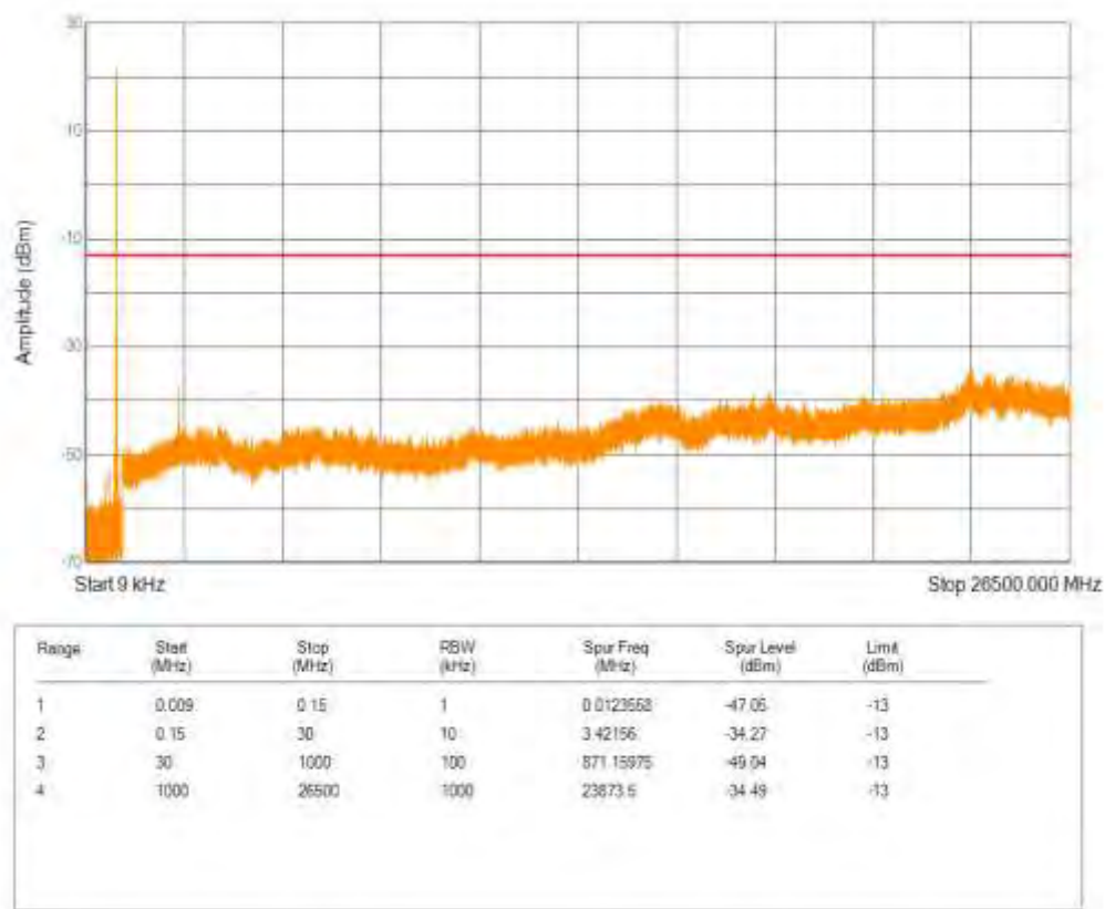
Band26(824-849) 16QAM BW=5MHz Channel=27015 RB Size=5 Position=#0 NB Index=0
