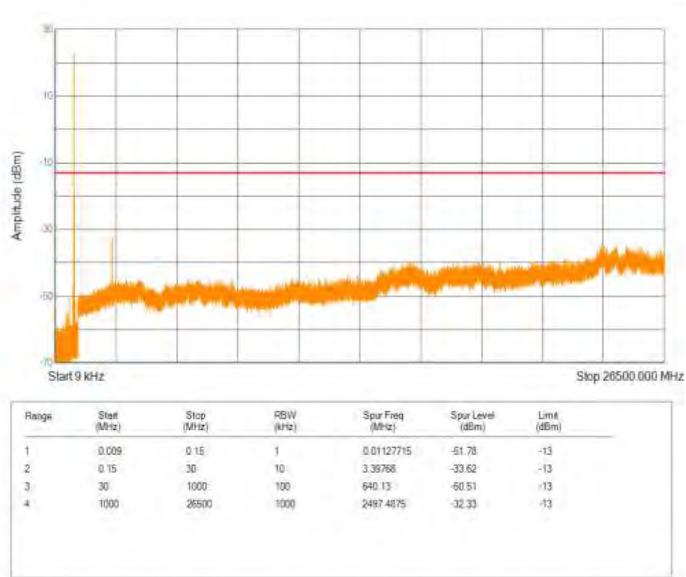
Band5 16QAM BW=10MHz Channel=20525 RB Size=5 Position=#0 NB Index=0
