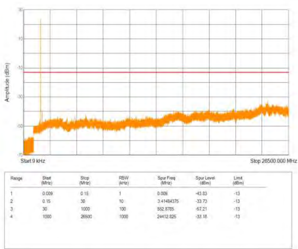
Band66 QPSK BW=5MHz Channel=132322 RB Size=1 Position=#0 NB Index=0
