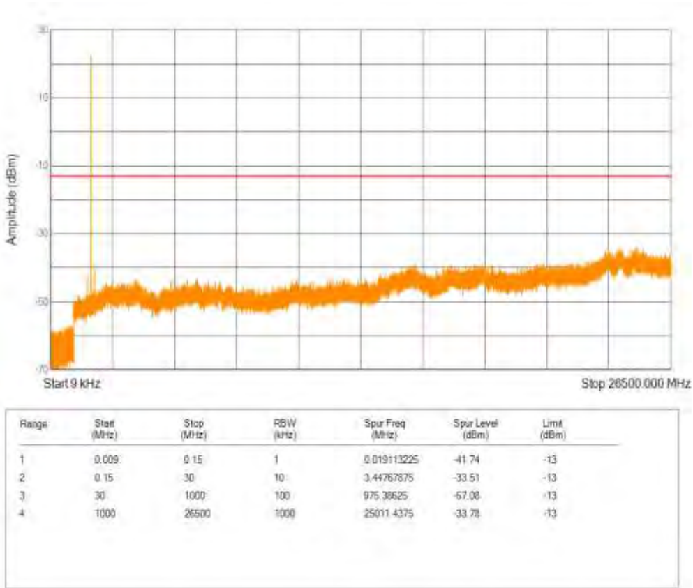
Band66 QPSK BW=10MHz Channel=132322 RB Size=6 Position=#0 NB Index=0
