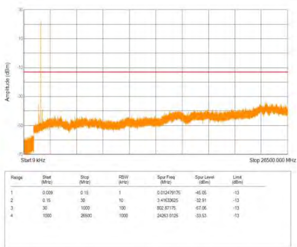
Band66 16QAM BW=10MHz Channel=132022 RB Size=1 Position=#0 NB Index=0
