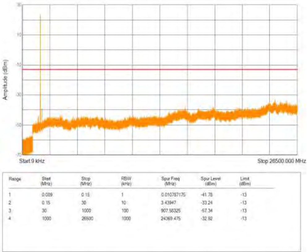
Band66 QPSK BW=3MHz Channel=132657 RB Size=1 Position=#0 NB Index=0
