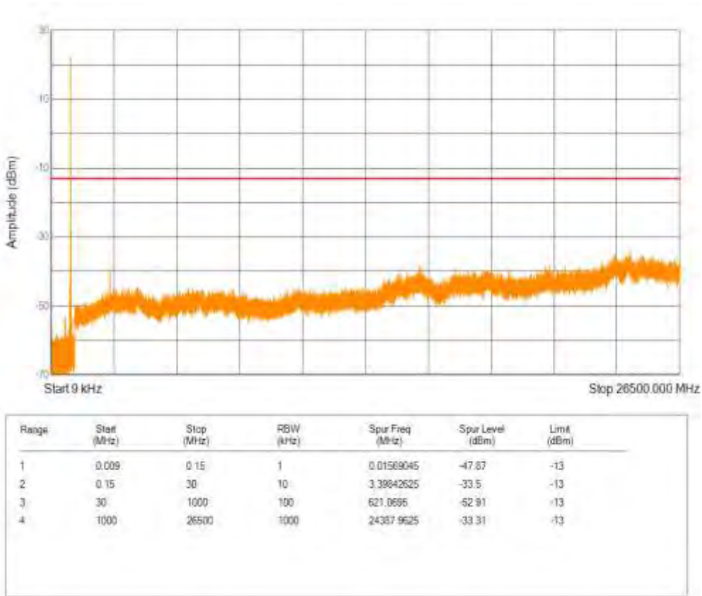
Band26(824-849) 16QAM BW=10MHz Channel=26915 RB Size=5 Position=#0 NB Index=0
