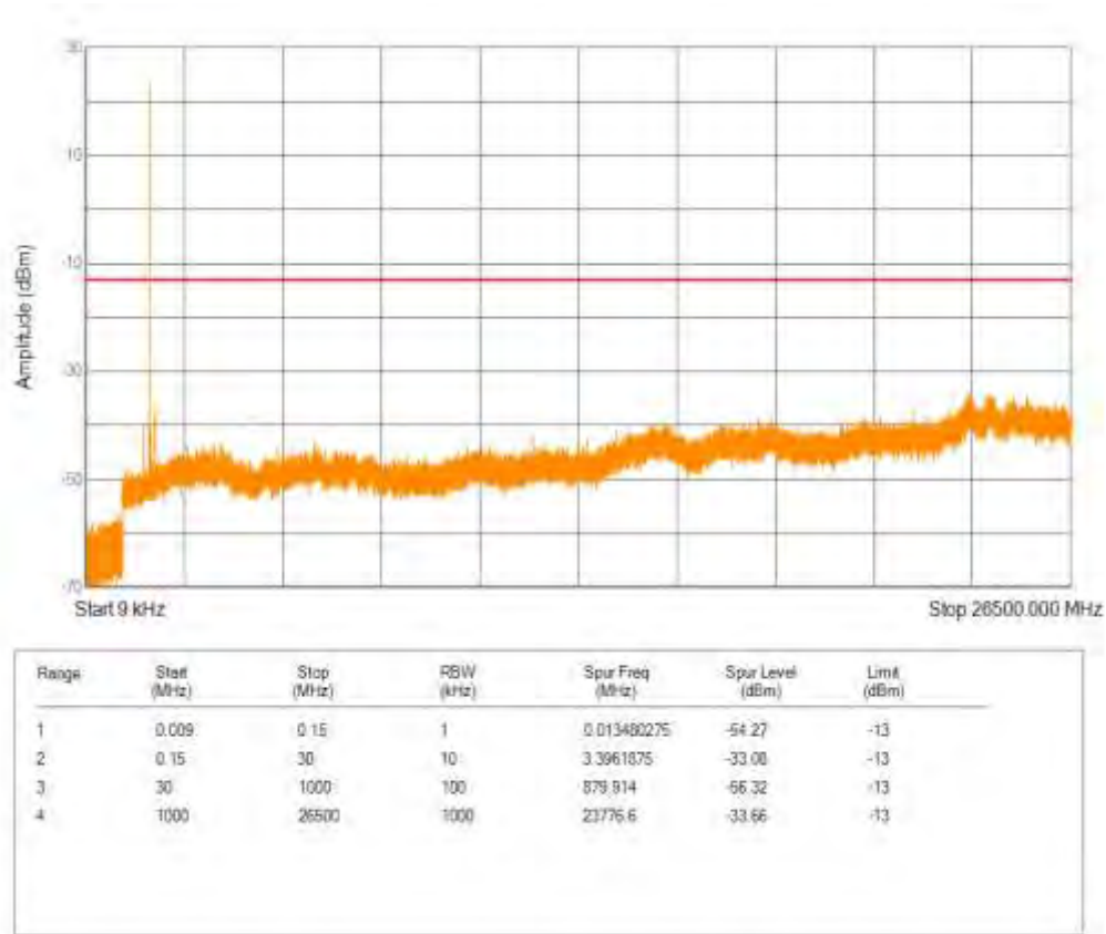
Band4 QPSK BW=20MHz Channel=20175 RB Size=6 Position=#0 NB Index=0
