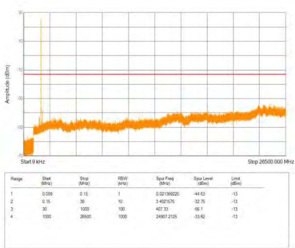
Band66 16QAM BW=10MHz Channel=132622 RB Size=5 Position=#0 NB Index=0
