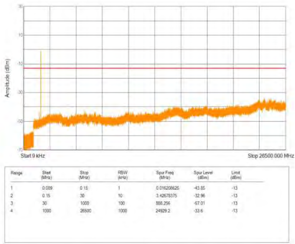
Band66 16QAM BW=1.4MHz Channel=132322 RB Size=1 Position=#0 NB Index=0
