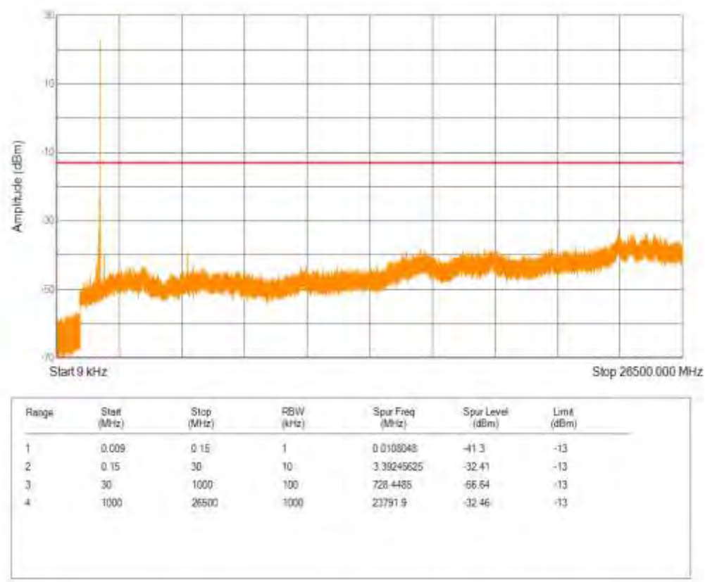
Band25 QPSK BW=15MHz Channel=26365 RB Size=1 Position=#0 NB Index=0
