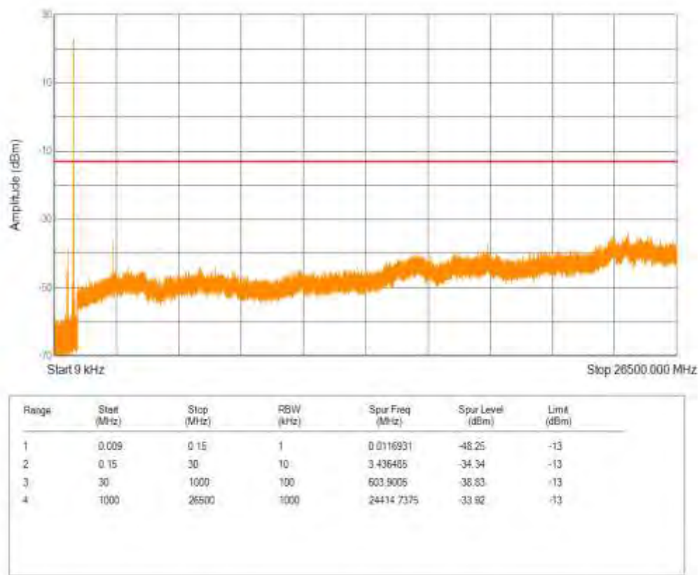
Band26(824-849) QPSK BW=5MHz Channel=26915 RB Size=6 Position=#0 NB Index=0
