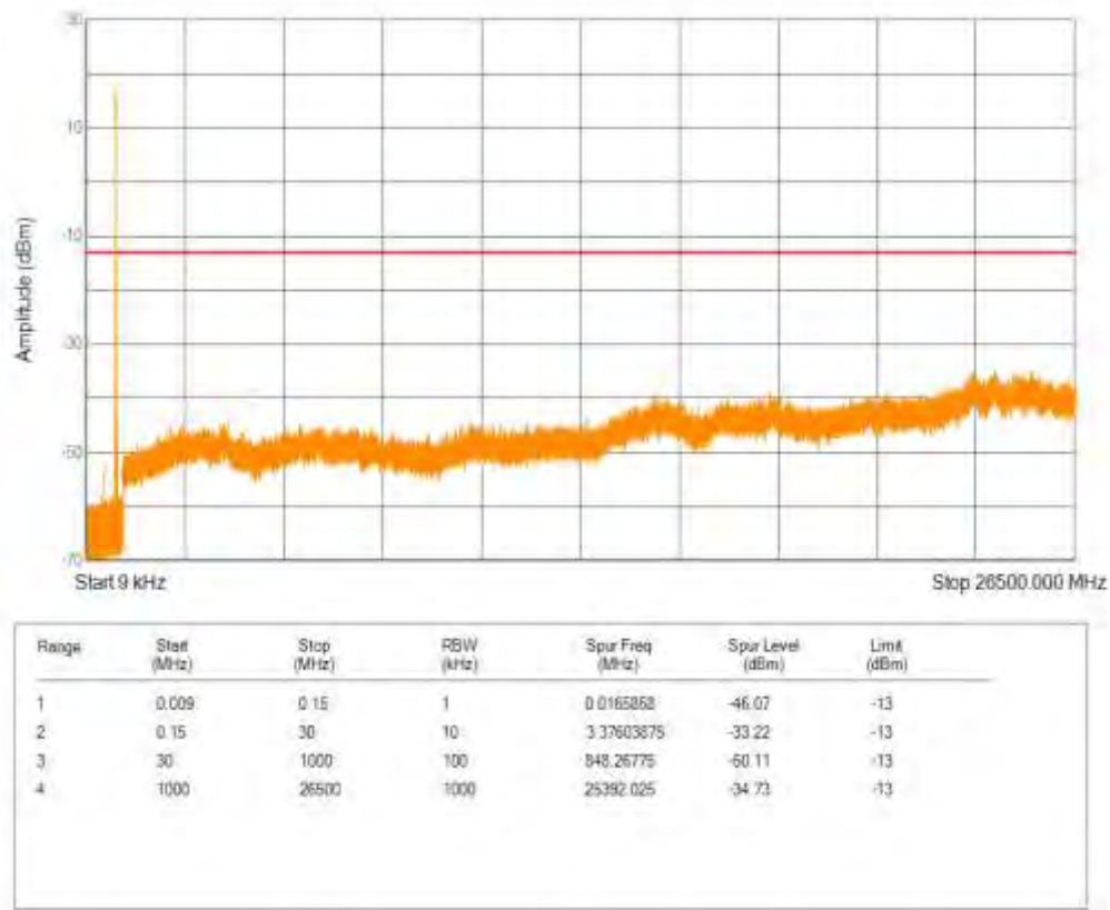
Band26(814-824) QPSK BW=3MHz Channel=26775 RB Size=1 Position=#0 NB Index=0
