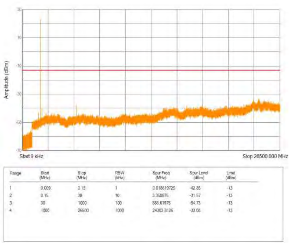
Band25 16QAM BW=15MHz Channel=26115 RB Size=1 Position=#0 NB Index=0
