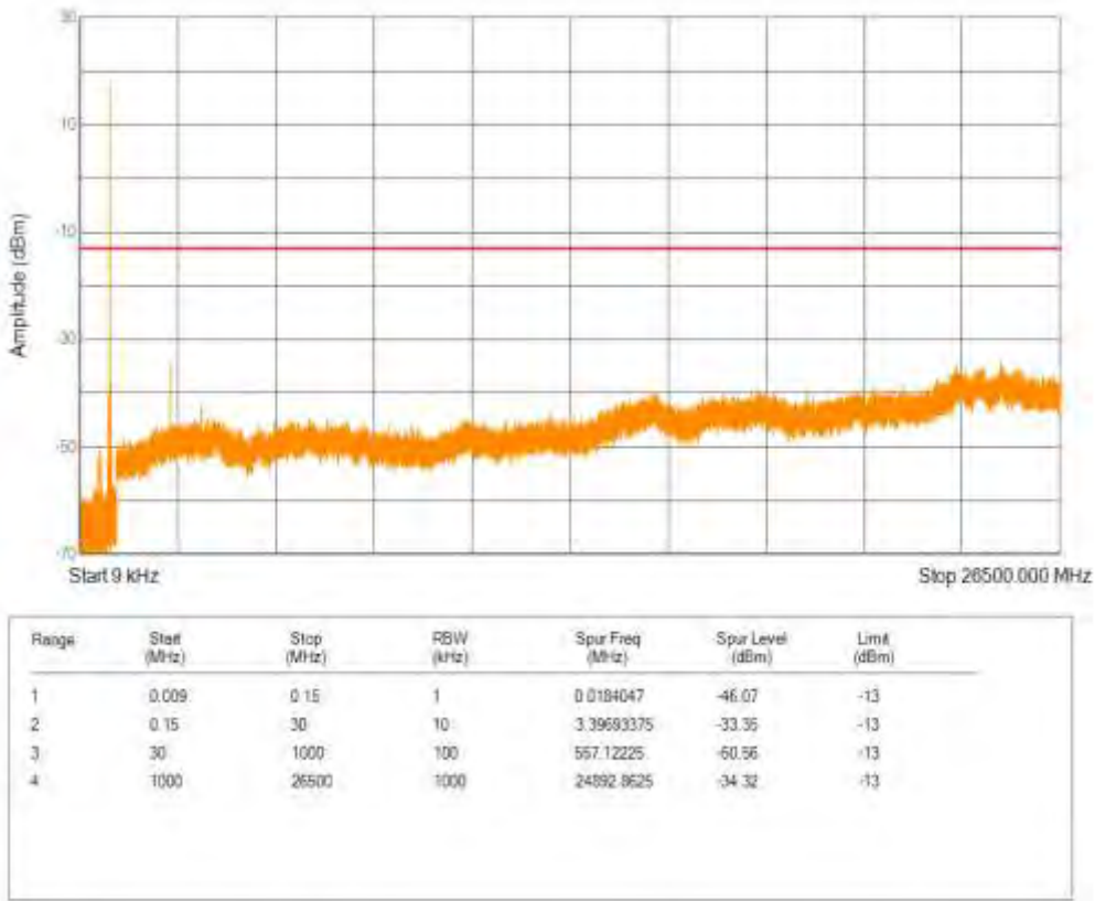
Band26(824-849) QPSK BW=15MHz Channel=26915 RB Size=1 Position=#0 NB Index=0
