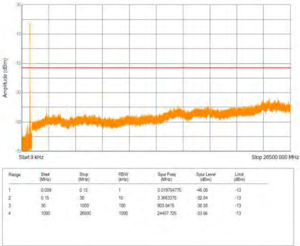
Band26(814-824) QPSK BW=1.4MHz Channel=26740 RB Size=1 Position=#0 NB Index=0
