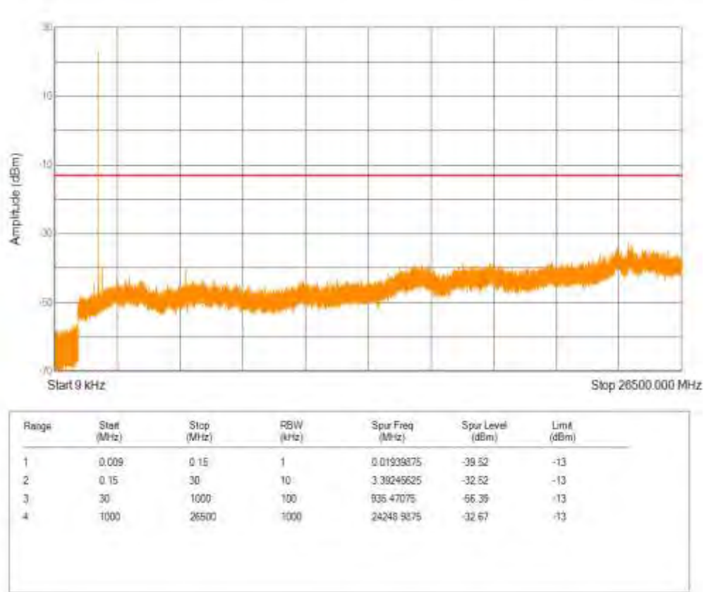
Band25 QPSK BW=15MHz Channel=26115 RB Size=6 Position=#0 NB Index=0
