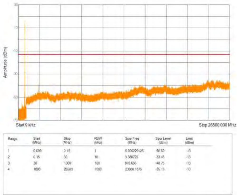
Band5 16QAM BW=3MHz Channel=20525 RB Size=1 Position=#0 NB Index=0
