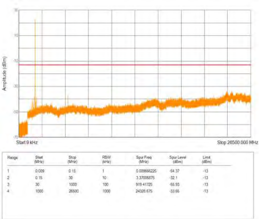
Band2 QPSK BW=15MHz Channel=18900 RB Size=6 Position=#0 NB Index=0
