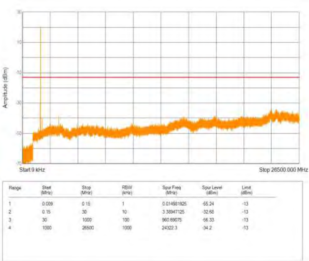
Band4 QPSK BW=15MHz Channel=20325 RB Size=6 Position=#0 NB Index=0
