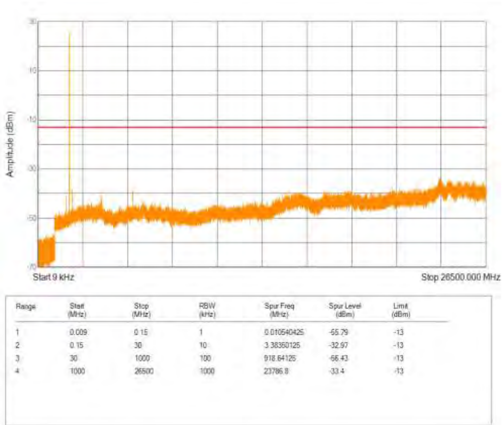
Band2 QPSK BW=20MHz Channel=18900 RB Size=6 Position=#0 NB Index=0
