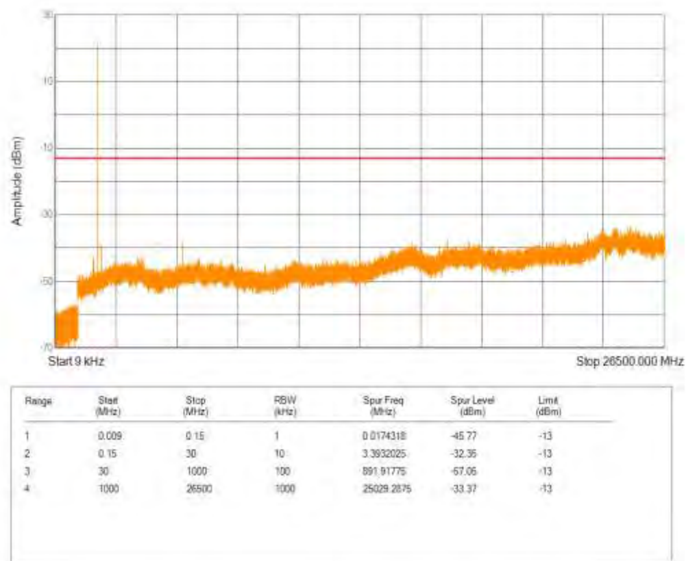
Band25 16QAM BW=20MHz Channel=26140 RB Size=1 Position=#0 NB Index=0
