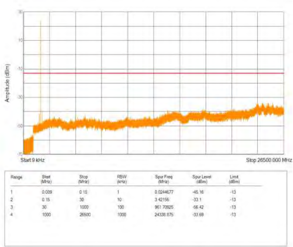
Band66 16QAM BW=20MHz Channel=132572 RB Size=1 Position=#0 NB Index=0
