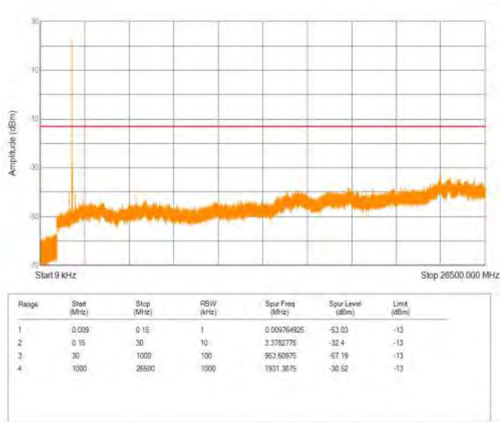
Band2 QPSK BW=5MHz Channel=19175 RB Size=6 Position=#0 NB Index=0
