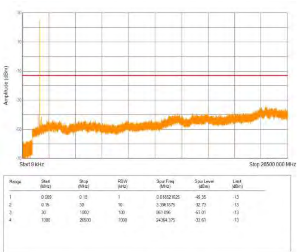
Band4 16QAM BW=5MHz Channel=20375 RB Size=5 Position=#0 NB Index=0
