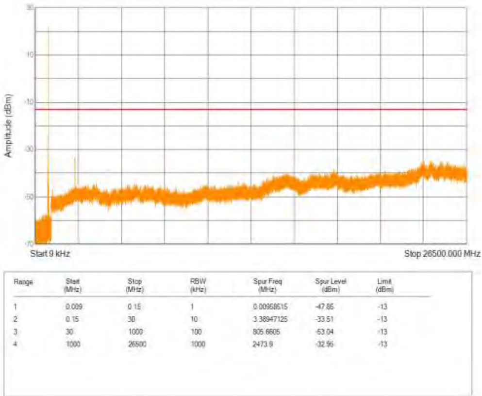
Band26(824-849) 16QAM BW=3MHz Channel=26805 RB Size=5 Position=#0 NB Index=0
