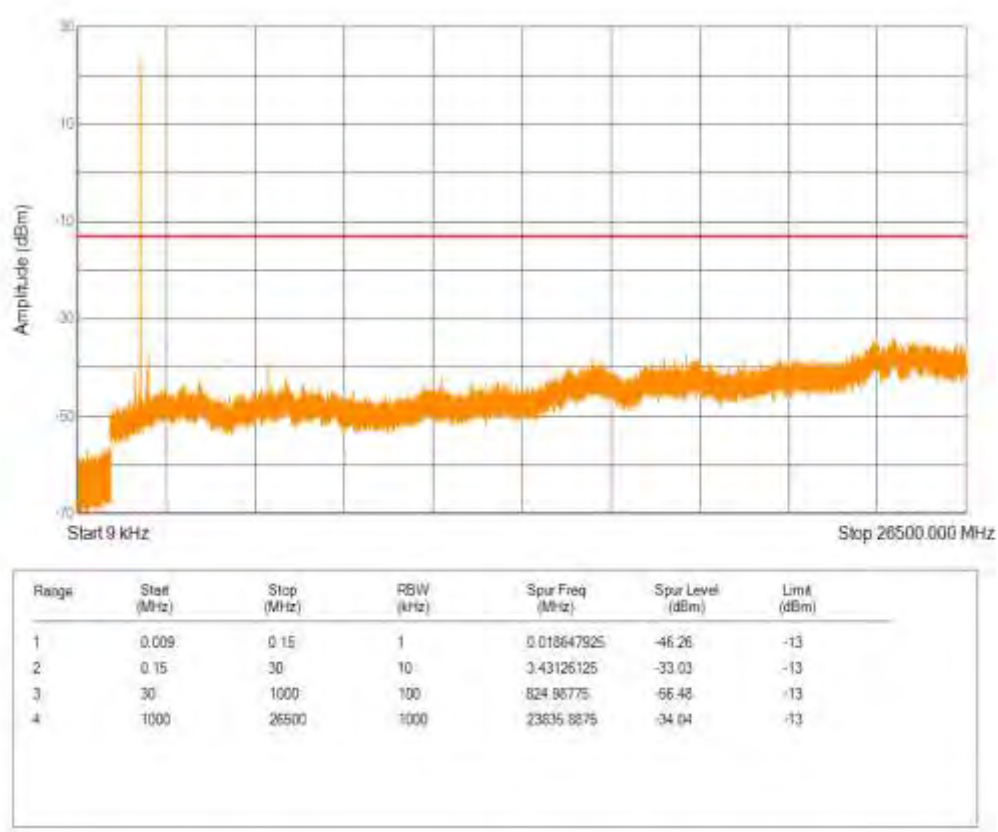
Band25 16QAM BW=15MHz Channel=26615 RB Size=1 Position=#0 NB Index=0
