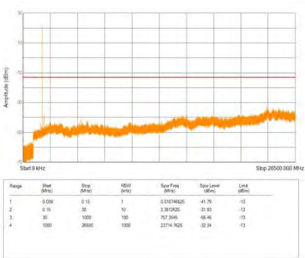
Band25 QPSK BW=1.4MHz Channel=26365 RB Size=6 Position=#0 NB Index=0
