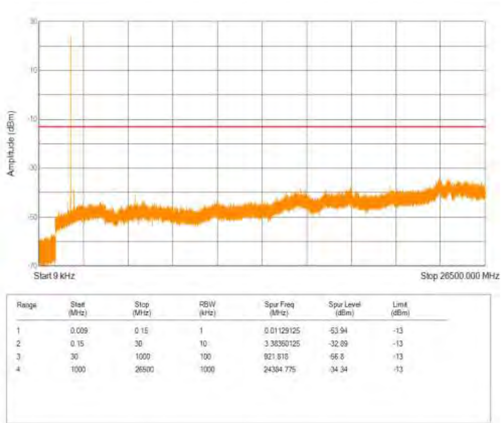
Band2 QPSK BW=3MHz Channel=19185 RB Size=6 Position=#0 NB Index=0
