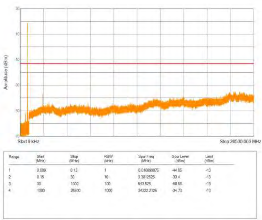
Band26(824-849) 16QAM BW=15MHz Channel=26965 RB Size=1 Position=#0 NB Index=0
