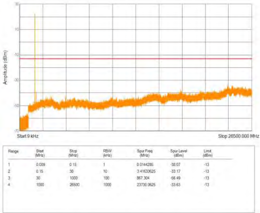
Band66 QPSK BW=1.4MHz Channel=132665 RB Size=1 Position=#0 NB Index=0
