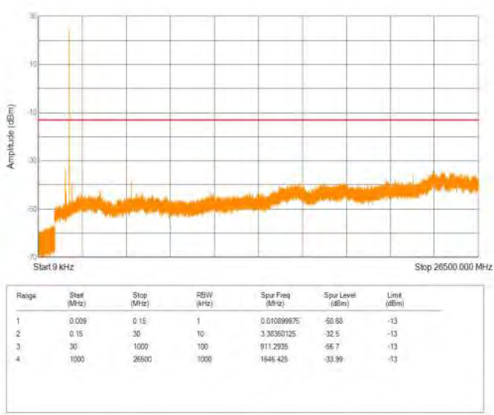
Band2 QPSK BW=10MHz Channel=19150 RB Size=1 Position=#0 NB Index=0
