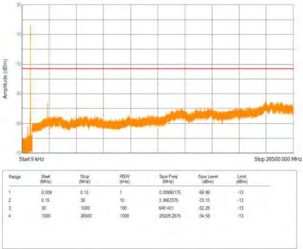
Band5 16QAM BW=10MHz Channel=20525 RB Size=1 Position=#0 NB Index=0
