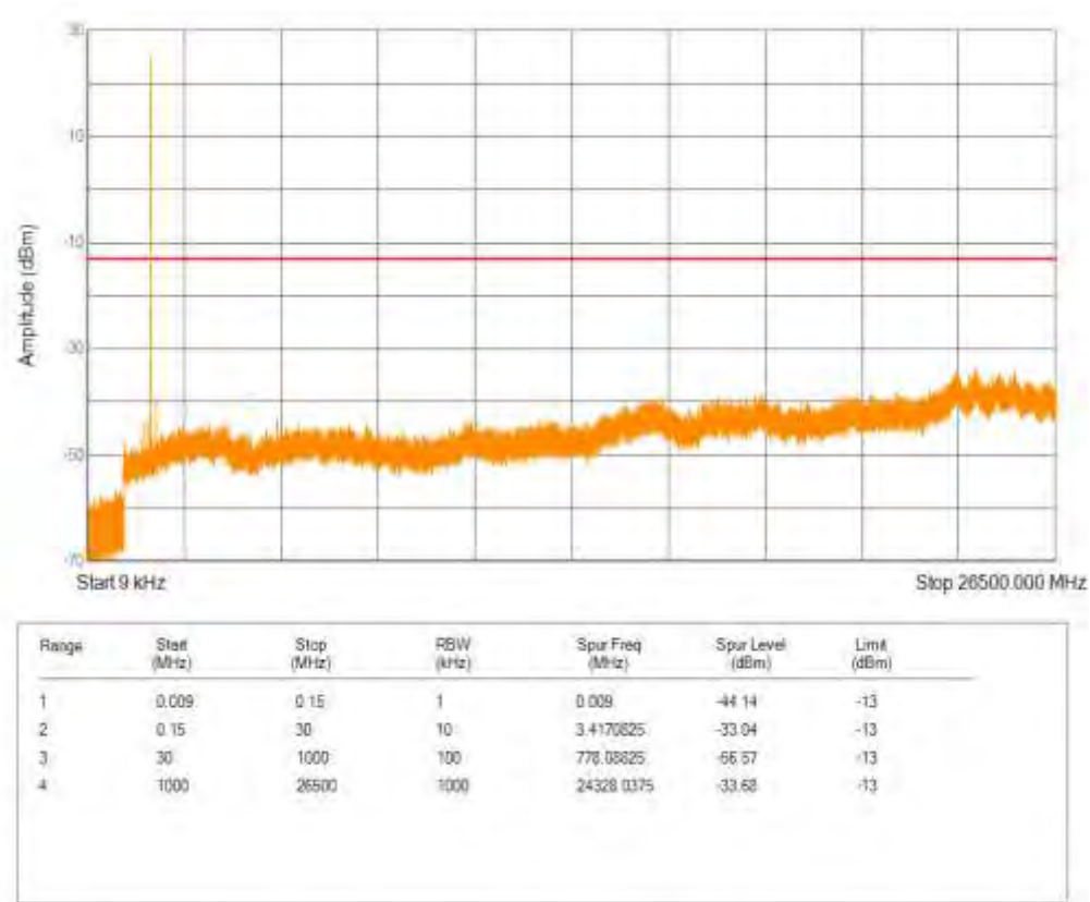
Band66 16QAM BW=20MHz Channel=132322 RB Size=5 Position=#0 NB Index=0
