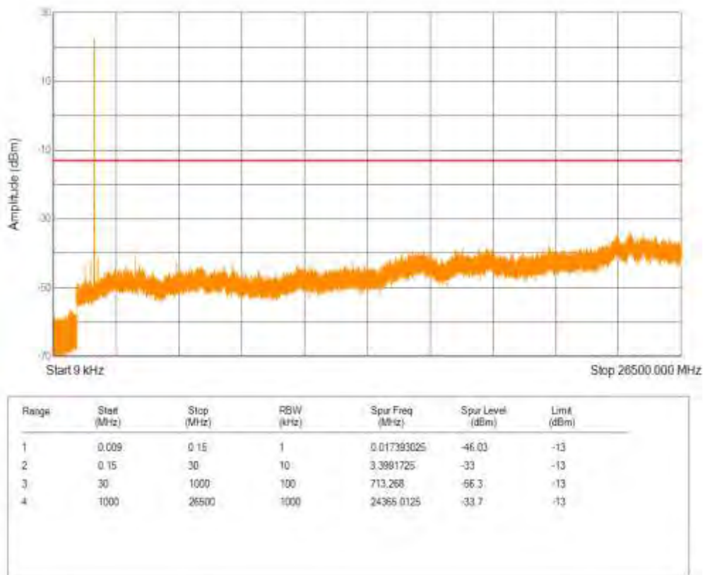
Band66 QPSK BW=10MHz Channel=132622 RB Size=1 Position=#0 NB Index=0
