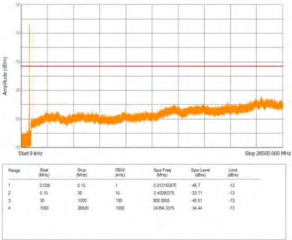
Band26(824-849) 16QAM BW=3MHz Channel=26915 RB Size=1 Position=#0 NB Index=0
