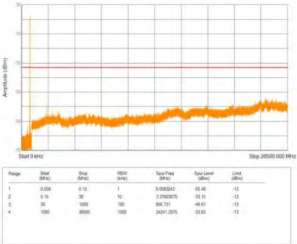
Band5 16QAM BW=1.4MHz Channel=20525 RB Size=5 Position=#0 NB Index=0
