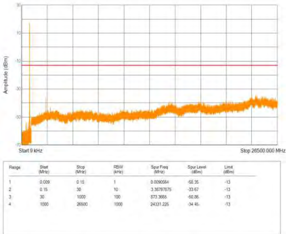
Band5 16QAM BW=5MHz Channel=20625 RB Size=1 Position=#0 NB Index=0
