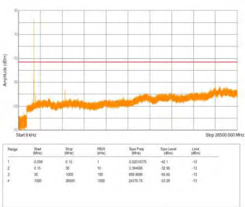
Band25 16QAM BW=1.4MHz Channel=26365 RB Size=5 Position=#0 NB Index=0
