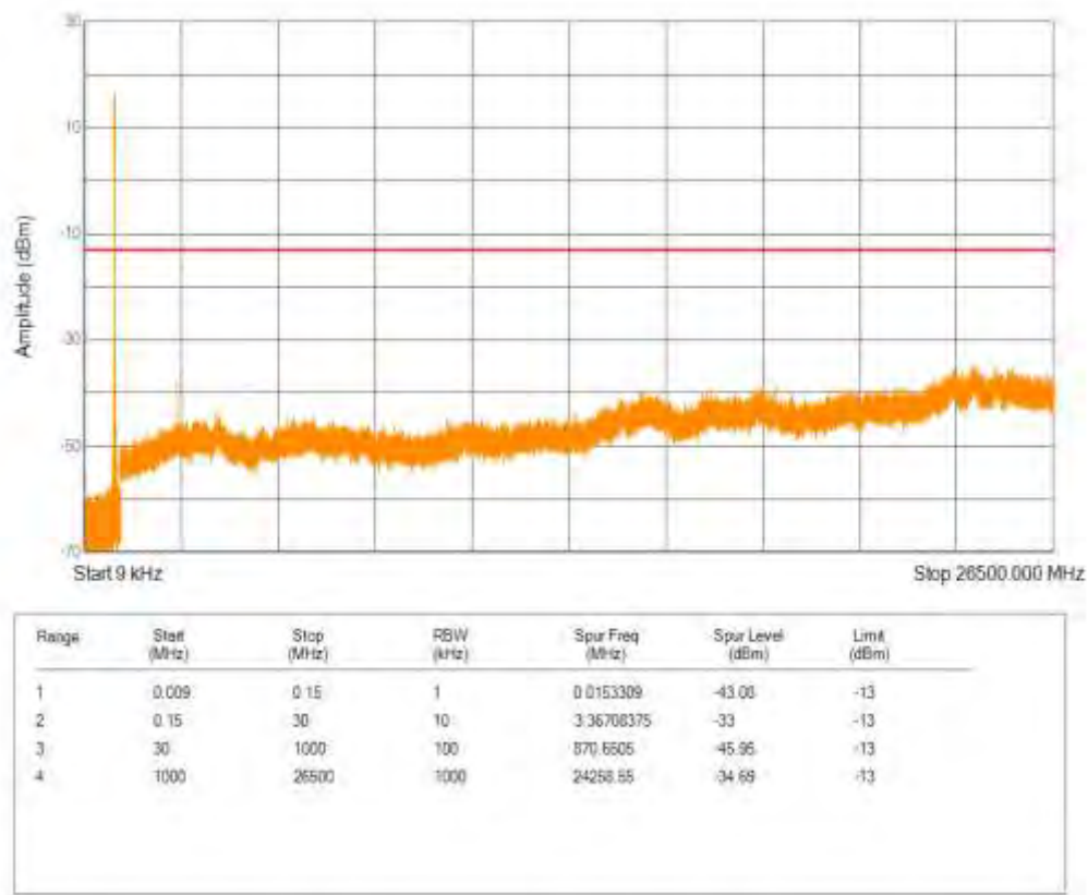
Band26(824-849) QPSK BW=5MHz Channel=26815 RB Size=1 Position=#0 NB Index=0
