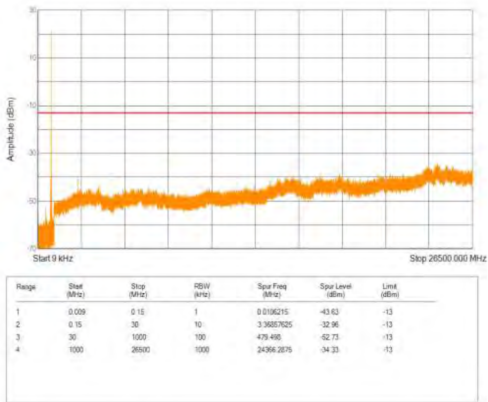
Band26(824-849) QPSK BW=15MHz Channel=26865 RB Size=6 Position=#0 NB Index=0
