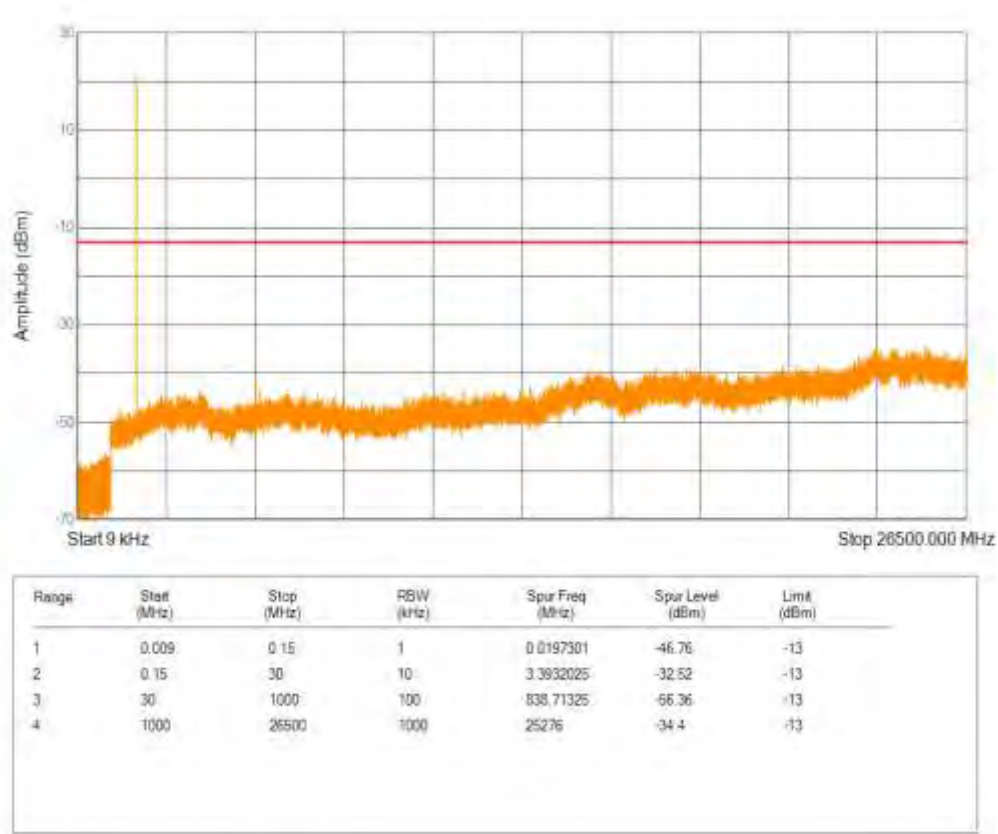
Band66 QPSK BW=10MHz Channel=132022 RB Size=1 Position=#0 NB Index=0
