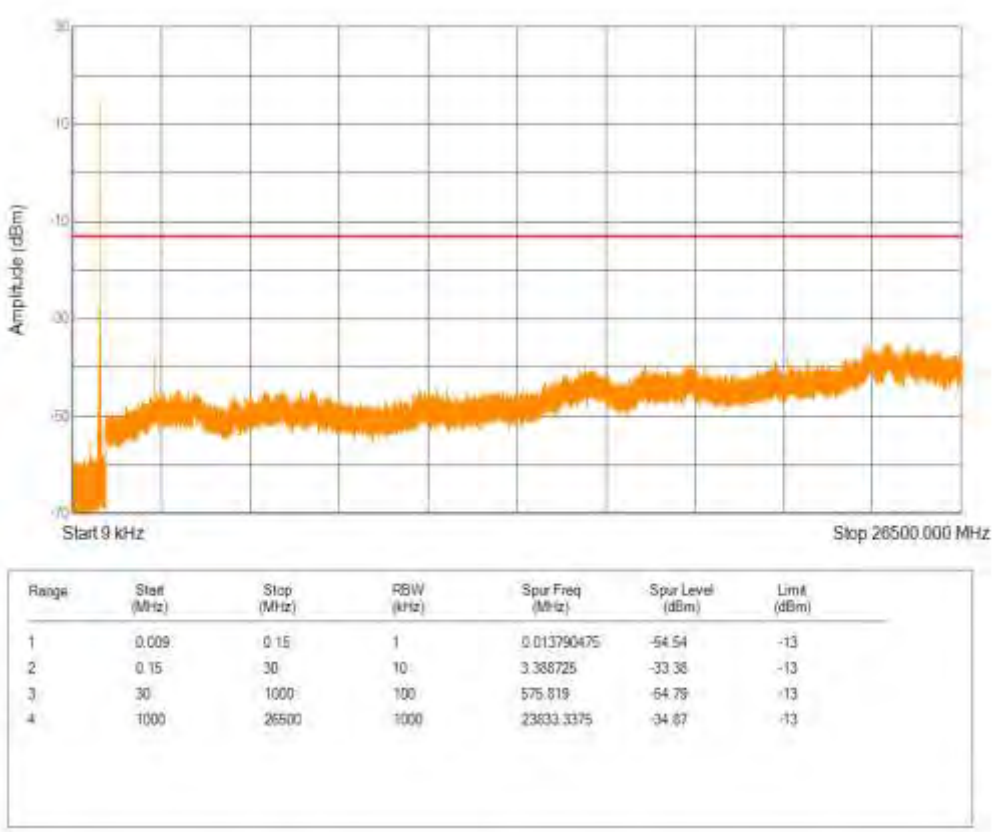
Band5 16QAM BW=10MHz Channel=20450 RB Size=1 Position=#0 NB Index=0
