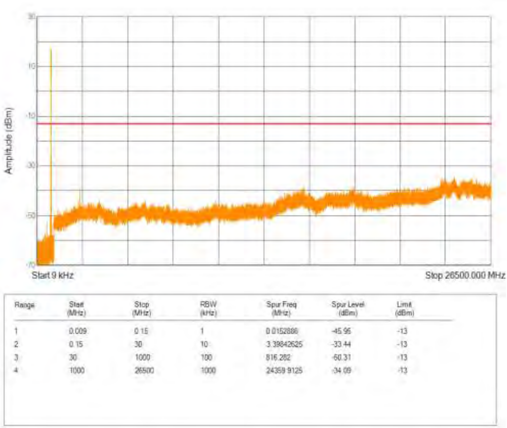
Band26(824-849) QPSK BW=1.4MHz Channel=27033 RB Size=1 Position=#0 NB Index=0
