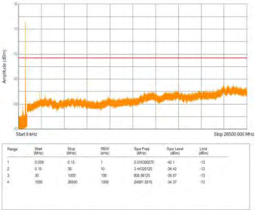
Band26(814-824) 16QAM BW=1.4MHz Channel=26697 RB Size=1 Position=#0 NB Index=0
