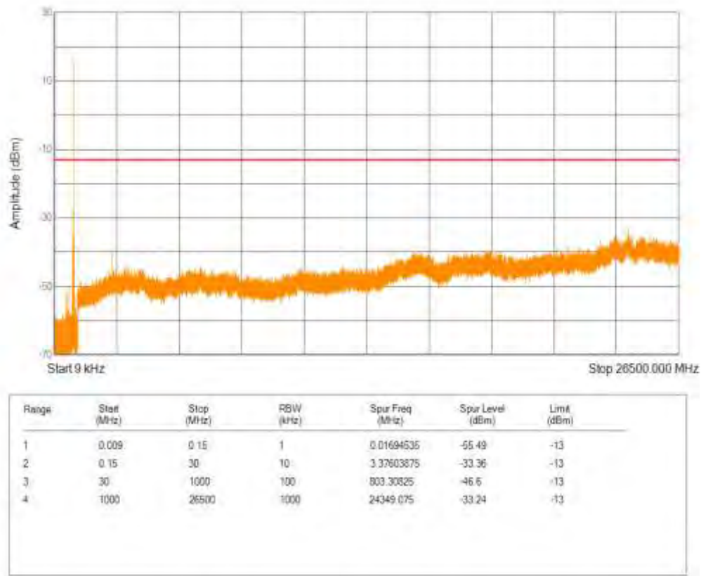
Band5 16QAM BW=5MHz Channel=20425 RB Size=1 Position=#0 NB Index=0
