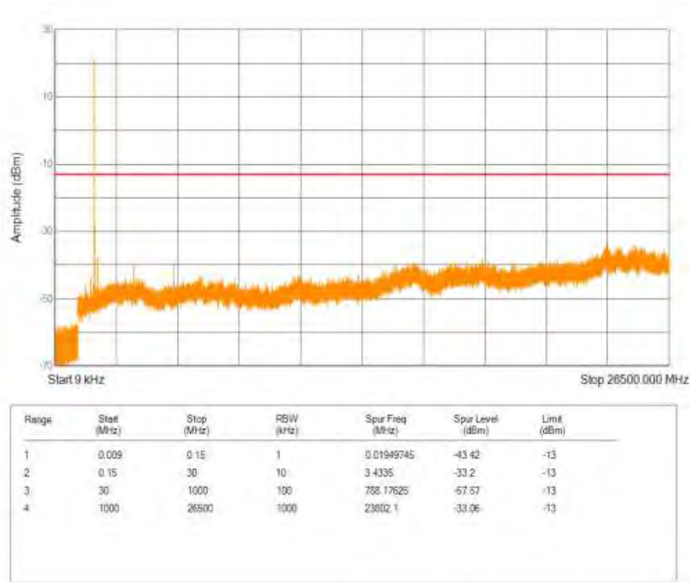
Band66 16QAM BW=5MHz Channel=131997 RB Size=5 Position=#0 NB Index=0
