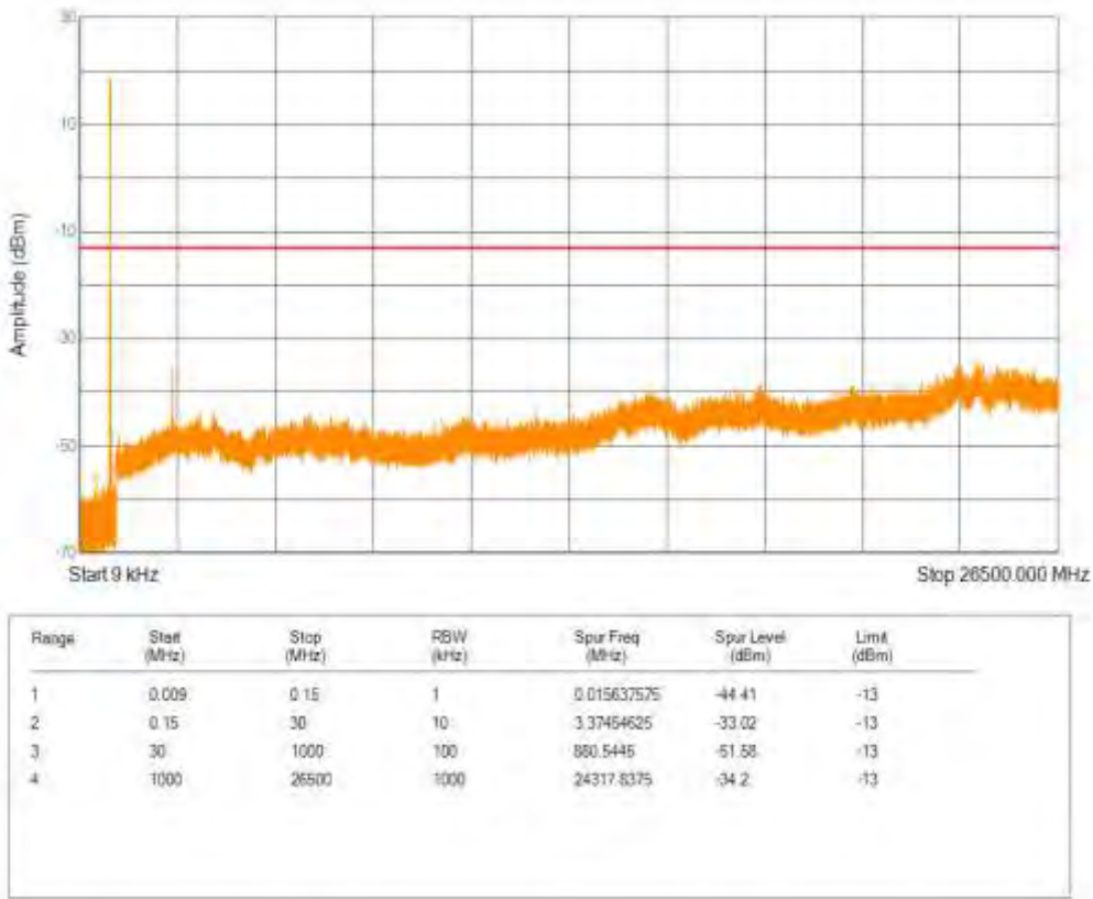
Band26(824-849) 16QAM BW=5MHz Channel=27015 RB Size=1 Position=#0 NB Index=0
