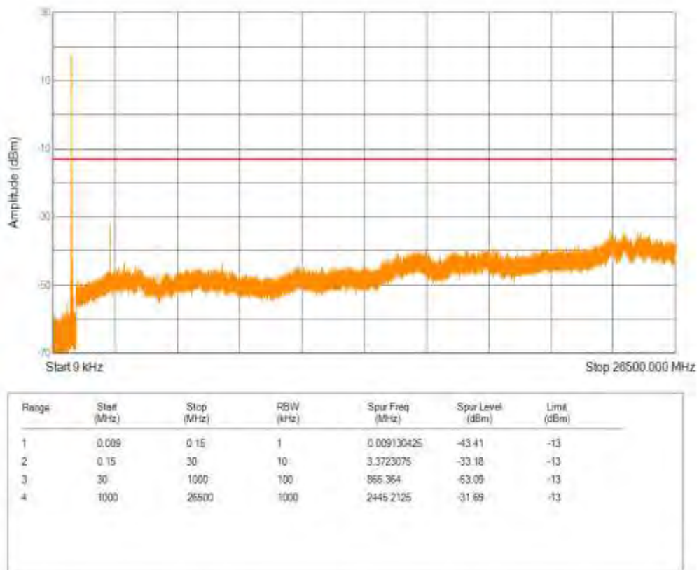
Band26(824-849) QPSK BW=1.4MHz Channel=26797 RB Size=1 Position=#0 NB Index=0
