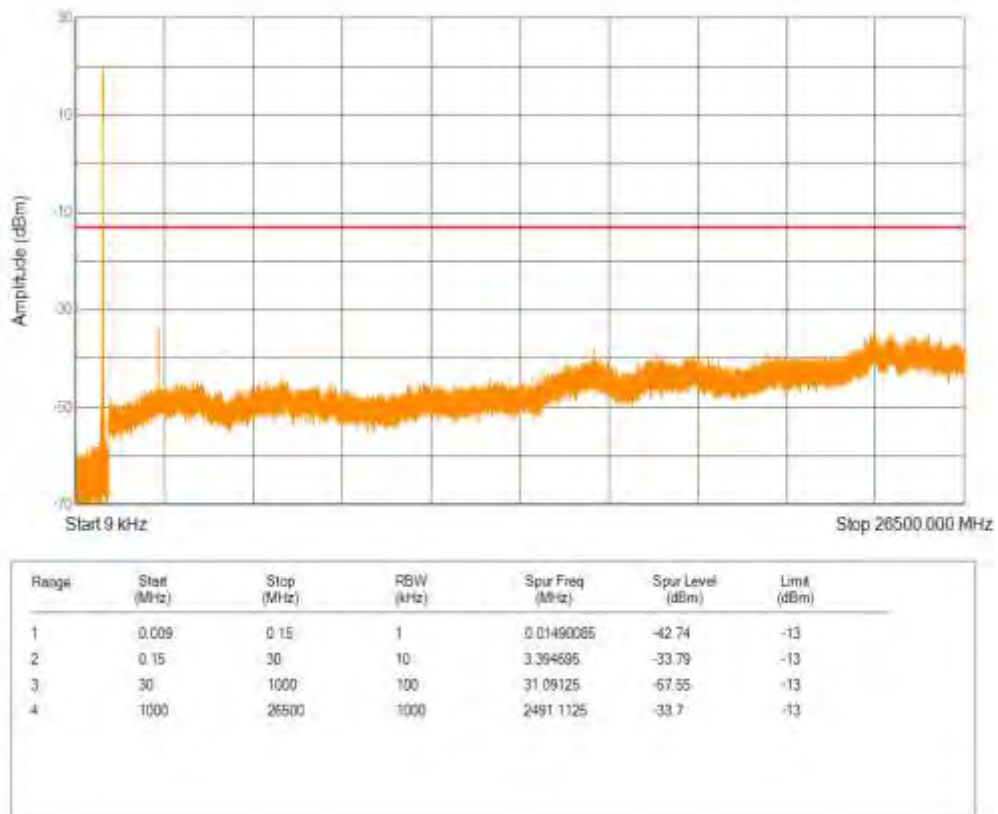
Band26(824-849) QPSK BW=15MHz Channel=26965 RB Size=1 Position=#0 NB Index=0
