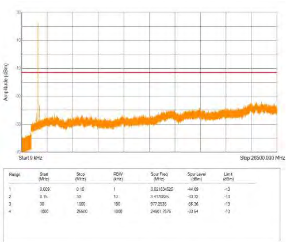
Band66 16QAM BW=1.4MHz Channel=131979 RB Size=5 Position=#0 NB Index=0
