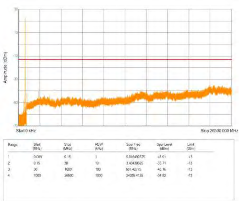
Band26(824-849) QPSK BW=15MHz Channel=26965 RB Size=6 Position=#0 NB Index=0
