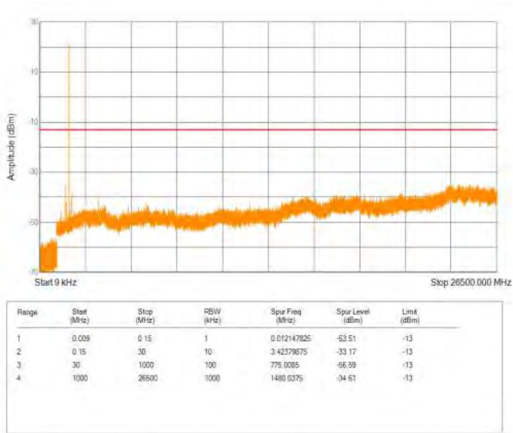
Band4 QPSK BW=3MHz Channel=19965 RB Size=6 Position=#0 NB Index=0
