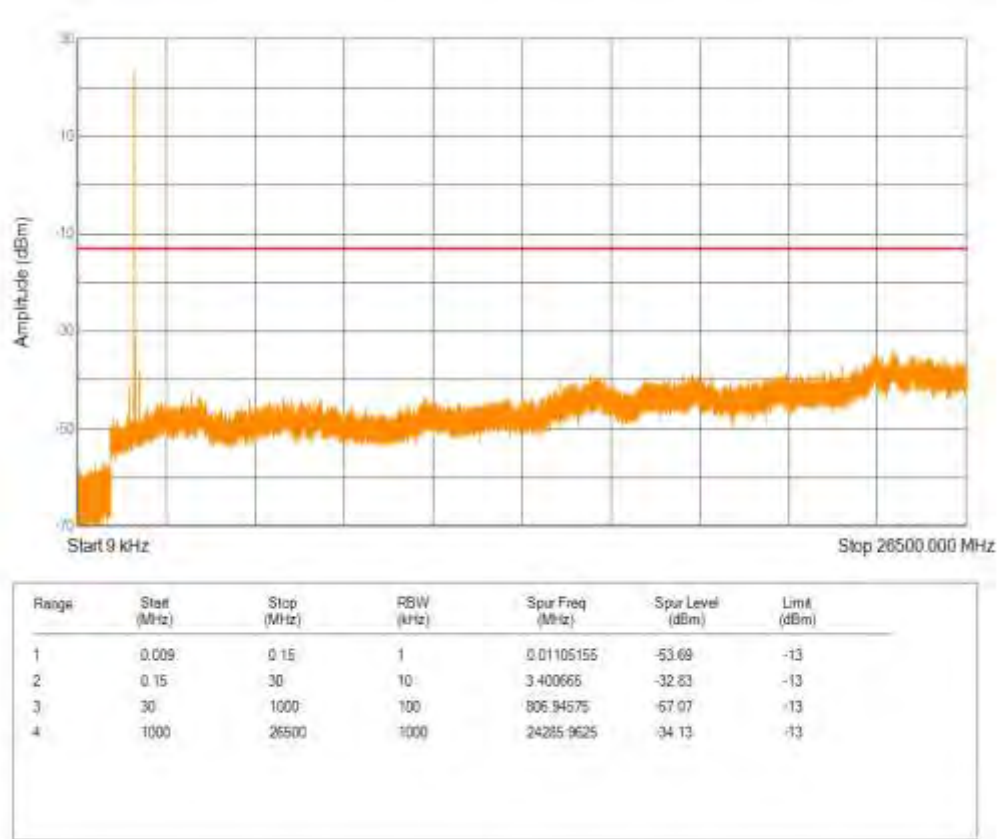
Band4 QPSK BW=15MHz Channel=20025 RB Size=6 Position=#0 NB Index=0
