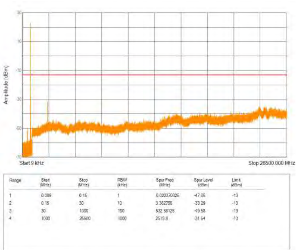
Band26(824-849) 16QAM BW=10MHz Channel=26990 RB Size=5 Position=#0 NB Index=0
