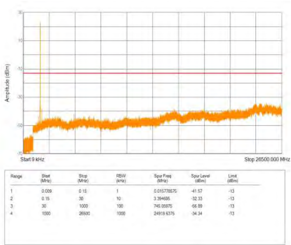
Band66 16QAM BW=15MHz Channel=132322 RB Size=1 Position=#0 NB Index=0
