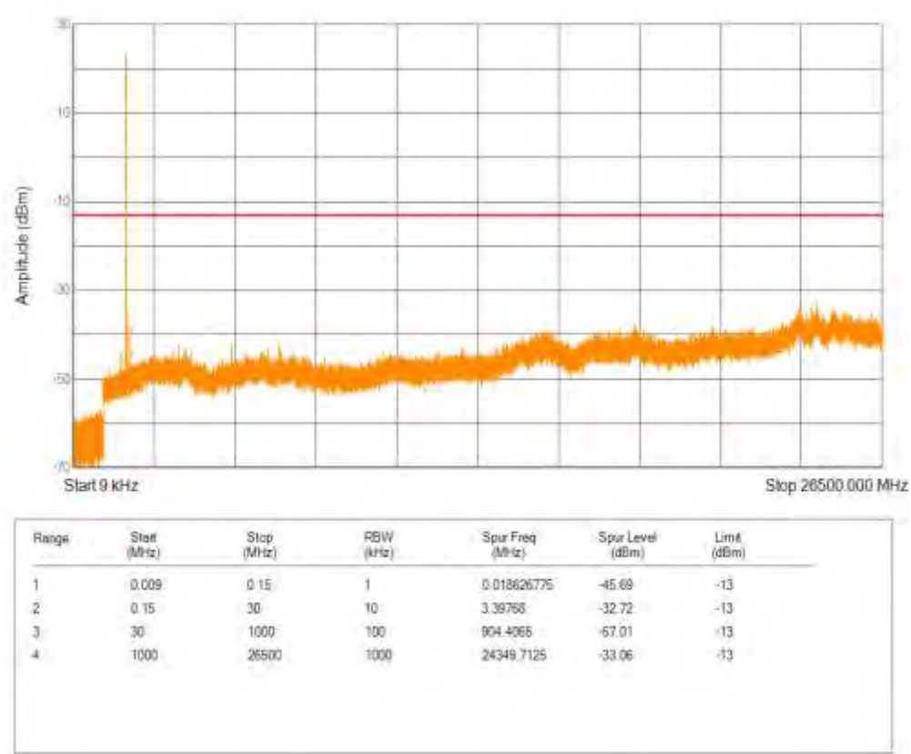
Band66 QPSK BW=20MHz Channel=132572 RB Size=1 Position=#0 NB Index=0
