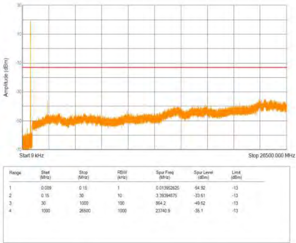
Band5 QPSK BW=3MHz Channel=20635 RB Size=1 Position=#0 NB Index=0
