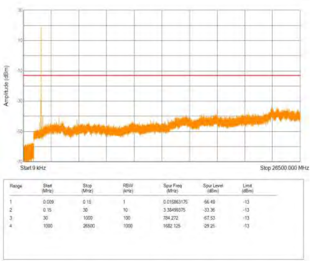
Band4 16QAM BW=5MHz Channel=19975 RB Size=1 Position=#0 NB Index=0
