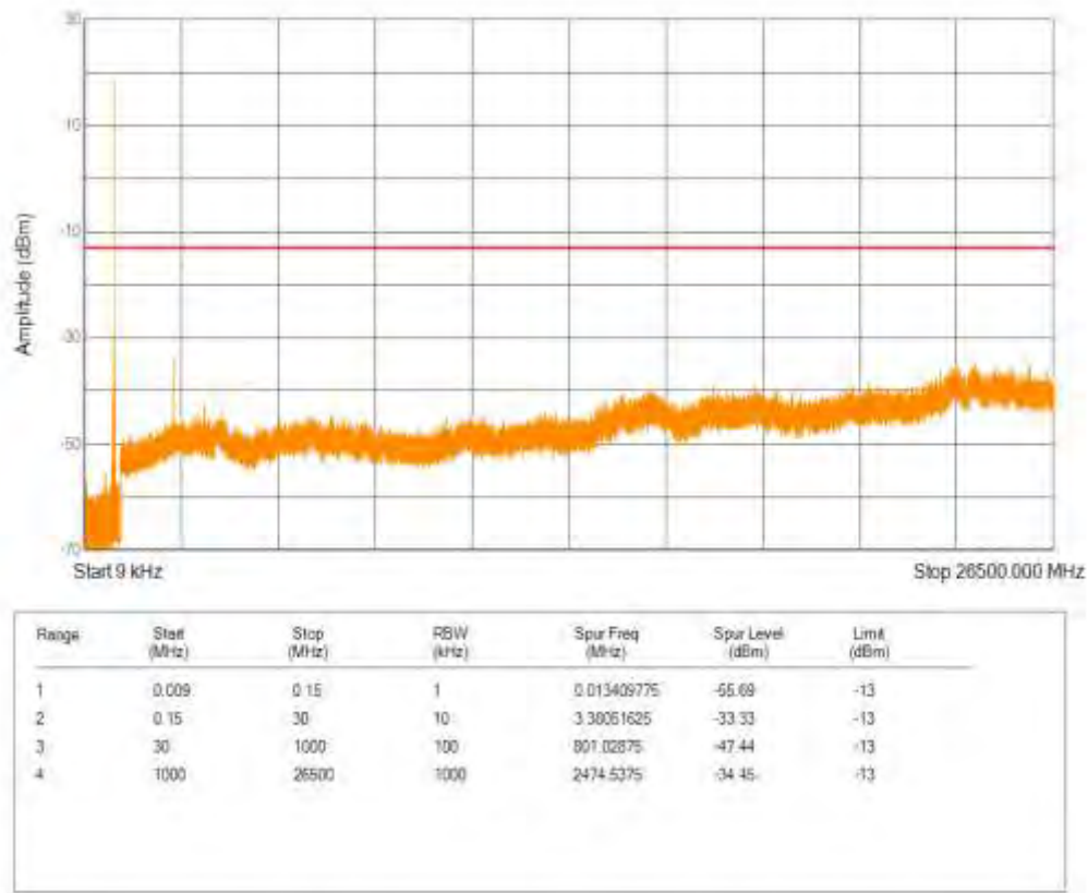
Band5 QPSK BW=5MHz Channel=20525 RB Size=1 Position=#0 NB Index=0
