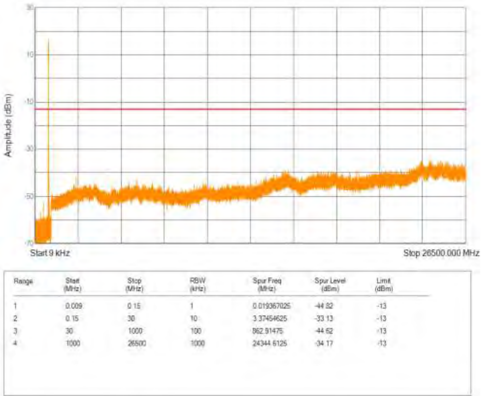
Band26(824-849) 16QAM BW=3MHz Channel=27025 RB Size=1 Position=#0 NB Index=0
