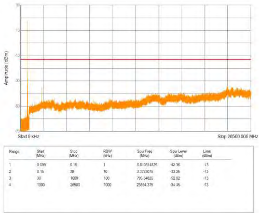
Band26(824-849) 16QAM BW=5MHz Channel=26815 RB Size=1 Position=#0 NB Index=0
