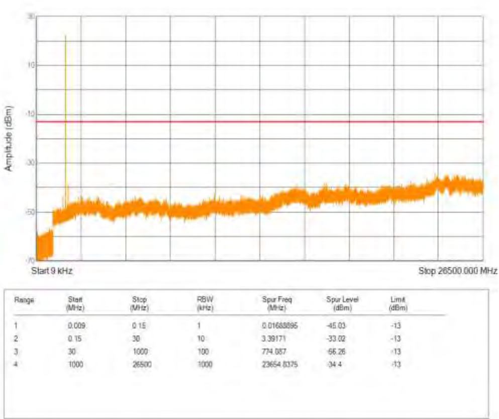
Band66 16QAM BW=10MHz Channel=132322 RB Size=1 Position=#0 NB Index=0
