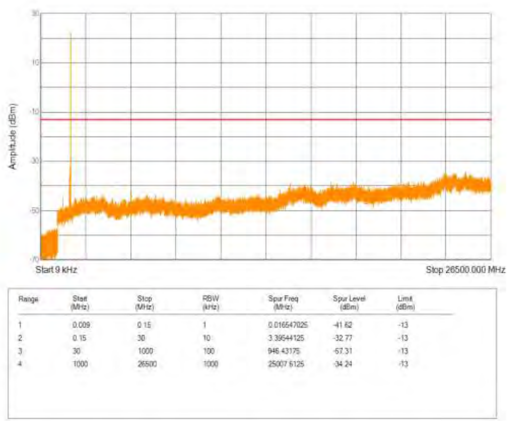
Band66 QPSK BW=5MHz Channel=131997 RB Size=1 Position=#0 NB Index=0
