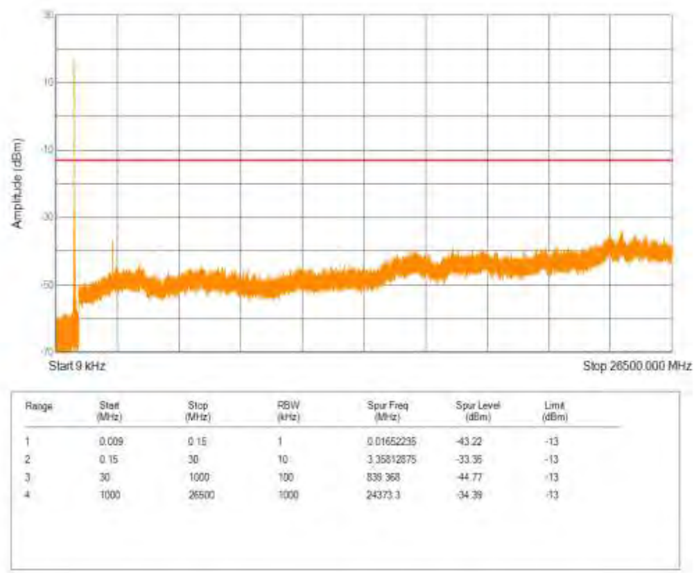
Band26(814-824) 16QAM BW=3MHz Channel=26740 RB Size=1 Position=#0 NB Index=0
