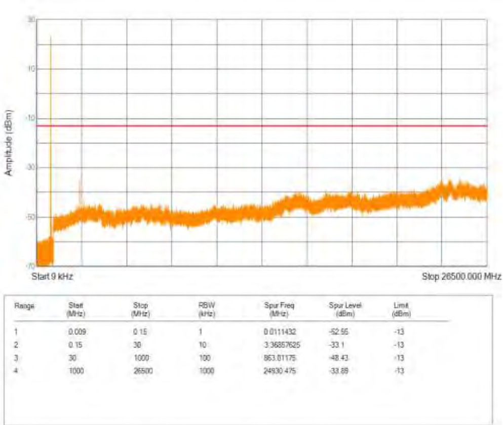
Band5 16QAM BW=1.4MHz Channel=20643 RB Size=5 Position=#0 NB Index=0
