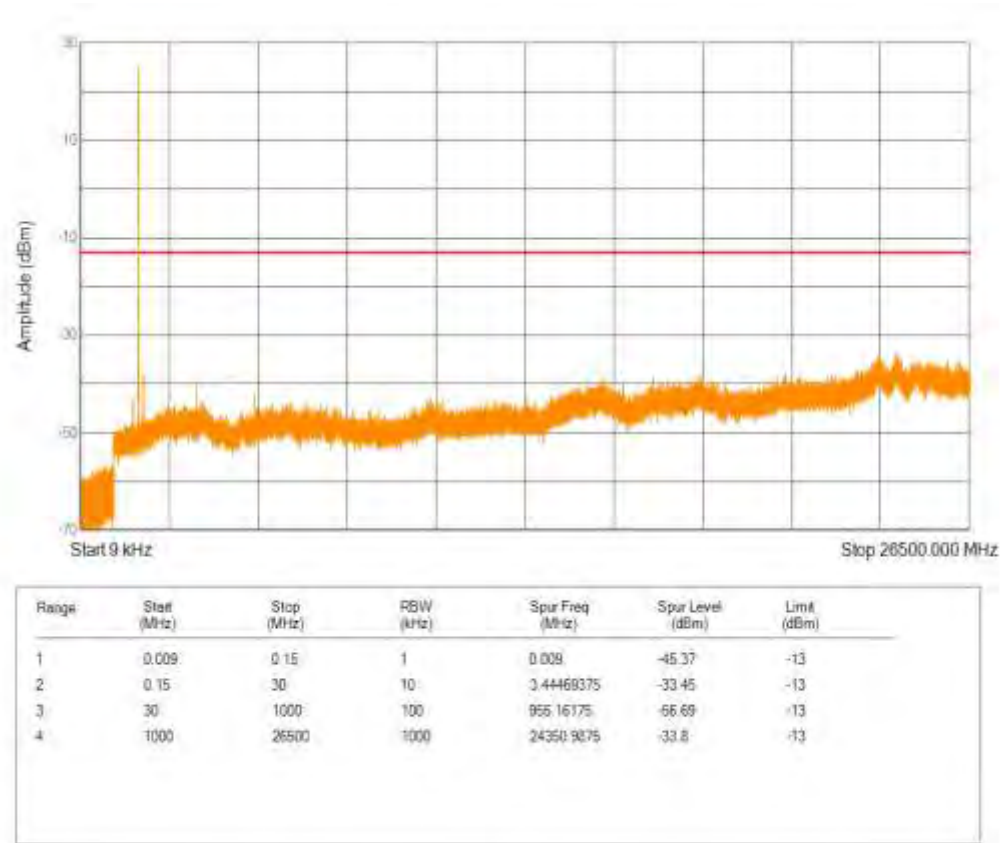
Band66 QPSK BW=15MHz Channel=132322 RB Size=6 Position=#0 NB Index=0
