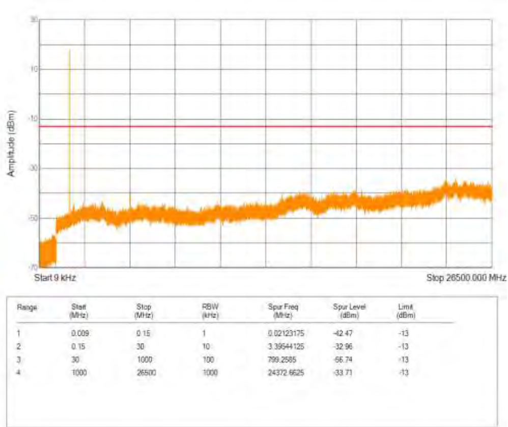
Band66 16QAM BW=1.4MHz Channel=132665 RB Size=5 Position=#0 NB Index=0
