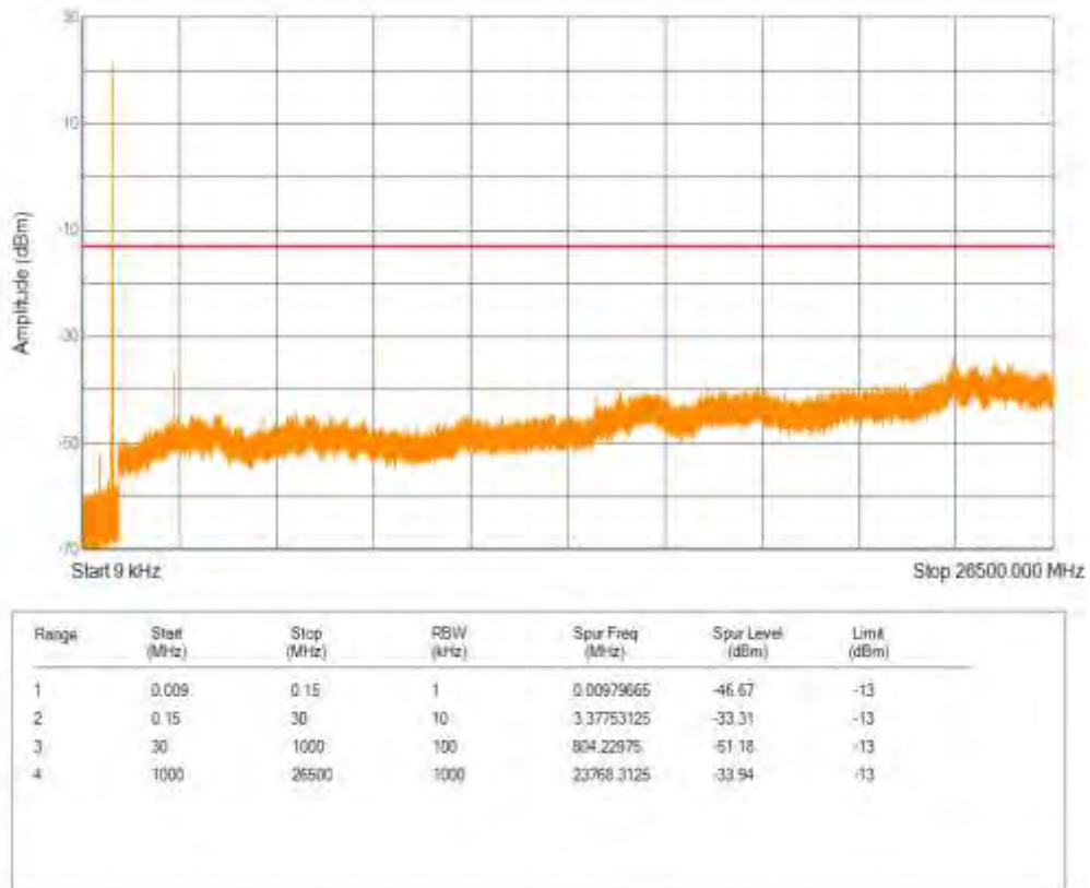
Band26(824-849) 16QAM BW=3MHz Channel=26915 RB Size=5 Position=#0 NB Index=0
