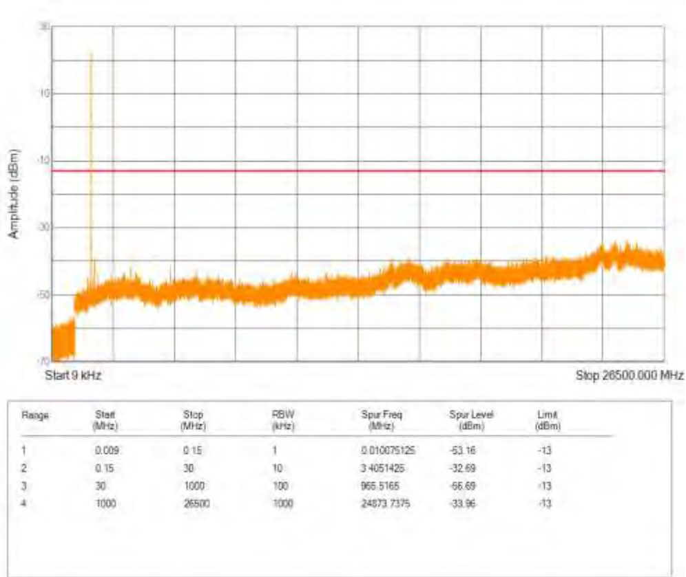
Band4 QPSK BW=5MHz Channel=19975 RB Size=6 Position=#0 NB Index=0
