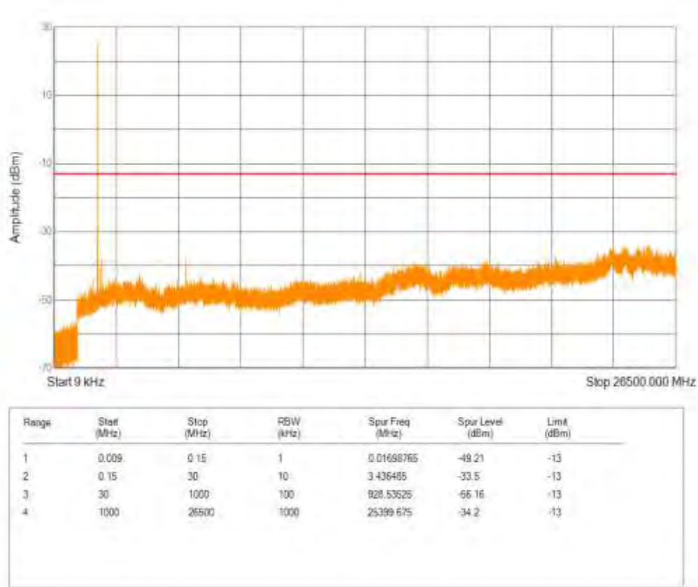
Band2 16QAM BW=10MHz Channel=18900 RB Size=5 Position=#0 NB Index=0
