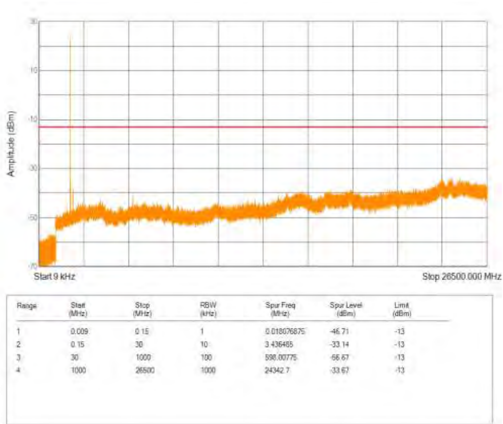
Band25 16QAM BW=20MHz Channel=26140 RB Size=5 Position=#0 NB Index=0
