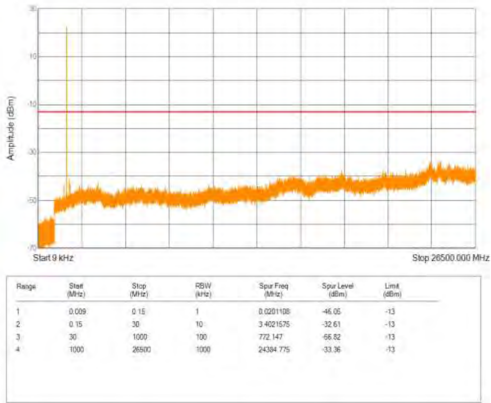
Band66 QPSK BW=5MHz Channel=132647 RB Size=1 Position=#0 NB Index=0
