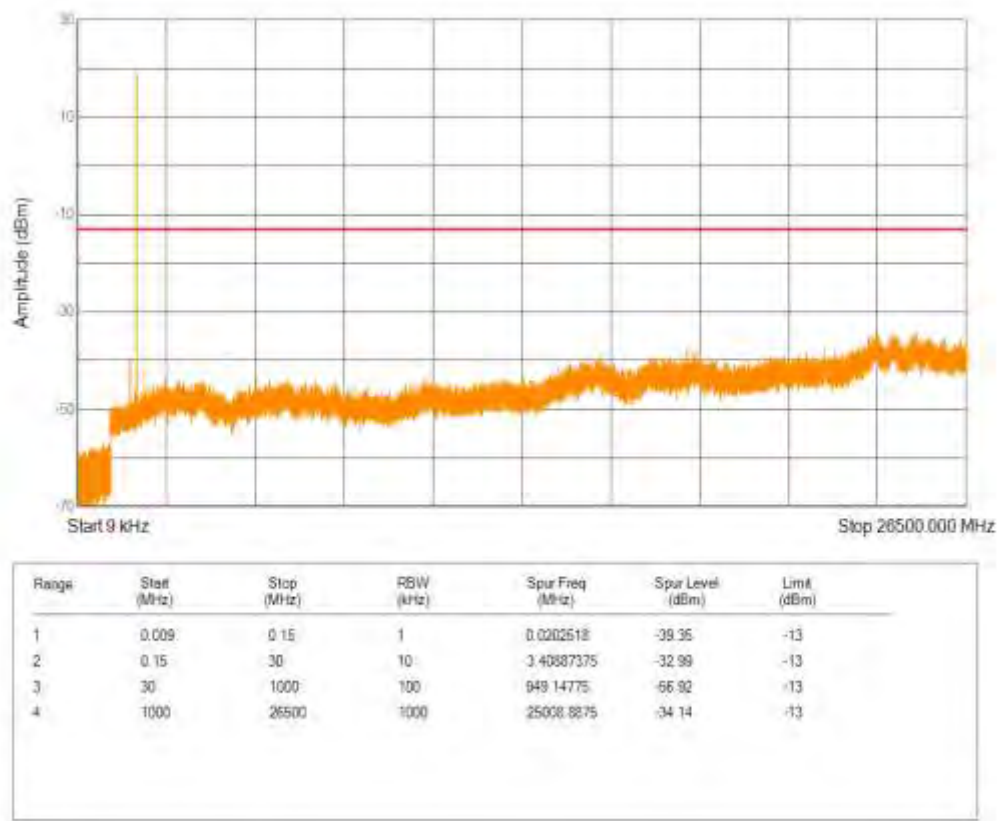
Band66 16QAM BW=3MHz Channel=132657 RB Size=1 Position=#0 NB Index=0
