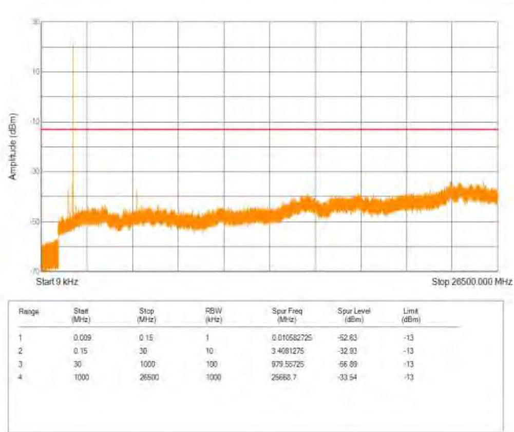
Band2 QPSK BW=20MHz Channel=18700 RB Size=6 Position=#0 NB Index=0
