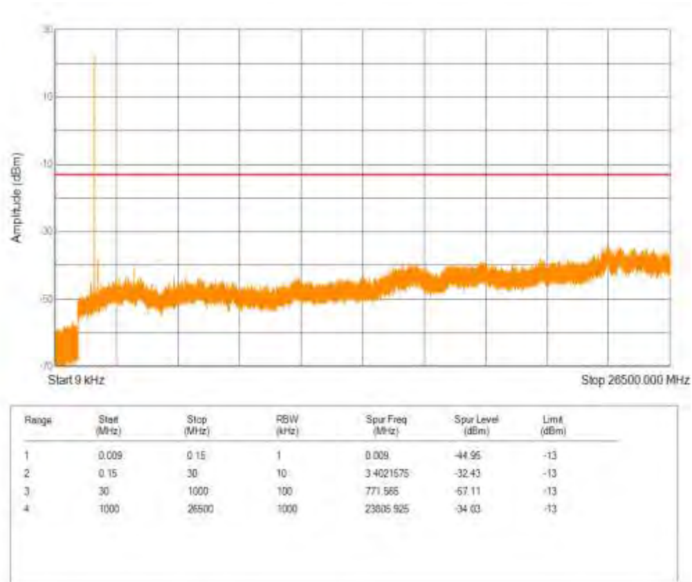
Band66 16QAM BW=5MHz Channel=131997 RB Size=1 Position=#0 NB Index=0
