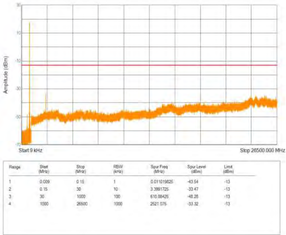
Band26(824-849) QPSK BW=15MHz Channel=26865 RB Size=1 Position=#0 NB Index=0
