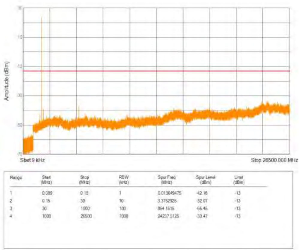
Band25 QPSK BW=10MHz Channel=26365 RB Size=1 Position=#0 NB Index=0
