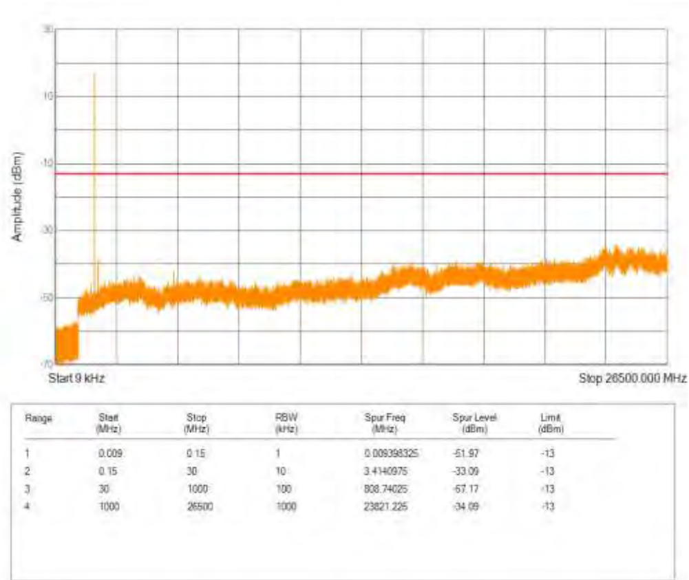
Band4 16QAM BW=3MHz Channel=19965 RB Size=5 Position=#0 NB Index=0
