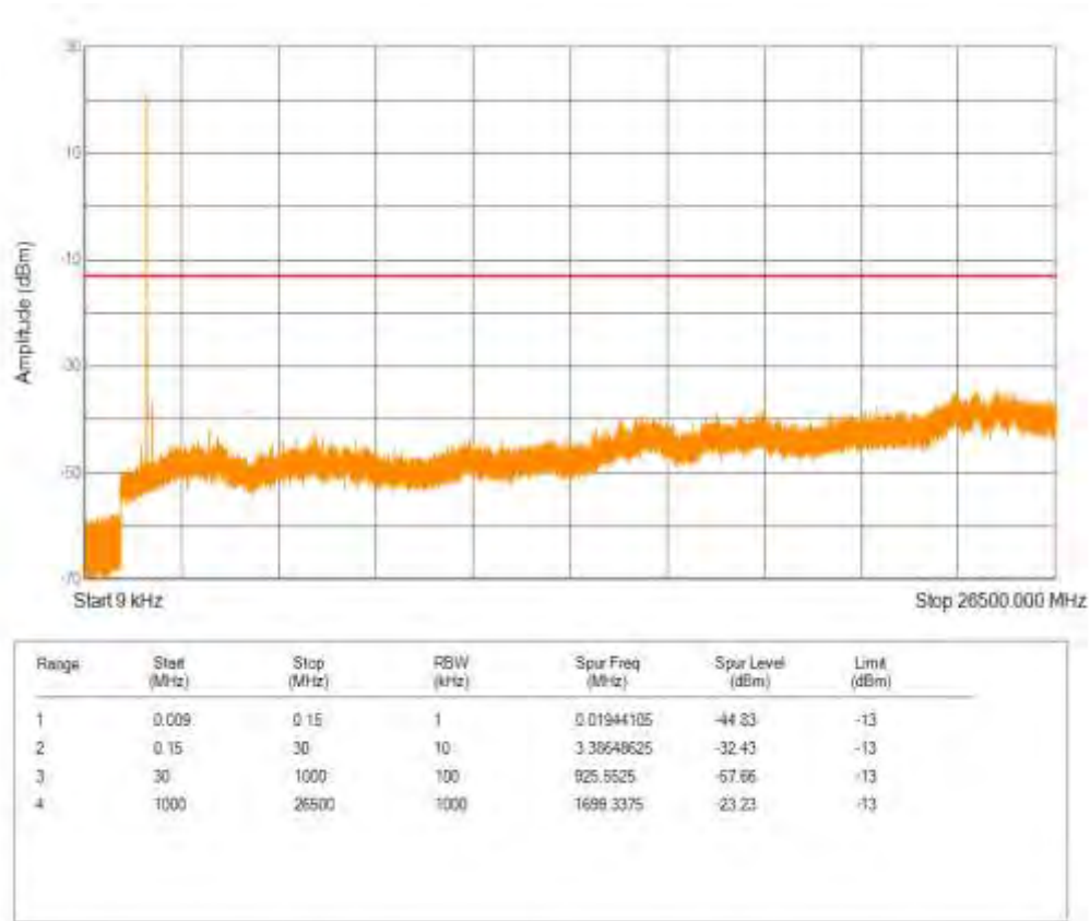
Band66 QPSK BW=1.4MHz Channel=131979 RB Size=6 Position=#0 NB Index=0
