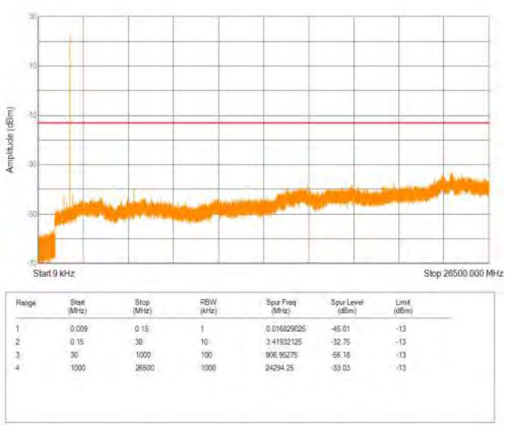
Band25 QPSK BW=10MHz Channel=26640 RB Size=1 Position=#0 NB Index=0
