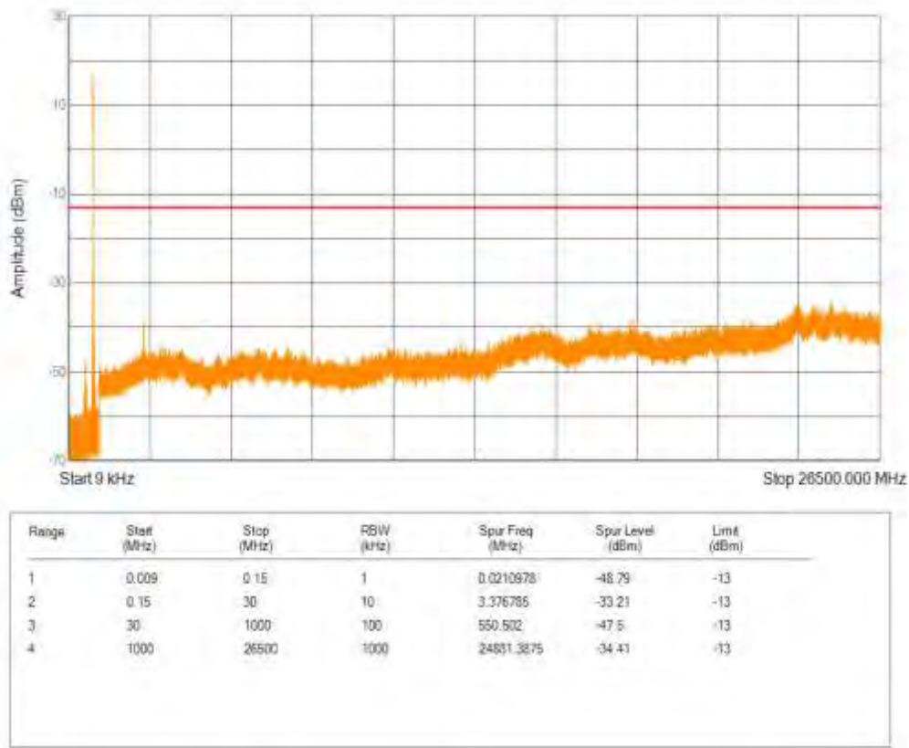
Band26(814-824) QPSK BW=10MHz Channel=26740 RB Size=1 Position=#0 NB Index=0
