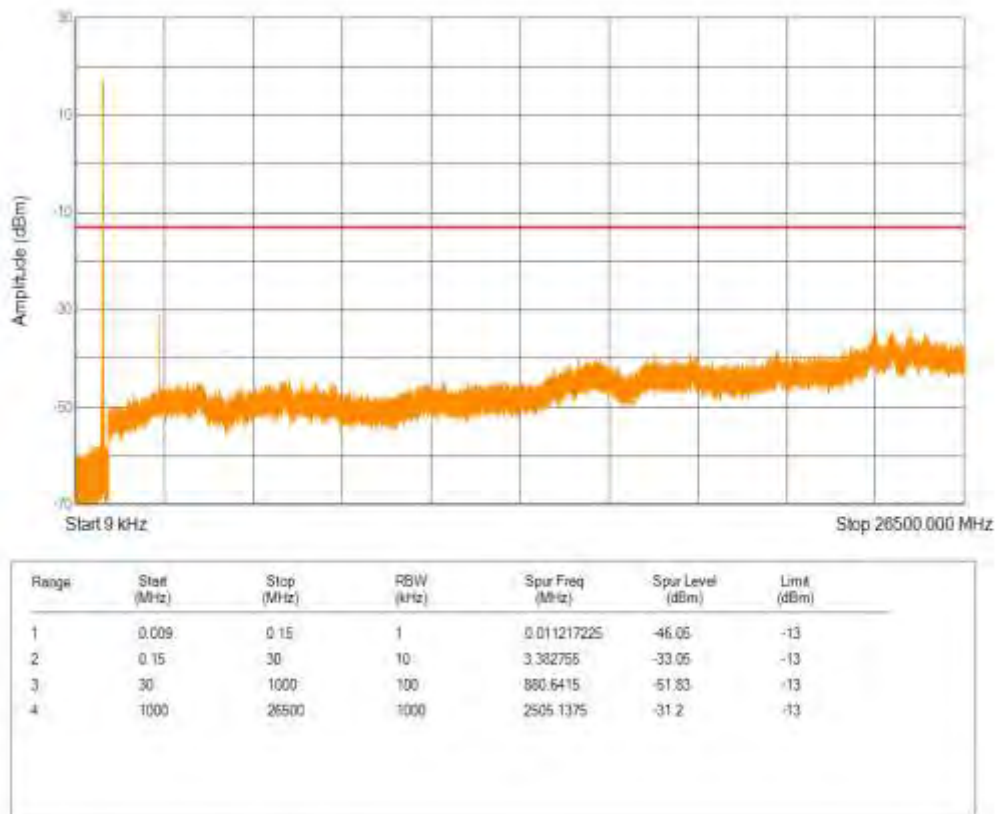
Band26(824-849) QPSK BW=5MHz Channel=27015 RB Size=1 Position=#0 NB Index=0
