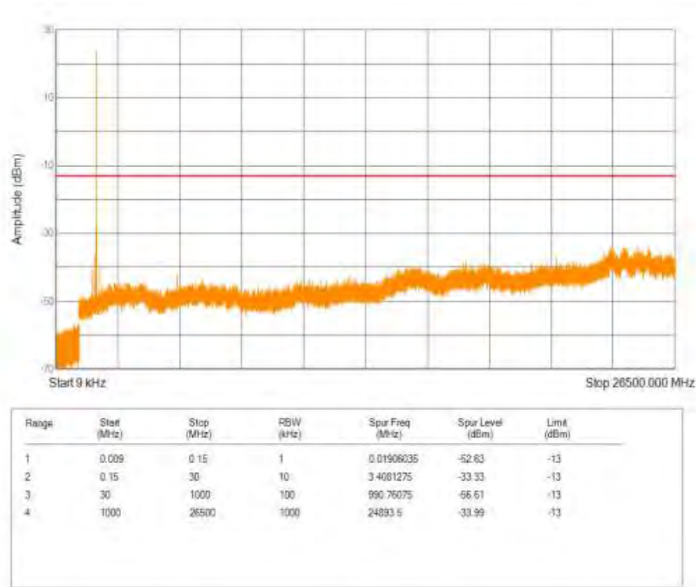
Band4 QPSK BW=1.4MHz Channel=20175 RB Size=6 Position=#0 NB Index=0
