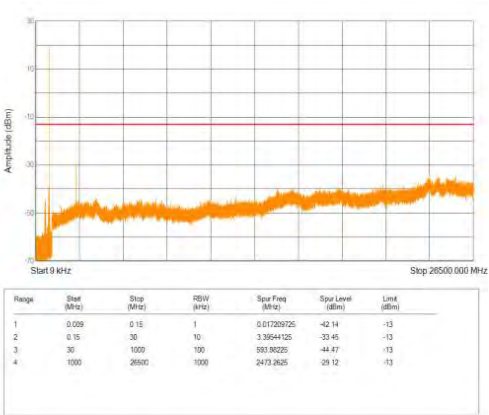
Band26(824-849) 16QAM BW=5MHz Channel=26815 RB Size=5 Position=#0 NB Index=0
