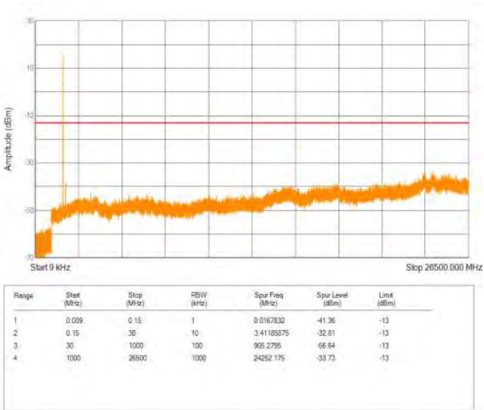
Band66 16QAM BW=3MHz Channel=131987 RB Size=5 Position=#0 NB Index=0
