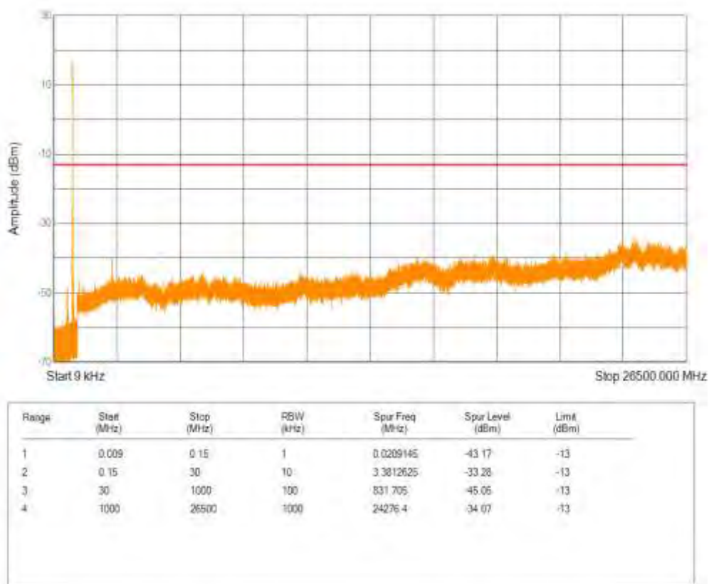
Band26(814-824) QPSK BW=1.4MHz Channel=26783 RB Size=1 Position=#0 NB Index=0
