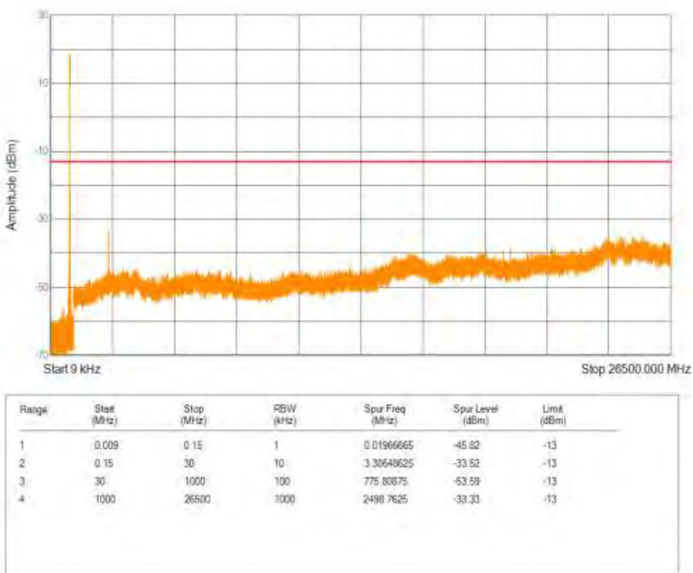
Band26(824-849) QPSK BW=10MHz Channel=26990 RB Size=1 Position=#0 NB Index=0
