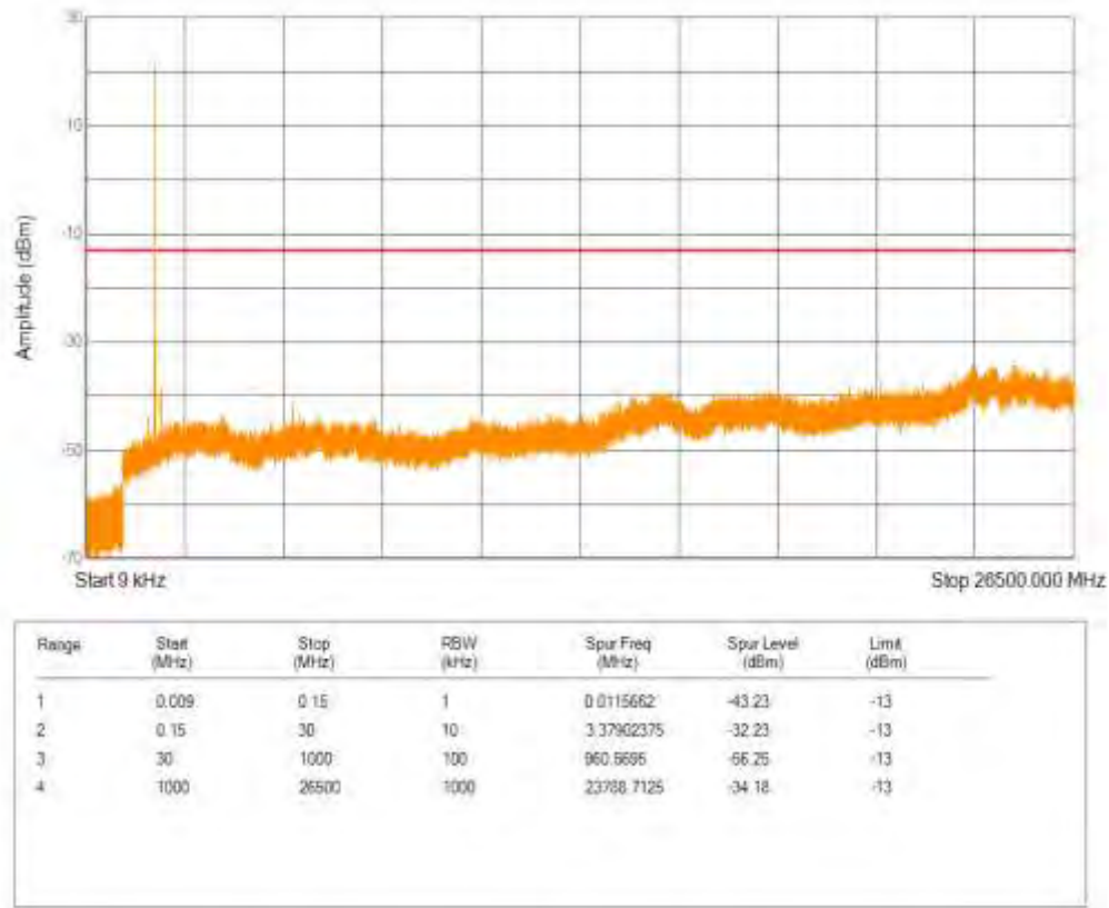
Band25 QPSK BW=20MHz Channel=26365 RB Size=1 Position=#0 NB Index=0
