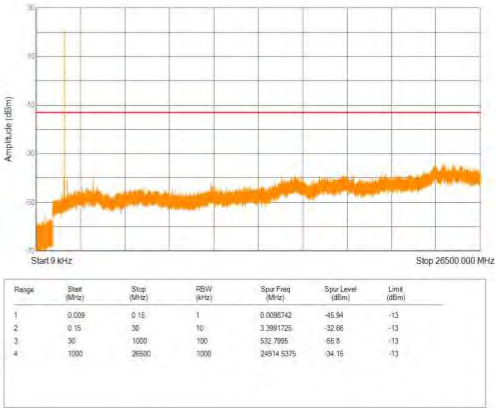
Band66 16QAM BW=3MHz Channel=131987 RB Size=1 Position=#0 NB Index=0
