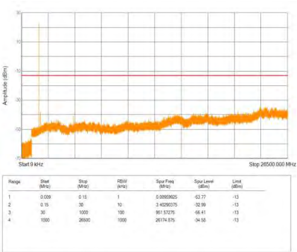
Band4 16QAM BW=20MHz Channel=20175 RB Size=5 Position=#0 NB Index=0
