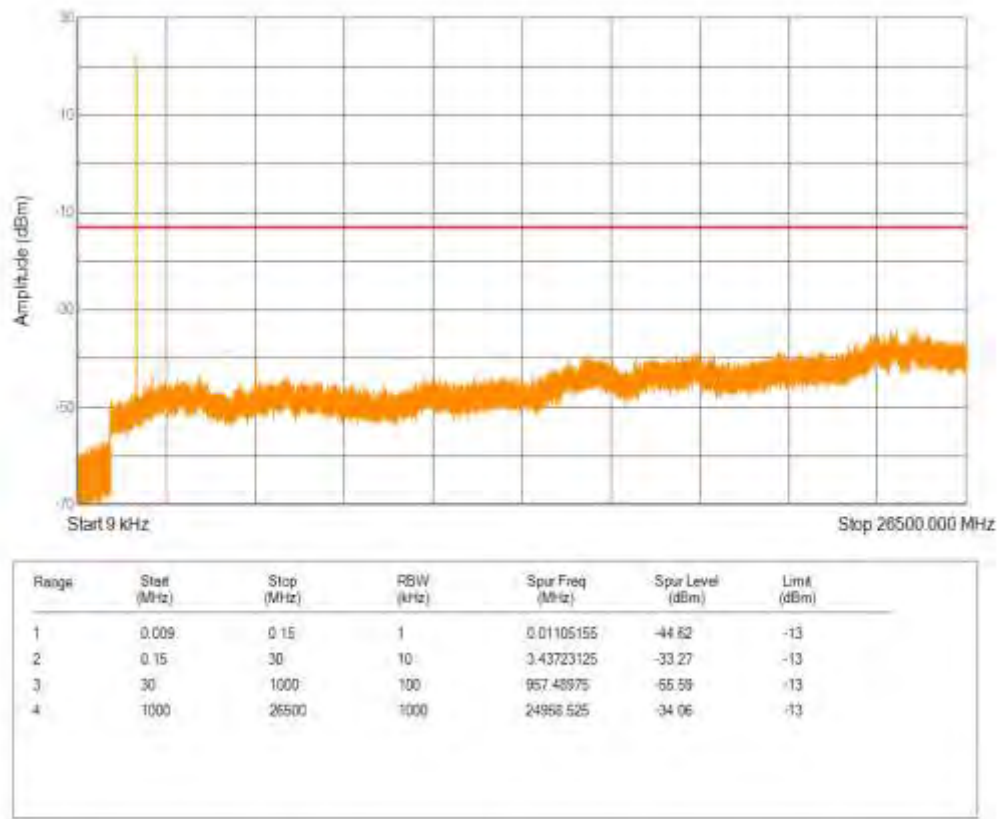
Band66 16QAM BW=5MHz Channel=132647 RB Size=1 Position=#0 NB Index=0
