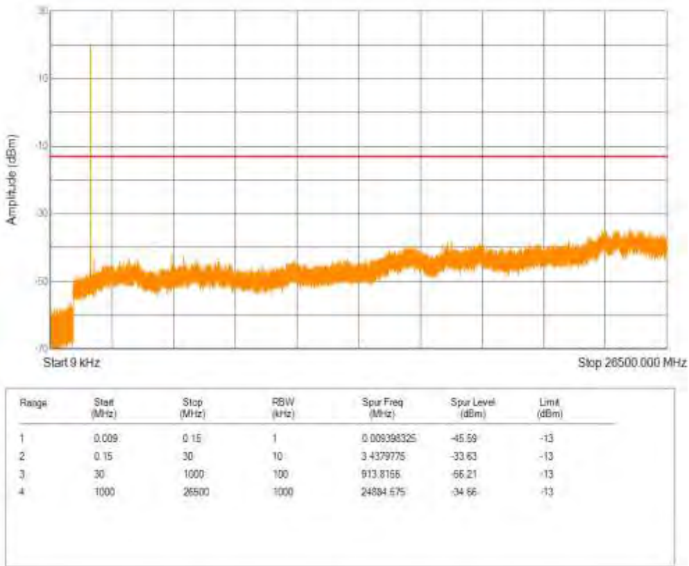
Band66 16QAM BW=3MHz Channel=132322 RB Size=5 Position=#0 NB Index=0
