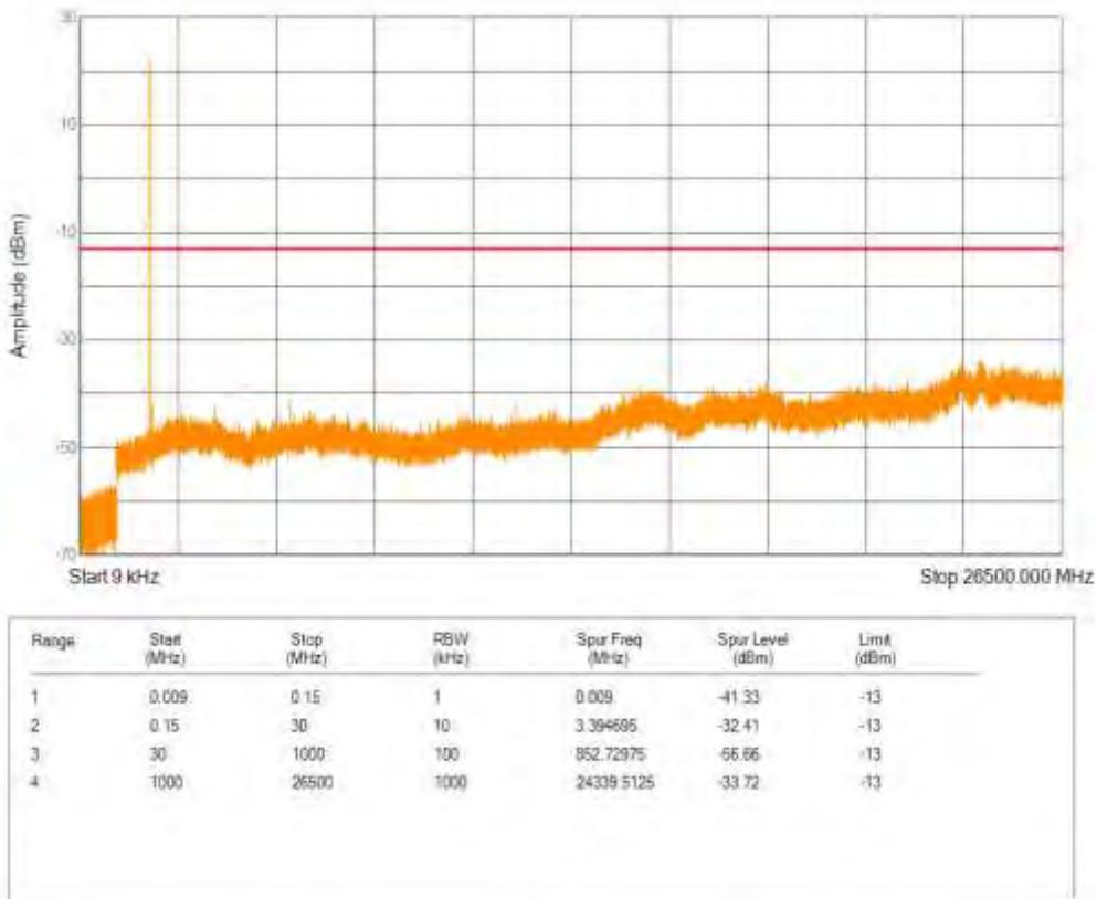
Band26(814-824) QPSK BW=1.4MHz Channel=26697 RB Size=1 Position=#0 NB Index=0
