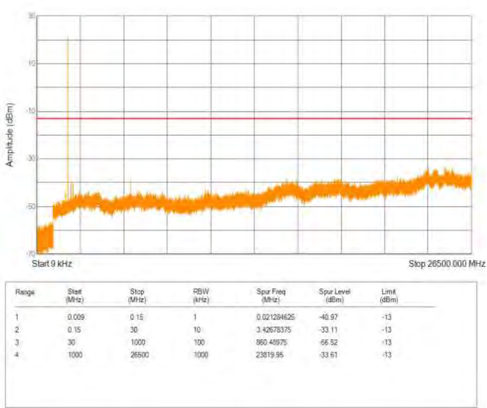
Band25 16QAM BW=10MHz Channel=26640 RB Size=1 Position=#0 NB Index=0
