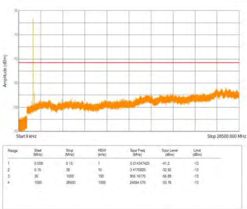
Band66 16QAM BW=1.4MHz Channel=132322 RB Size=5 Position=#0 NB Index=0
