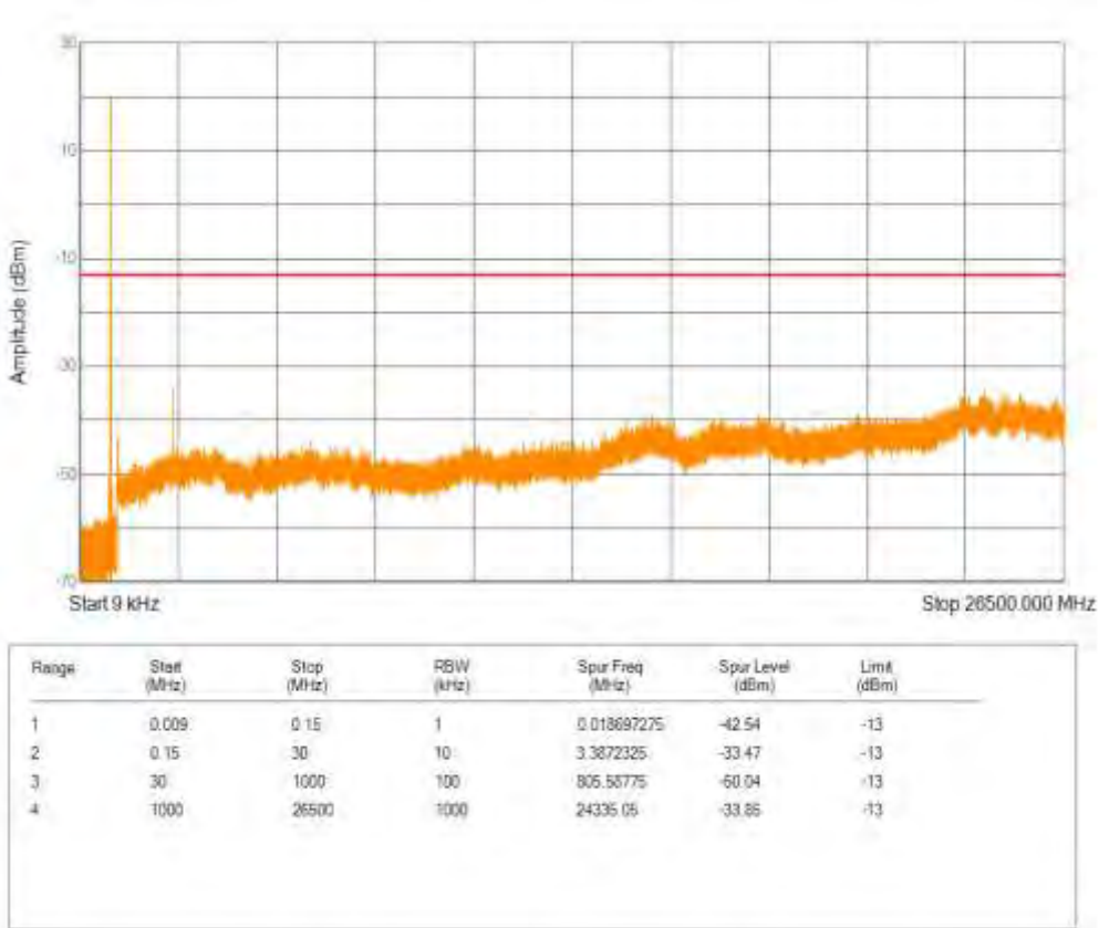
Band26(824-849) 16QAM BW=1.4MHz Channel=26915 RB Size=5 Position=#0 NB Index=0
