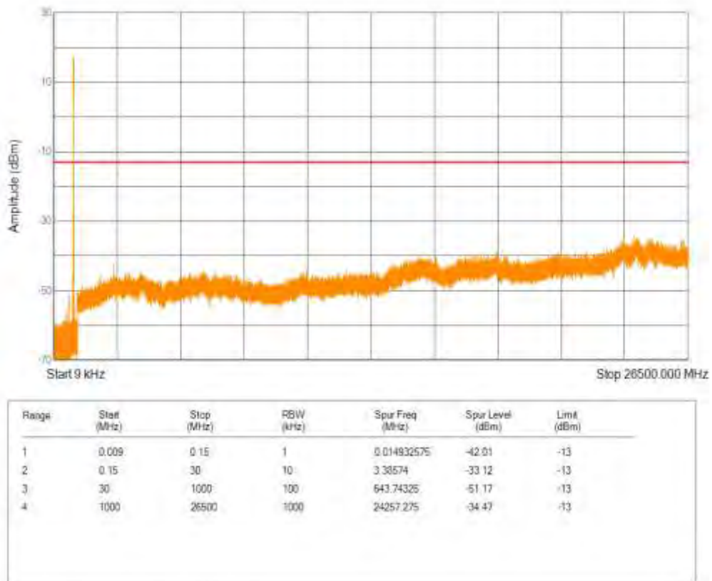
Band26(824-849) QPSK BW=3MHz Channel=27025 RB Size=1 Position=#0 NB Index=0
