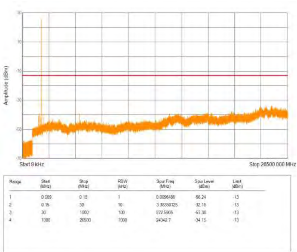
Band2 QPSK BW=20MHz Channel=19100 RB Size=6 Position=#0 NB Index=0
