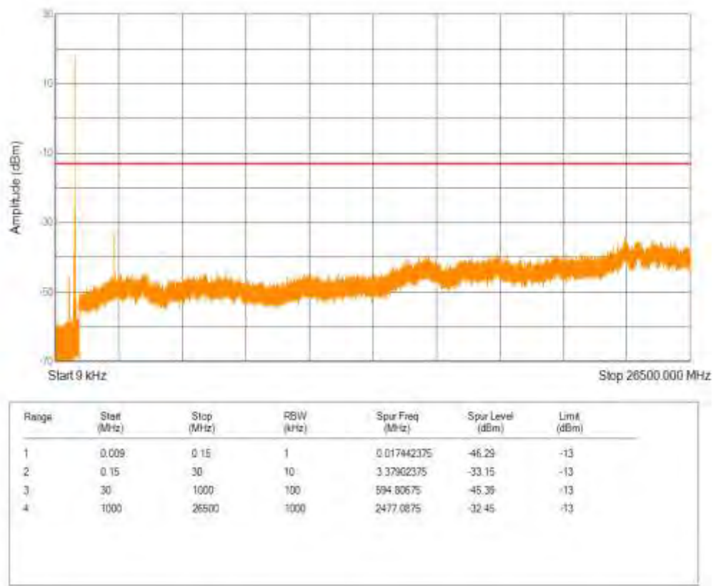
Band26(824-849) 16QAM BW=15MHz Channel=26865 RB Size=1 Position=#0 NB Index=0
