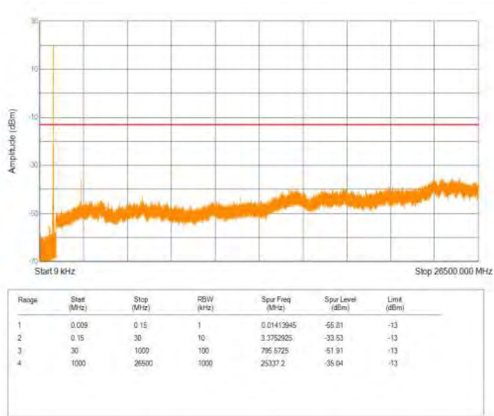
Band5 16QAM BW=5MHz Channel=20525 RB Size=5 Position=#0 NB Index=0
