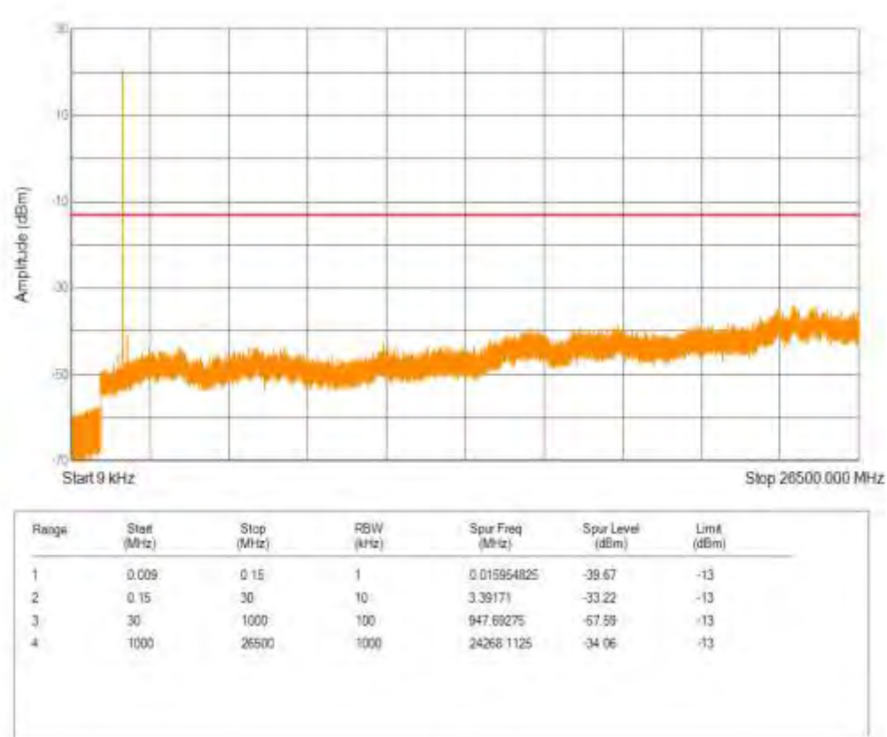
Band66 16QAM BW=3MHz Channel=132322 RB Size=1 Position=#0 NB Index=0
