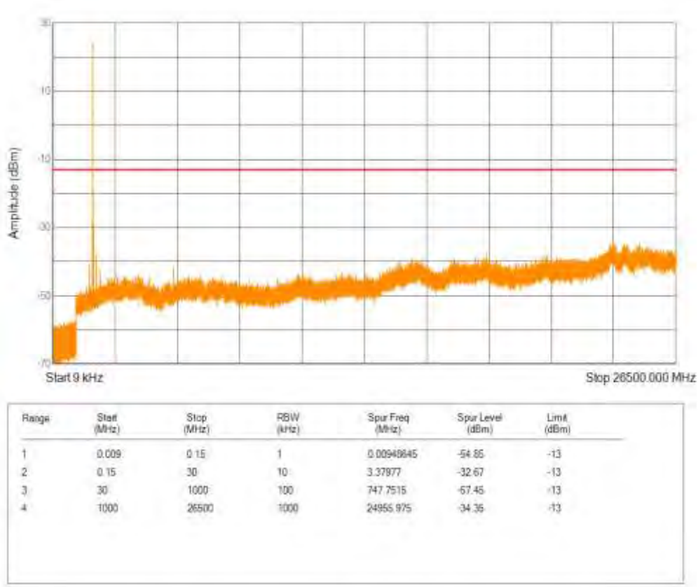
Band4 QPSK BW=15MHz Channel=20175 RB Size=1 Position=#0 NB Index=0
