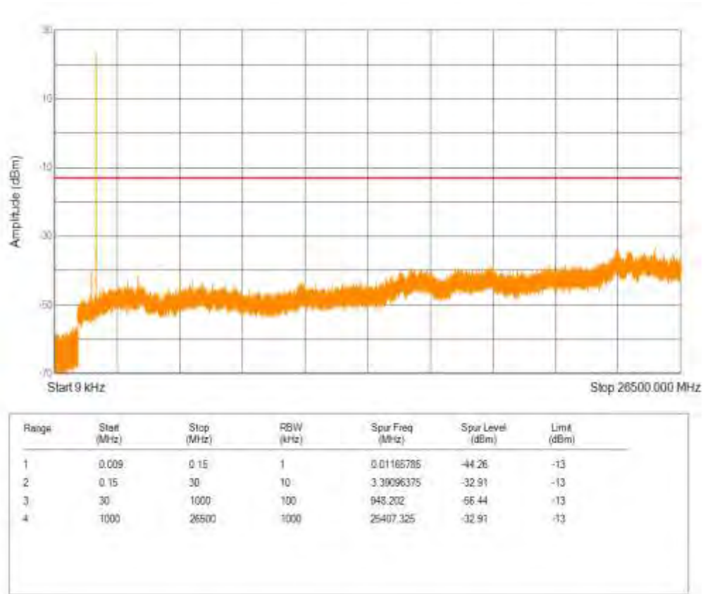
Band66 16QAM BW=5MHz Channel=132647 RB Size=5 Position=#0 NB Index=0
