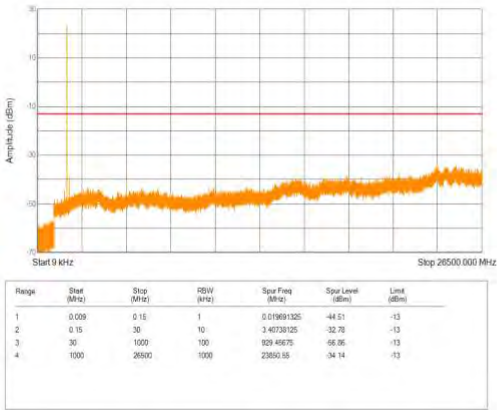
Band66 16QAM BW=10MHz Channel=132622 RB Size=1 Position=#0 NB Index=0
