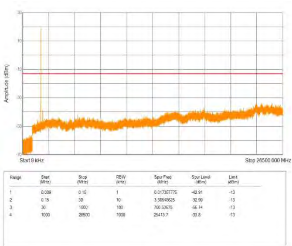
Band25 16QAM BW=15MHz Channel=26365 RB Size=5 Position=#0 NB Index=0
