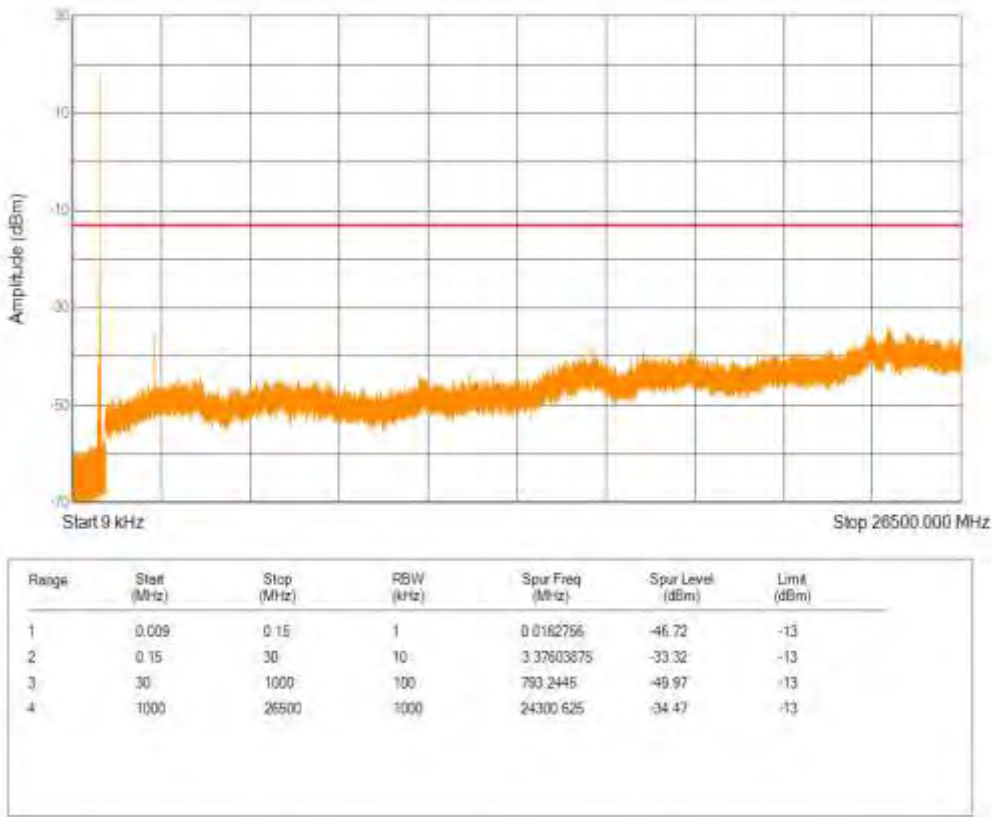
Band26(824-849) QPSK BW=5MHz Channel=26915 RB Size=1 Position=#0 NB Index=0
