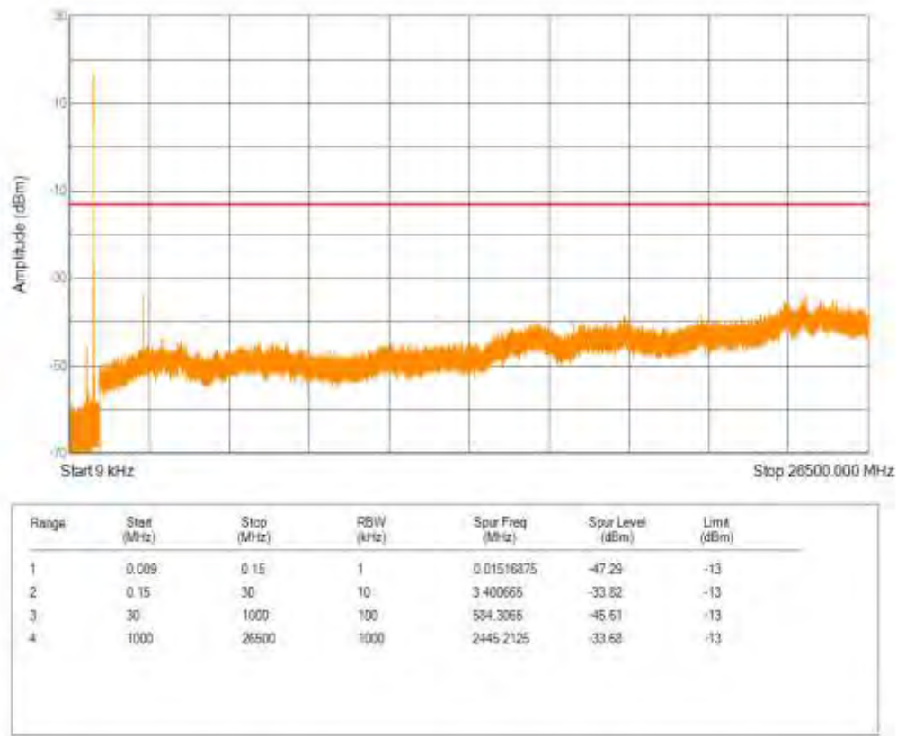
Band26(814-824) QPSK BW=3MHz Channel=26740 RB Size=1 Position=#0 NB Index=0
