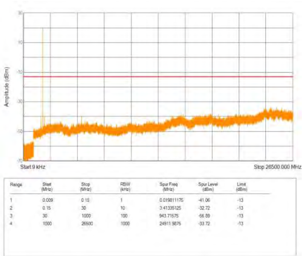
Band25 QPSK BW=3MHz Channel=26675 RB Size=6 Position=#0 NB Index=0
