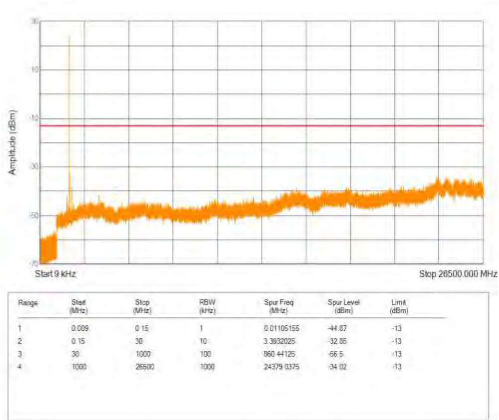
Band66 QPSK BW=20MHz Channel=132572 RB Size=6 Position=#0 NB Index=0
