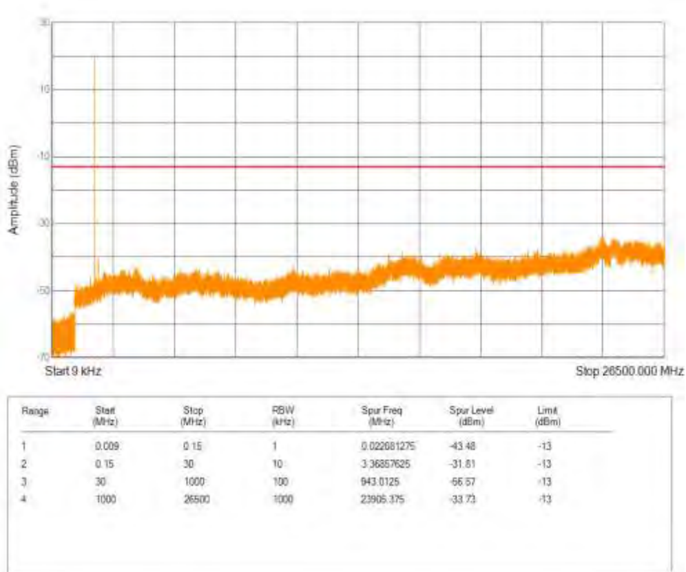
Band25 QPSK BW=1.4MHz Channel=26365 RB Size=1 Position=#0 NB Index=0
