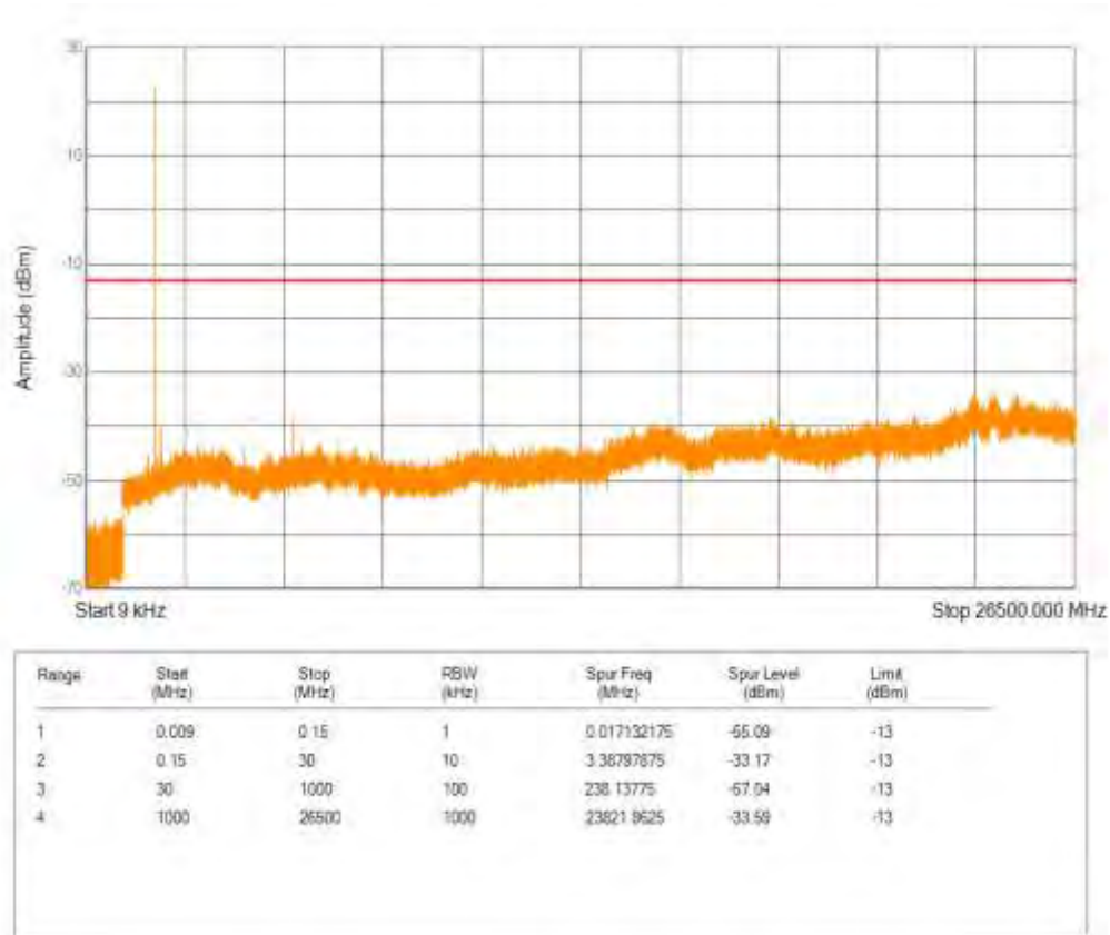
Band2 16QAM BW=3MHz Channel=18615 RB Size=1 Position=#0 NB Index=0
