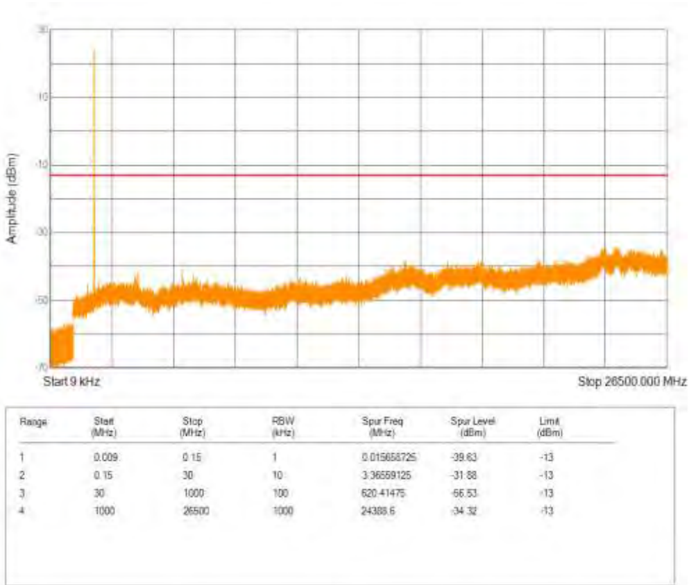
Band25 16QAM BW=20MHz Channel=26590 RB Size=5 Position=#0 NB Index=0
