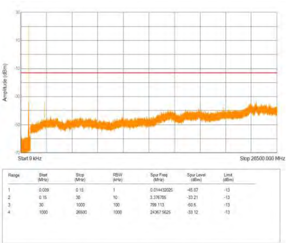
Band26(824-849) QPSK BW=3MHz Channel=26805 RB Size=6 Position=#0 NB Index=0
