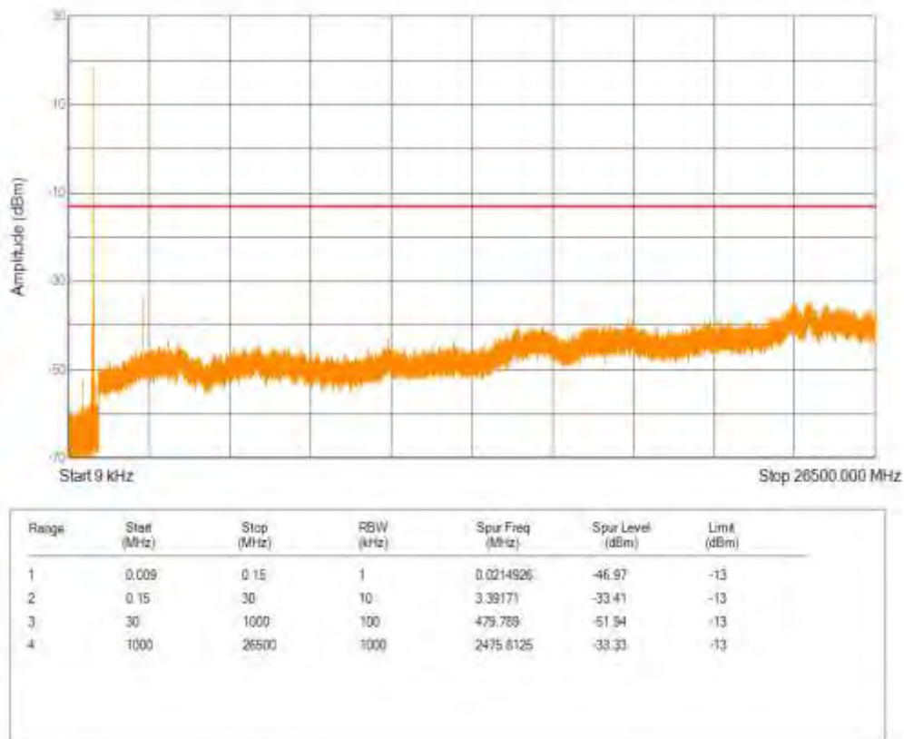
Band26(824-849) QPSK BW=10MHz Channel=26915 RB Size=1 Position=#0 NB Index=0
