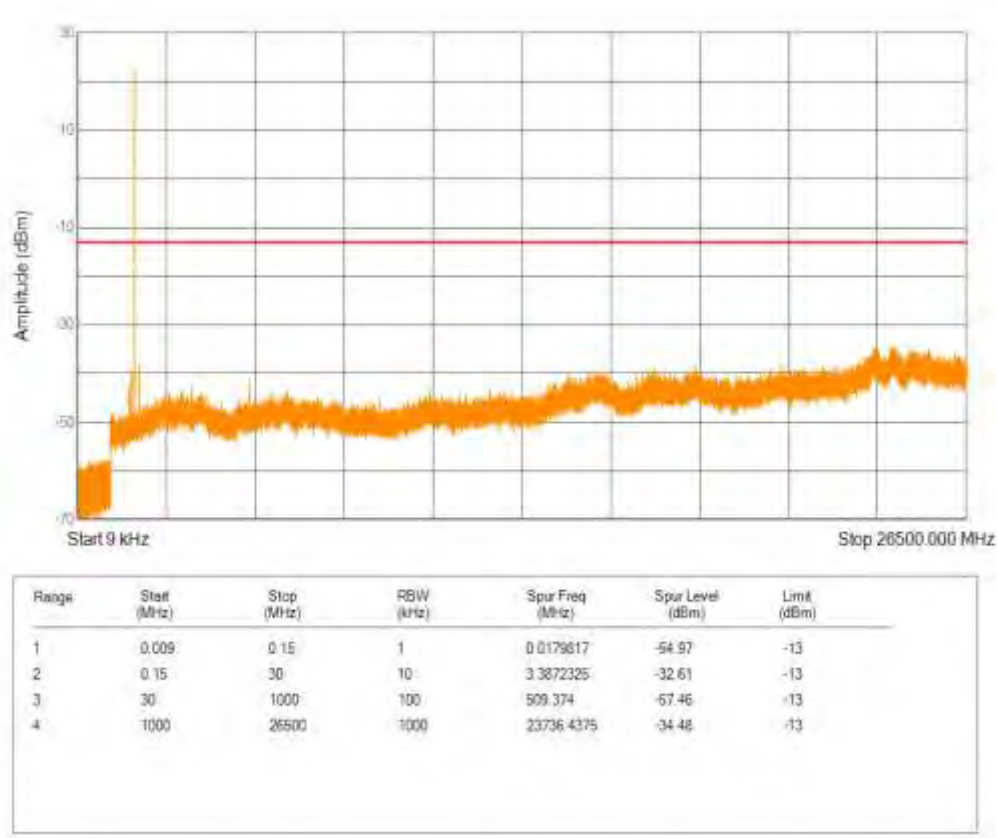
Band4 16QAM BW=15MHz Channel=20025 RB Size=1 Position=#0 NB Index=0
