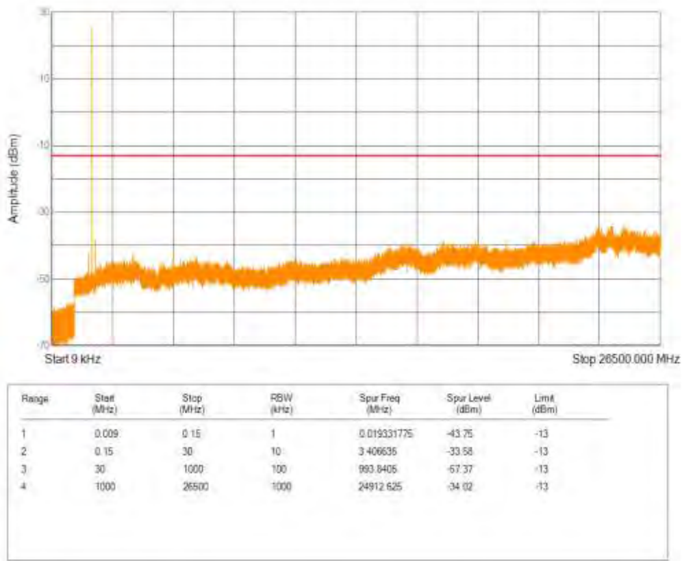
Band66 QPSK BW=20MHz Channel=132072 RB Size=1 Position=#0 NB Index=0
