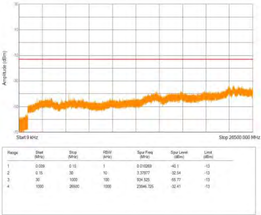
Band25 16QAM BW=10MHz Channel=26365 RB Size=1 Position=#0 NB Index=0
