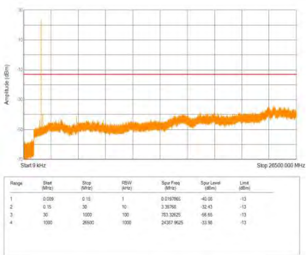
Band66 QPSK BW=15MHz Channel=132322 RB Size=1 Position=#0 NB Index=0
