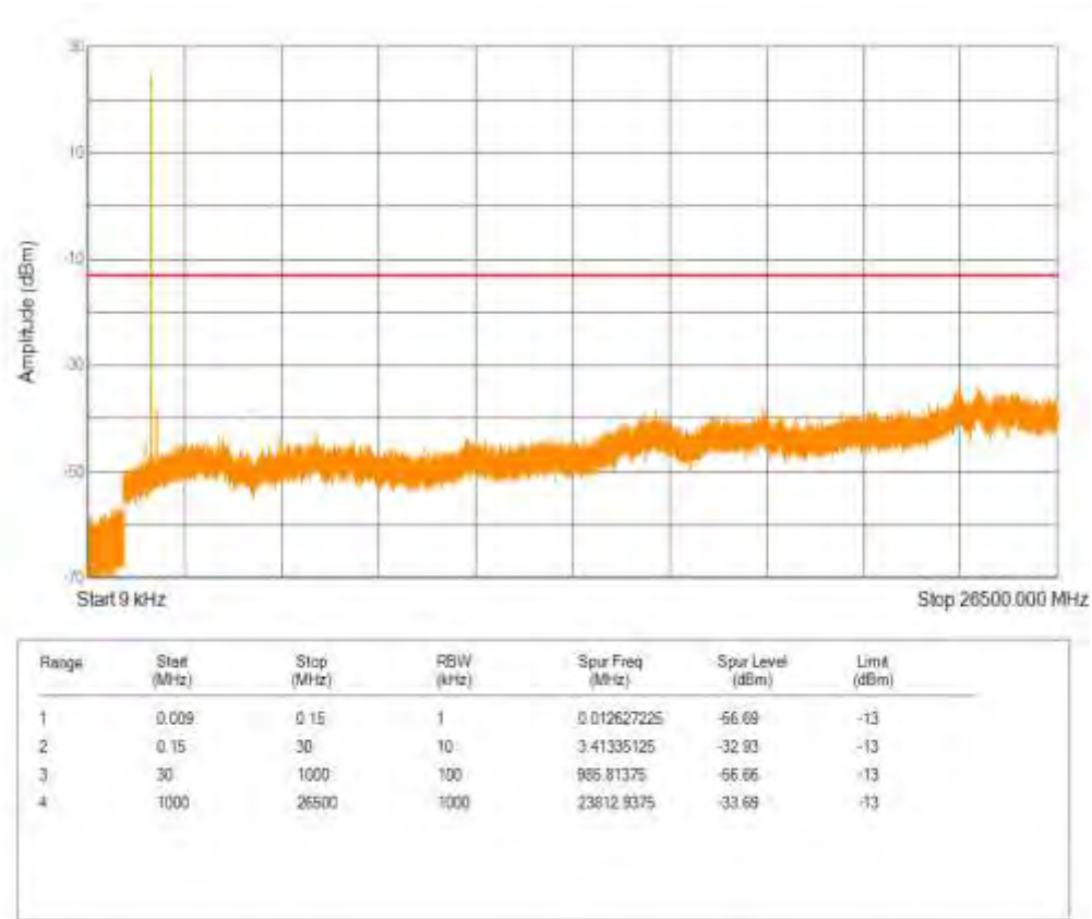
Band4 QPSK BW=10MHz Channel=20350 RB Size=6 Position=#0 NB Index=0
