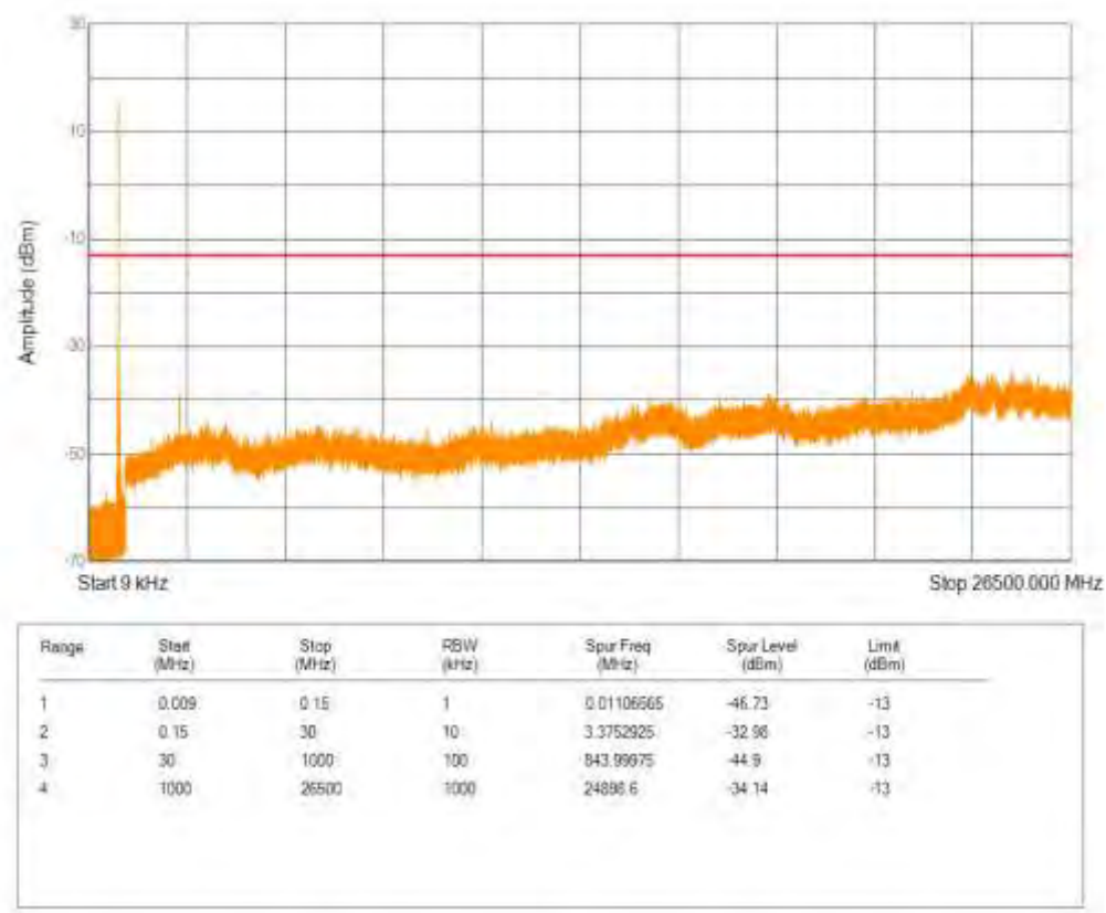
Band26(814-824) 16QAM BW=3MHz Channel=26775 RB Size=1 Position=#0 NB Index=0
