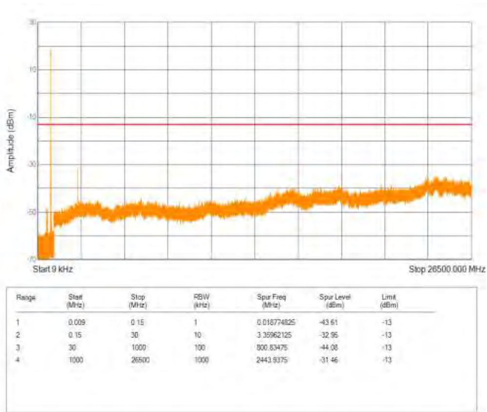
Band26(814-824) 16QAM BW=3MHz Channel=26705 RB Size=5 Position=#0 NB Index=0
