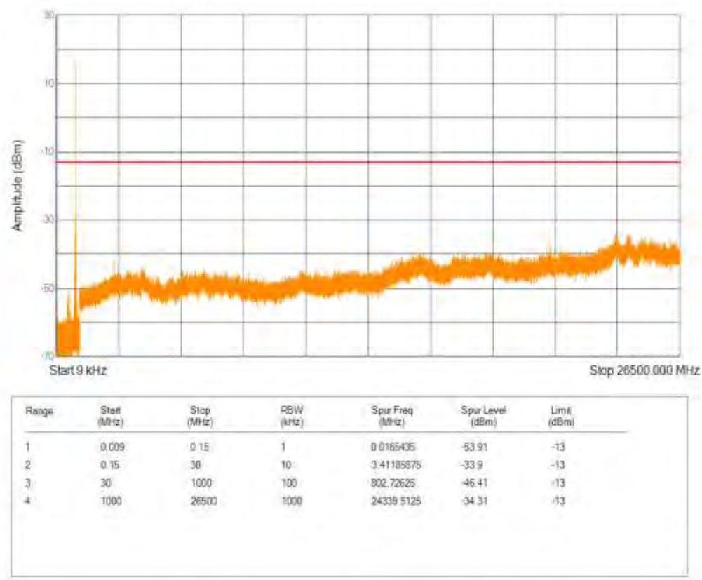
Band5 16QAM BW=3MHz Channel=20415 RB Size=1 Position=#0 NB Index=0
