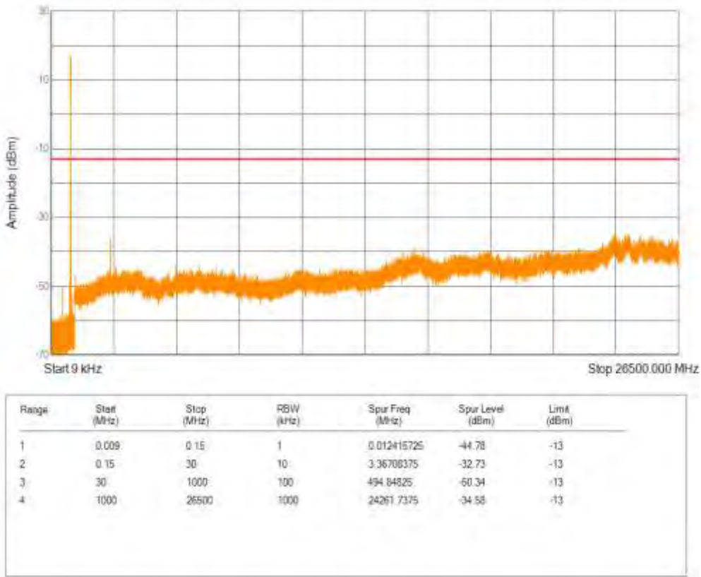
Band26(824-849) 16QAM BW=10MHz Channel=26990 RB Size=1 Position=#0 NB Index=0
