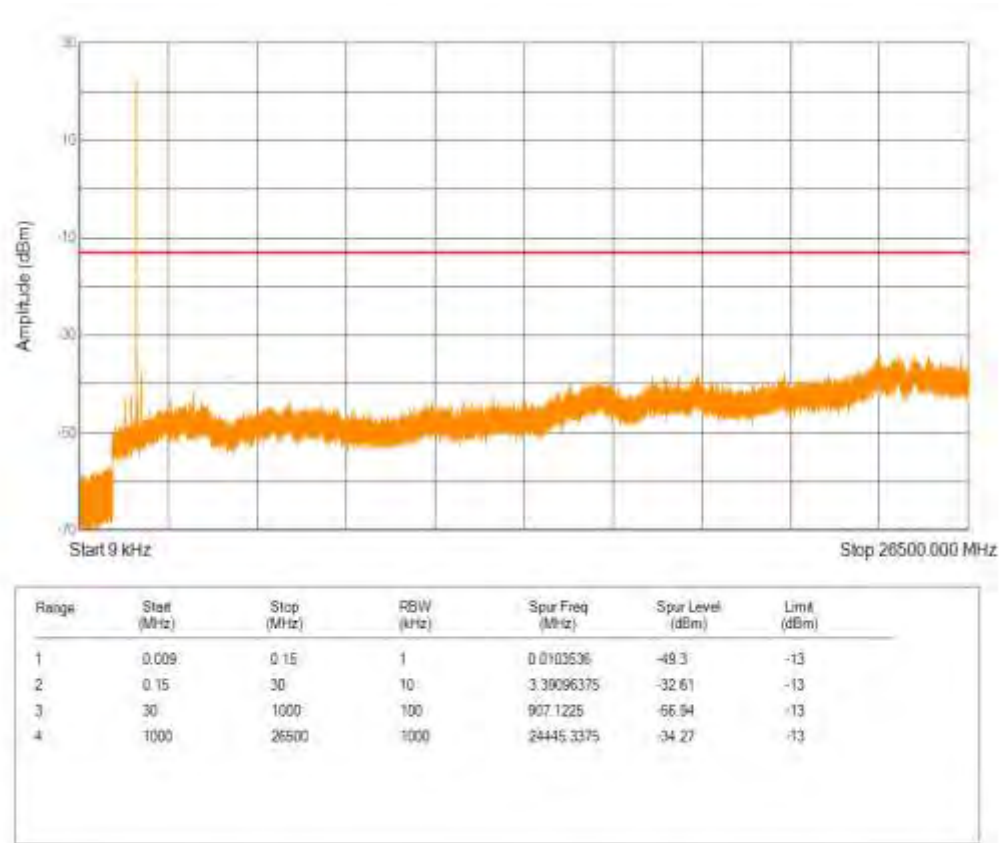
Band4 16QAM BW=1.4MHz Channel=19957 RB Size=5 Position=#0 NB Index=0
