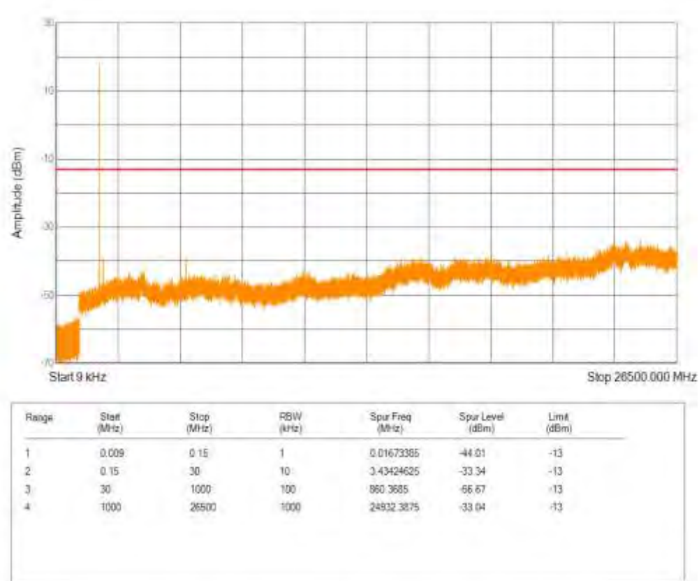
Band25 QPSK BW=3MHz Channel=26365 RB Size=1 Position=#0 NB Index=0
