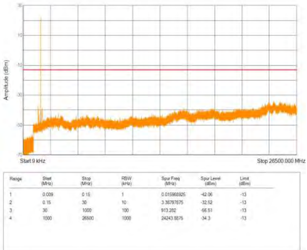
Band66 QPSK BW=20MHz Channel=132322 RB Size=1 Position=#0 NB Index=0
