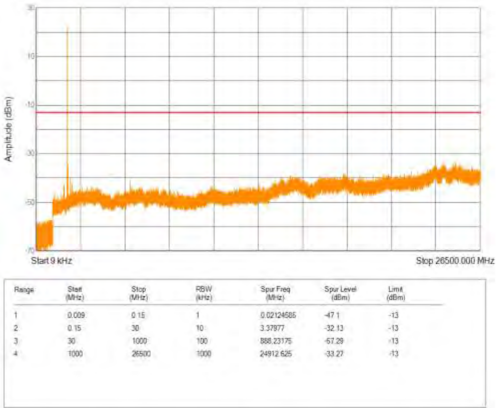
Band25 16QAM BW=20MHz Channel=26365 RB Size=1 Position=#0 NB Index=0
