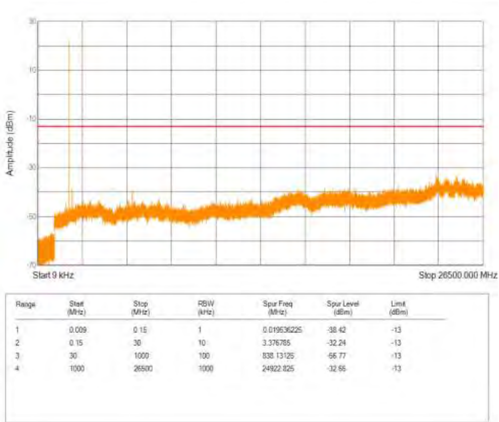
Band25 QPSK BW=5MHz Channel=26365 RB Size=6 Position=#0 NB Index=0
