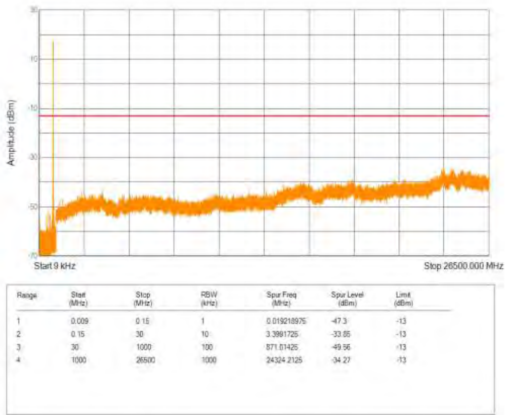
Band26(824-849) QPSK BW=10MHz Channel=26840 RB Size=1 Position=#0 NB Index=0
