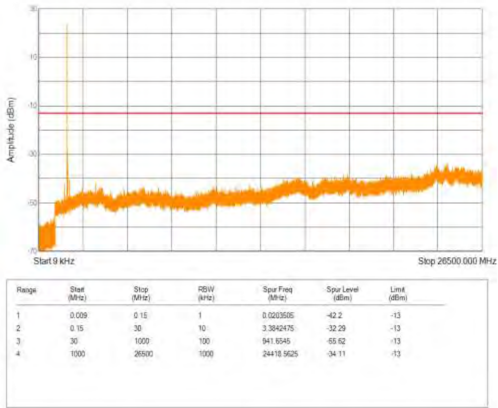
Band66 16QAM BW=15MHz Channel=132047 RB Size=1 Position=#0 NB Index=0
