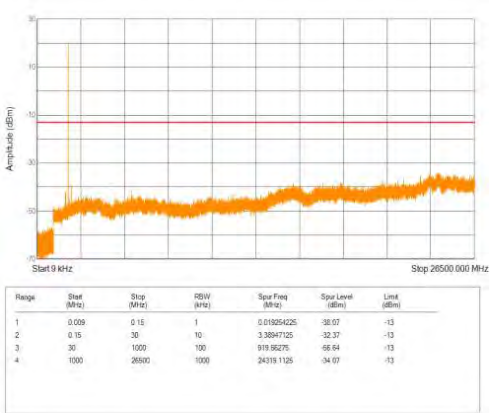
Band25 QPSK BW=10MHz Channel=26640 RB Size=6 Position=#0 NB Index=0
