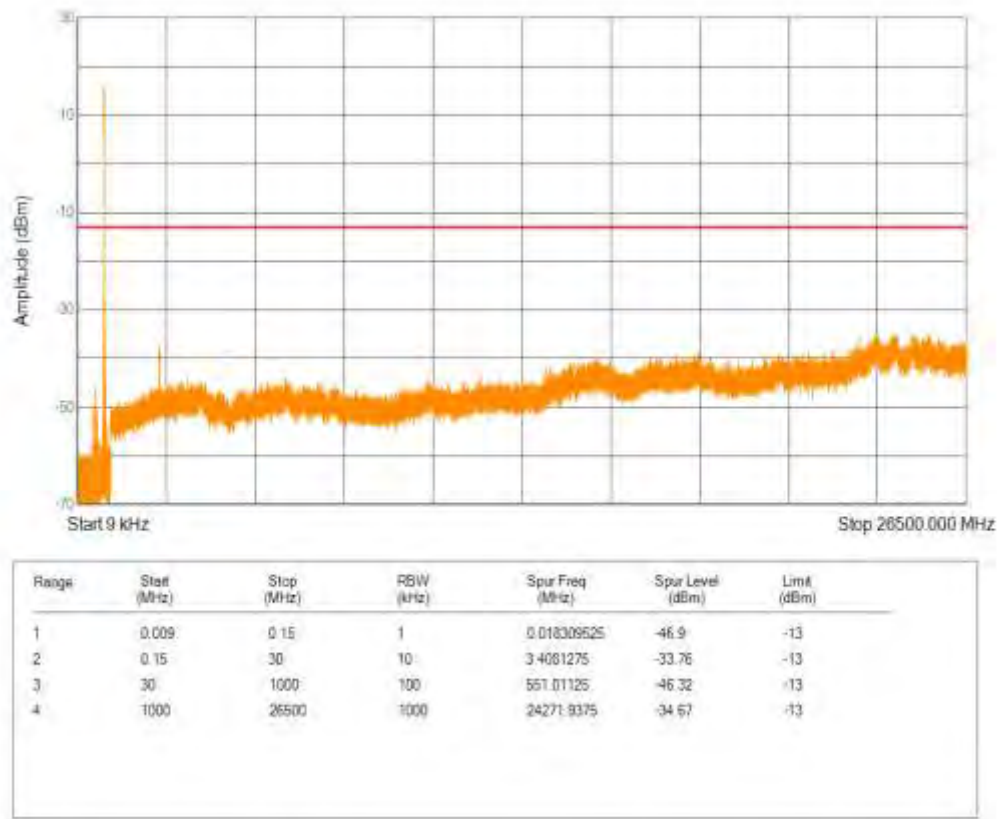
Band26(814-824) 16QAM BW=5MHz Channel=26765 RB Size=1 Position=#0 NB Index=0
