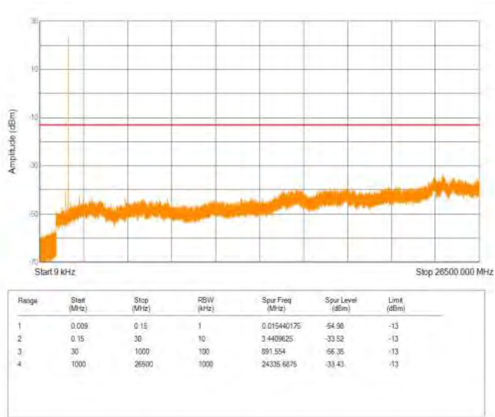
Band4 QPSK BW=15MHz Channel=20175 RB Size=6 Position=#0 NB Index=0
