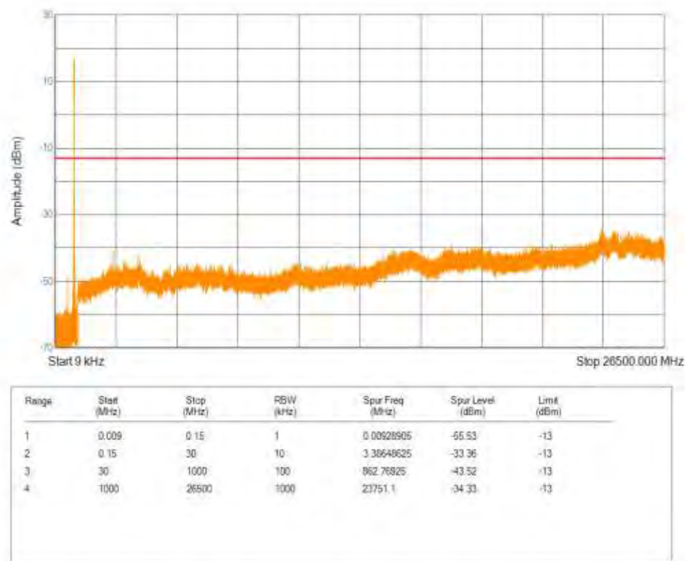
Band5 16QAM BW=3MHz Channel=20635 RB Size=1 Position=#0 NB Index=0
