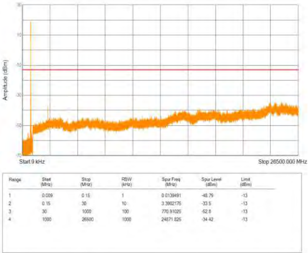
Band26(814-824) 16QAM BW=10MHz Channel=26740 RB Size=1 Position=#0 NB Index=0
