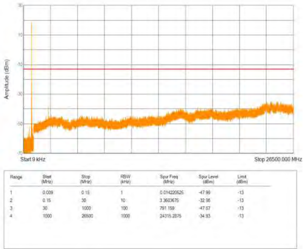
Band26(814-824) 16QAM BW=5MHz Channel=26715 RB Size=1 Position=#0 NB Index=0
