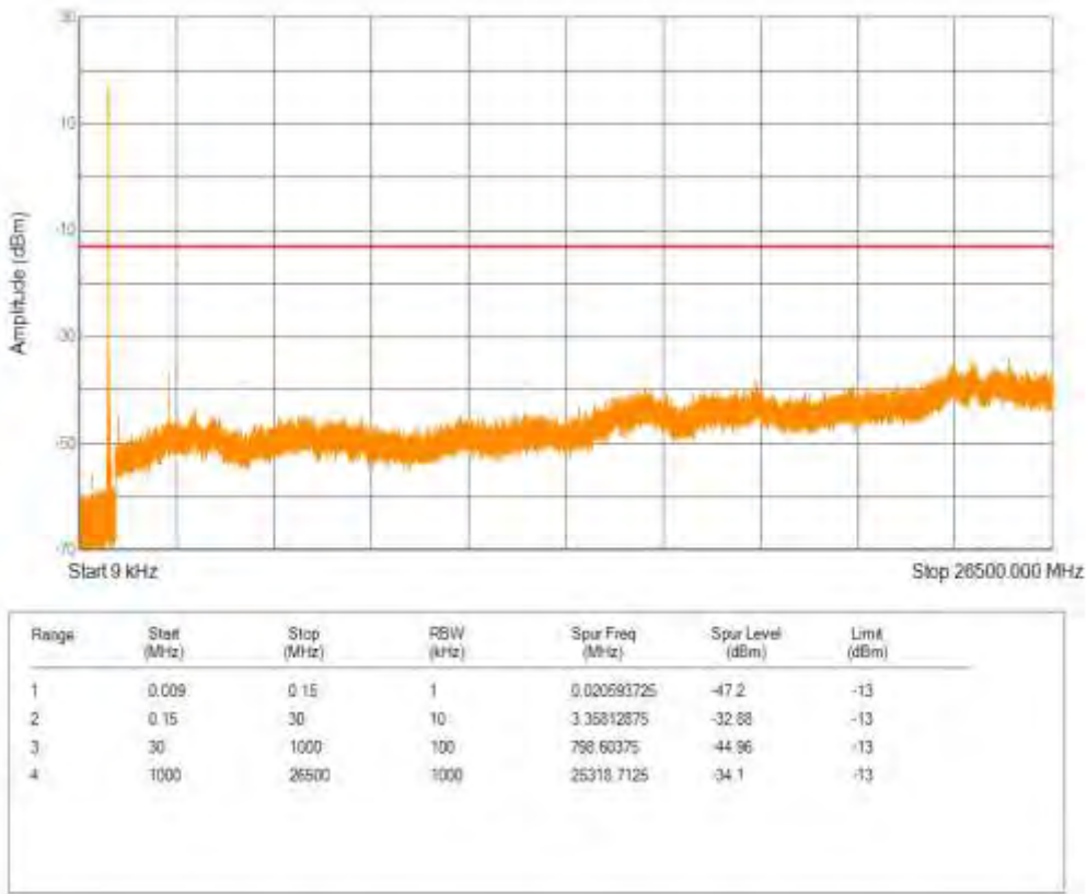
Band26(814-824) 16QAM BW=3MHz Channel=26705 RB Size=1 Position=#0 NB Index=0
