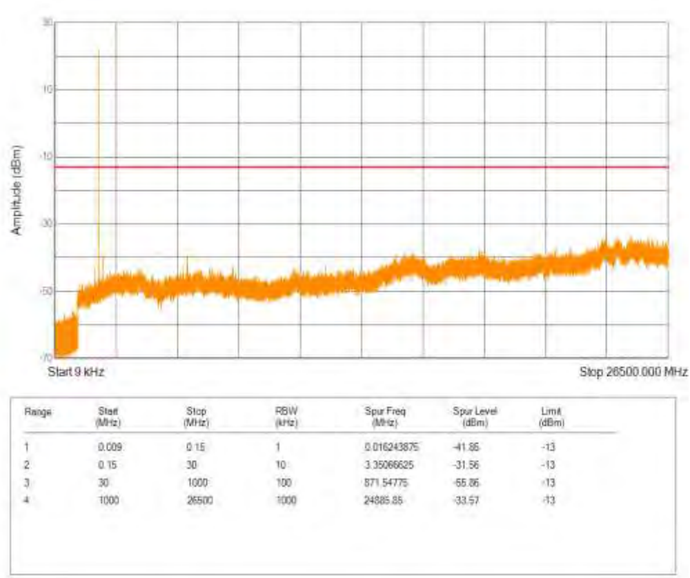
Band25 16QAM BW=5MHz Channel=26665 RB Size=1 Position=#0 NB Index=0
