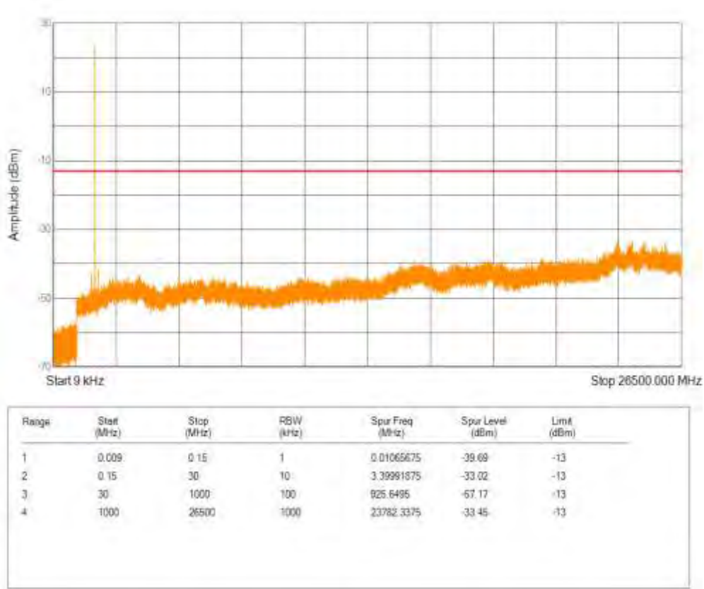
Band66 16QAM BW=15MHz Channel=132597 RB Size=1 Position=#0 NB Index=0
