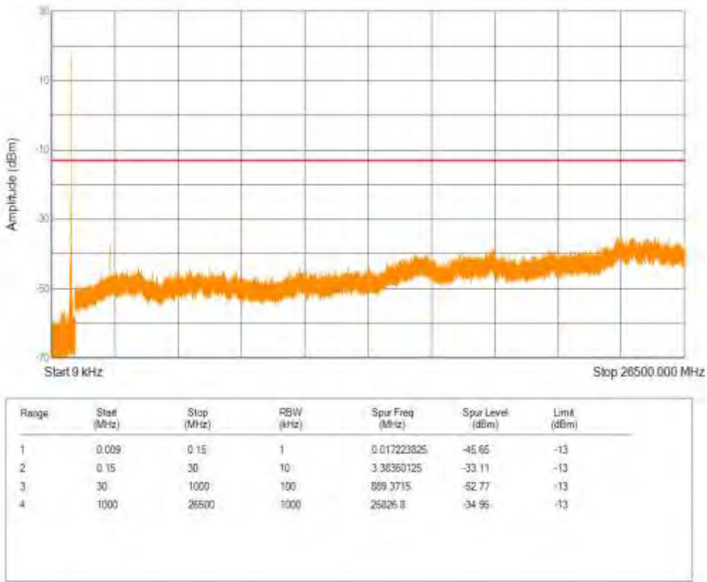
Band26(824-849) 16QAM BW=10MHz Channel=26840 RB Size=1 Position=#0 NB Index=0
