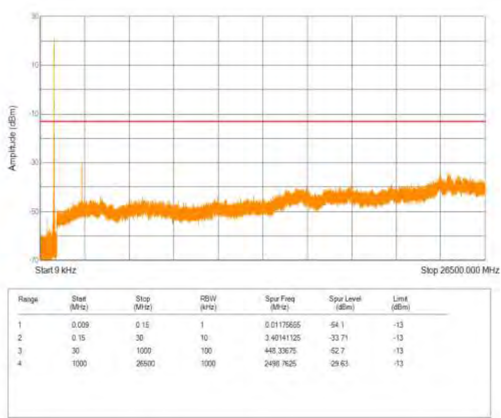
Band5 QPSK BW=10MHz Channel=20600 RB Size=1 Position=#0 NB Index=0
