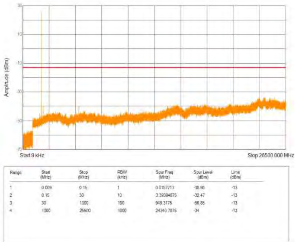
Band25 16QAM BW=3MHz Channel=26365 RB Size=5 Position=#0 NB Index=0
