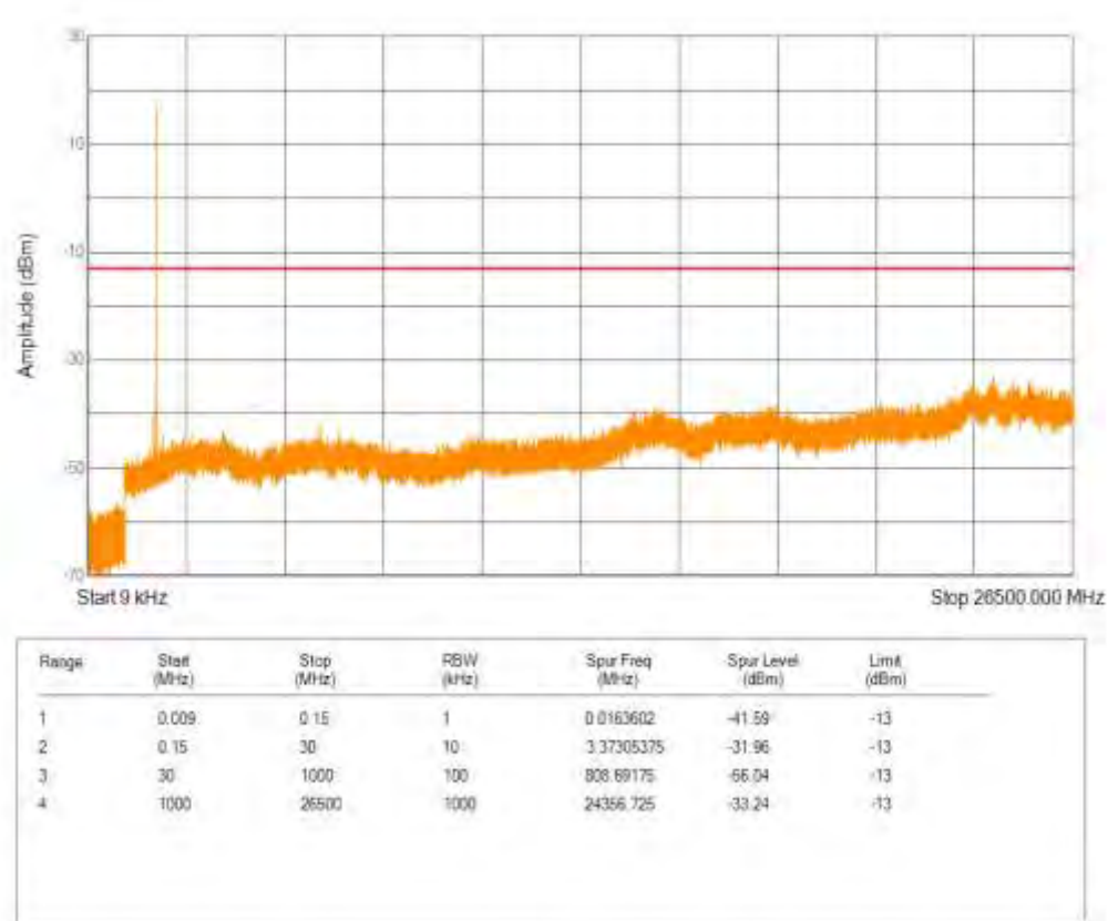
Band25 16QAM BW=1.4MHz Channel=26047 RB Size=1 Position=#0 NB Index=0
