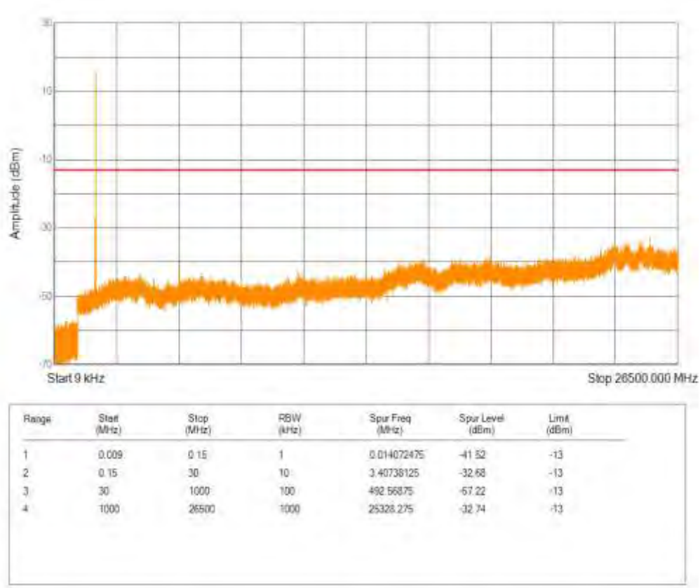
Band66 QPSK BW=3MHz Channel=131987 RB Size=1 Position=#0 NB Index=0
