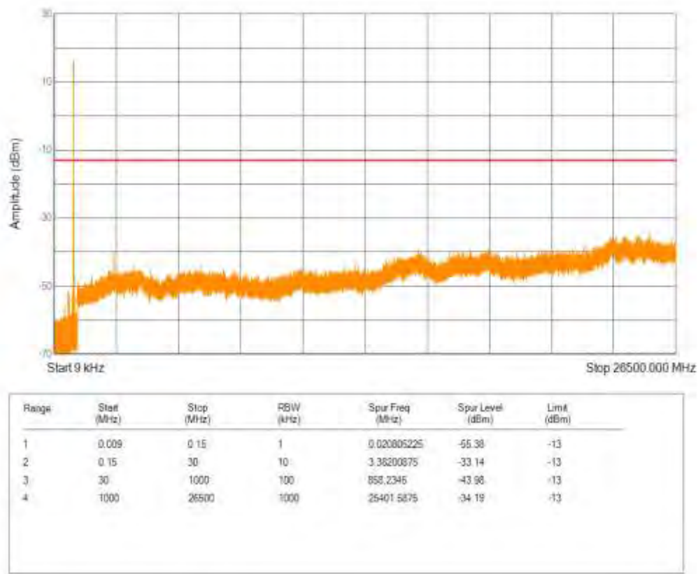
Band5 16QAM BW=1.4MHz Channel=20643 RB Size=1 Position=#0 NB Index=0
