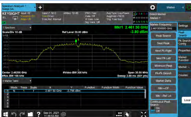
802.11b HIGH CHANNEL, Carrier level
