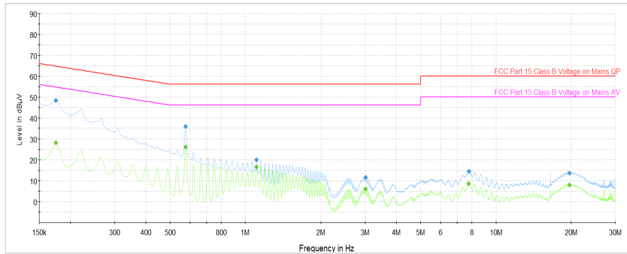
Plot 7-40. AC Line-Conducted Test Plot (N, GFSK – Ch.0, with host PC and USB-C cable)
