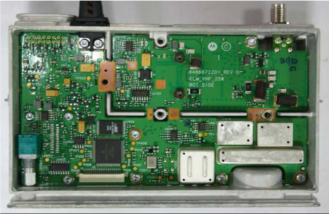
Figure 9-5: Top View of PCB placed in chassis.
