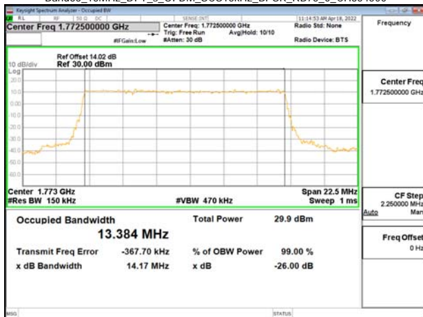
Band66_15MHz_DFT_s_OFDM_SCS15kHz_BPSK_RB75_0_CH354500
