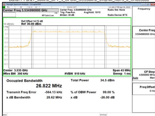
Band77-Part27_30MHz_DFT_s_OFDM_SCS30kHz_64QAM_RB75_0_CH635666
