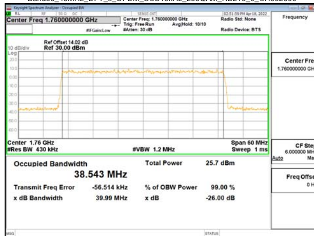
Band66_40MHz_DFT_s_OFDM_SCS15kHz_256QAM_RB216_0_CH352000
