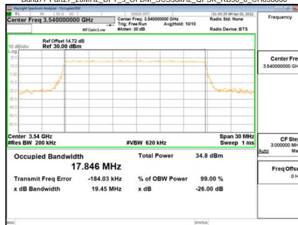
Band77-Part27_20MHz_DFT_s_OFDM_SCS30kHz_QPSK_RB50_0_CH636000
