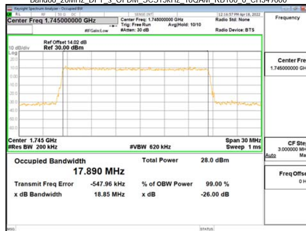
Band66_20MHz_DFT_s_OFDM_SCS15kHz_16QAM_RB100_0_CH354000
