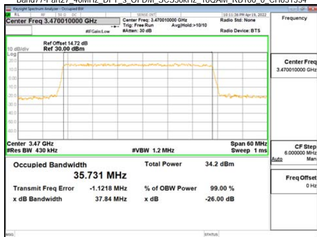
Band77-Part27_40MHz_DFT_s_OFDM_SCS30kHz_16QAM_RB100_0_CH633334
