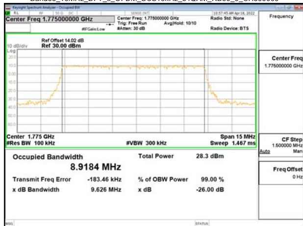
Band66_10MHz_DFT_s_OFDM_SCS15kHz_64QAM_RB50_0_CH355000
