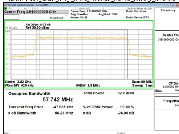
Band77-Part27_60MHz_DFT_s_OFDM_SCS30kHz_256QAM_RB162_0_CH634666
