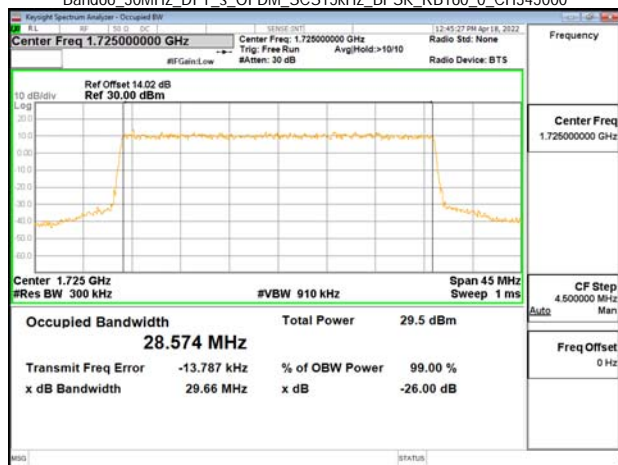
Band66_30MHz_DFT_s_OFDM_SCS15kHz_BPSK_RB160_0_CH349000
