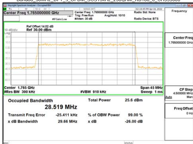
Band66_30MHz_DFT_s_OFDM_SCS15kHz_256QAM_RB160_0_CH353000
