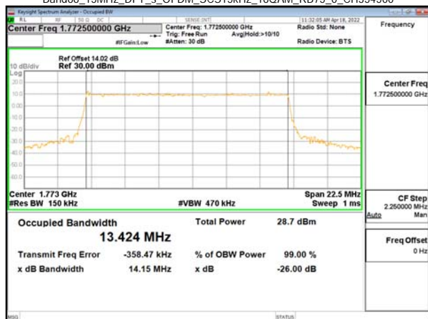
Band66_15MHz_DFT_s_OFDM_SCS15kHz_16QAM_RB75_0_CH354500
