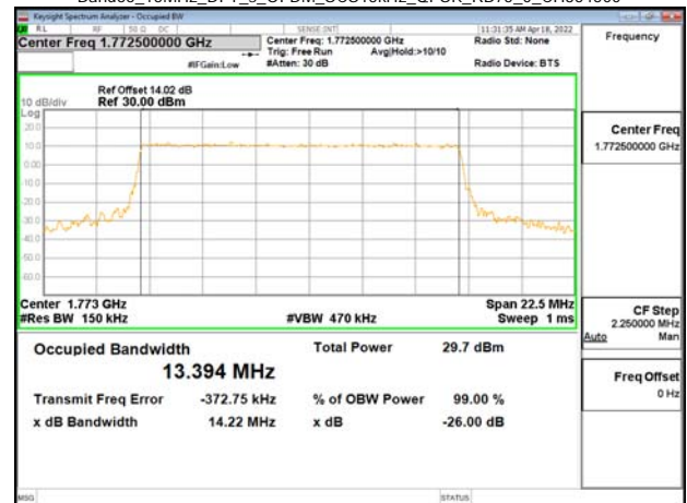
Band66_15MHz_DFT_s_OFDM_SCS15kHz_QPSK_RB75_0_CH354500
