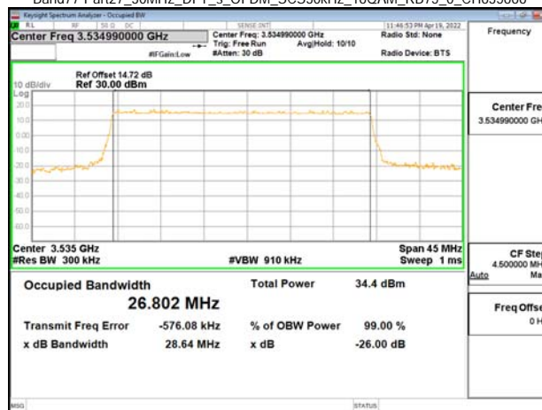
Band77-Part27_30MHz_DFT_s_OFDM_SCS30kHz_16QAM_RB75_0_CH635666
