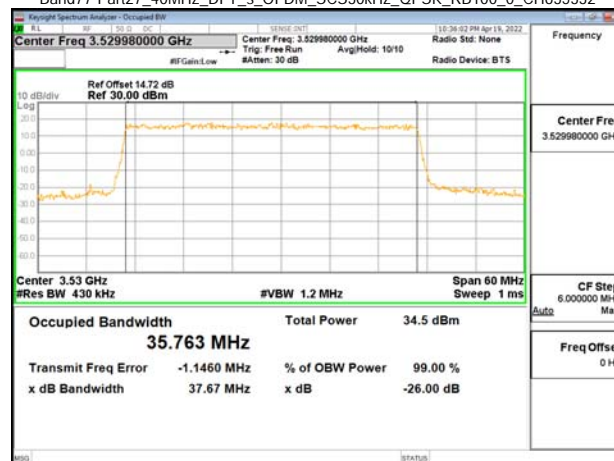
Band77-Part27_40MHz_DFT_s_OFDM_SCS30kHz_QPSK_RB100_0_CH635332
