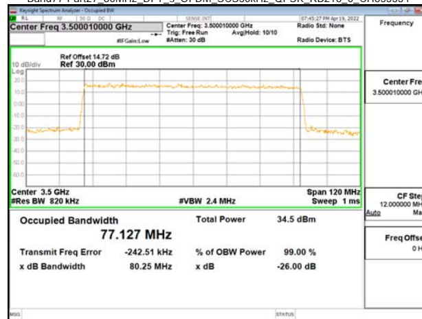
Band77-Part27_80MHz_DFT_s_OFDM_SCS30kHz_QPSK_RB216_0_CH634000
