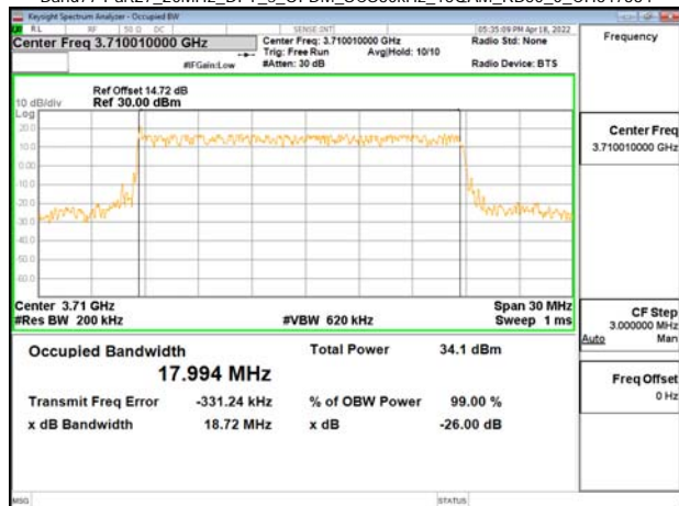
Band77-Part27_20MHz_DFT_s_OFDM_SCS30kHz_16QAM_RB50_0_CH647334
