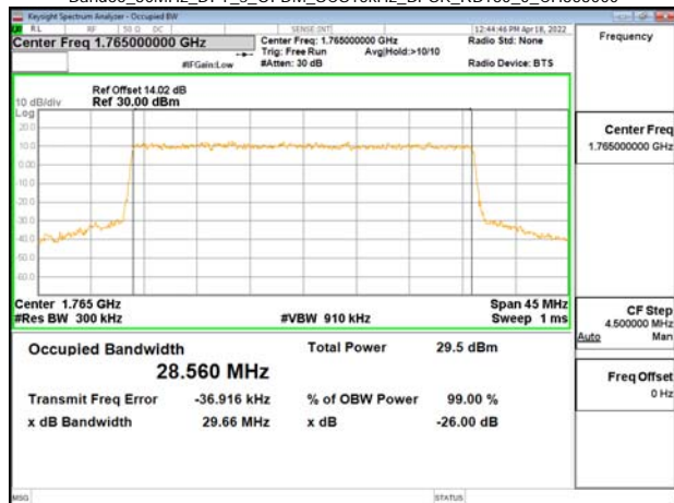
Band66_30MHz_DFT_s_OFDM_SCS15kHz_BPSK_RB160_0_CH353000
