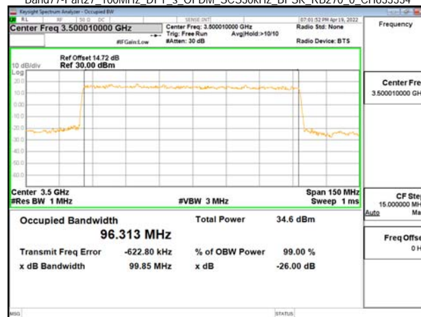
Band77-Part27_100MHz_DFT_s_OFDM_SCS30kHz_QPSK_RB270_0_CH633334
