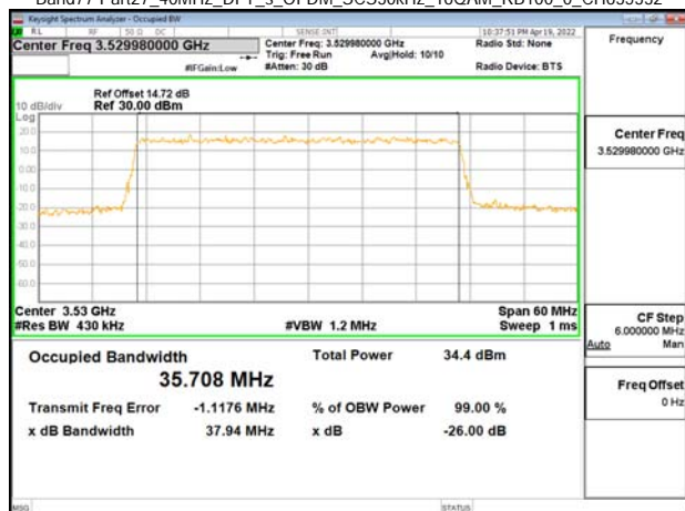
Band77-Part27_40MHz_DFT_s_OFDM_SCS30kHz_16QAM_RB100_0_CH635332
