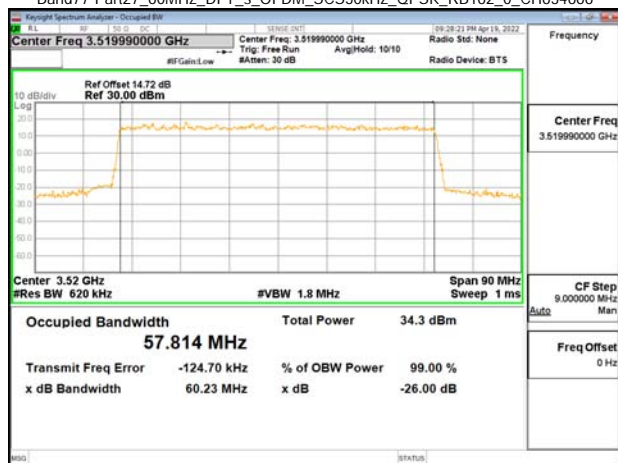
Band77-Part27_60MHz_DFT_s_OFDM_SCS30kHz_QPSK_RB162_0_CH634666
