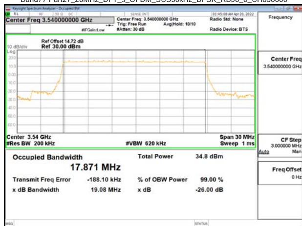
Band77-Part27_20MHz_DFT_s_OFDM_SCS30kHz_BPSK_RB50_0_CH636000
