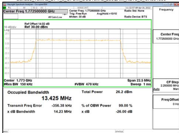
Band66_15MHz_DFT_s_OFDM_SCS15kHz_256QAM_RB75_0_CH354500
