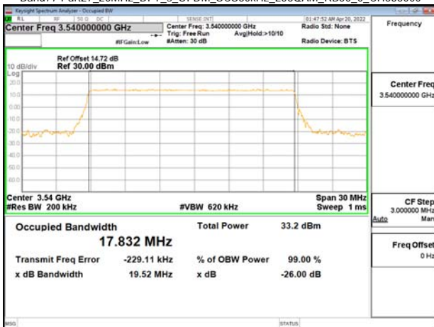
Band77-Part27_20MHz_DFT_s_OFDM_SCS30kHz_256QAM_RB50_0_CH636000
