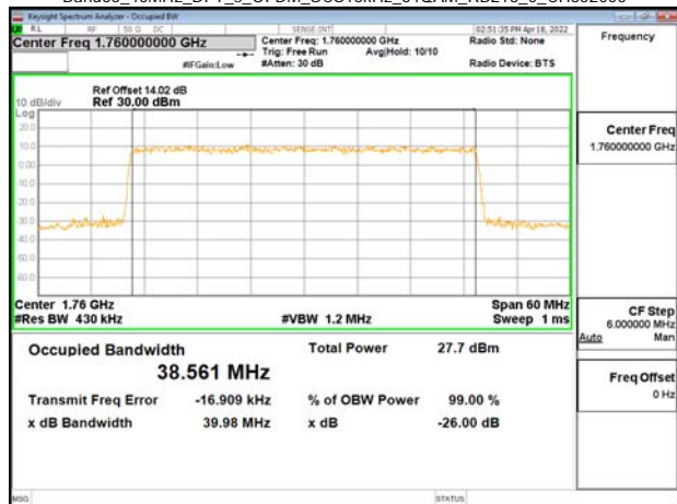
Band66_40MHz_DFT_s_OFDM_SCS15kHz_64QAM_RB216_0_CH352000
