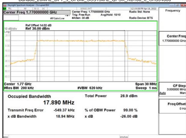
Band66_20MHz_DFT_s_OFDM_SCS15kHz_QPSK_RB100_0_CH354000
