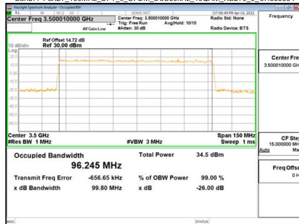
Band77-Part27_100MHz_DFT_s_OFDM_SCS30kHz_16QAM_RB270_0_CH633334
