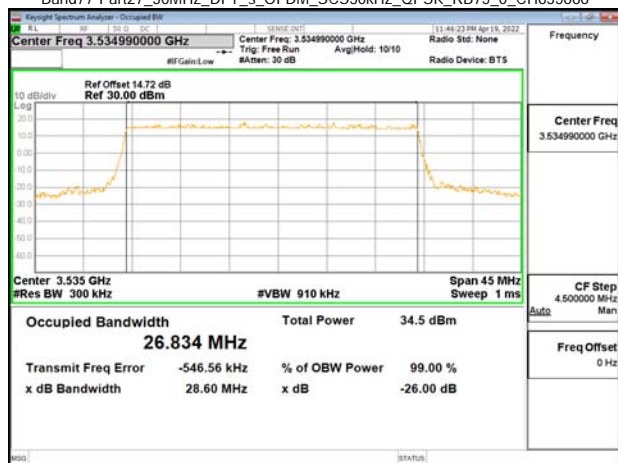
Band77-Part27_30MHz_DFT_s_OFDM_SCS30kHz_QPSK_RB75_0_CH635666
