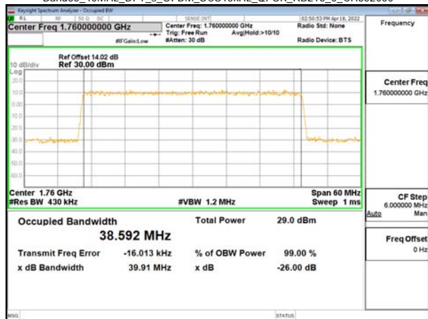
Band66_40MHz_DFT_s_OFDM_SCS15kHz_QPSK_RB216_0_CH352000
