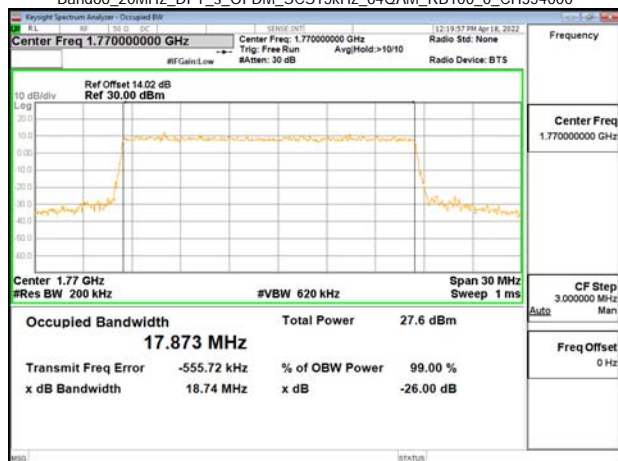
Band66_20MHz_DFT_s_OFDM_SCS15kHz_64QAM_RB100_0_CH354000
