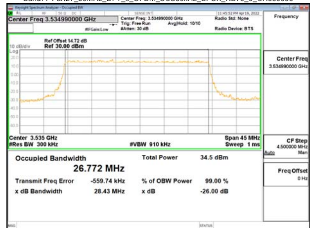
Band77-Part27_30MHz_DFT_s_OFDM_SCS30kHz_BPSK_RB75_0_CH635666
