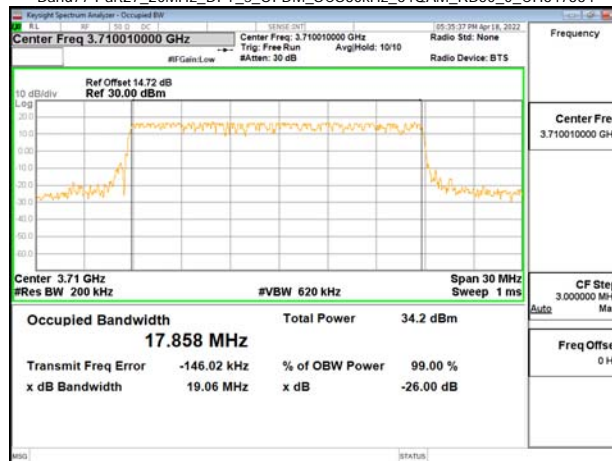
Band77-Part27_20MHz_DFT_s_OFDM_SCS30kHz_64QAM_RB50_0_CH647334
