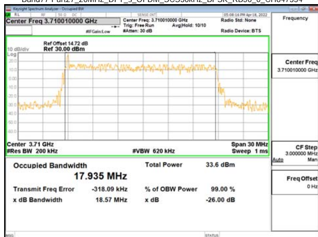
Band77-Part27_20MHz_DFT_s_OFDM_SCS30kHz_BPSK_RB50_0_CH647334
