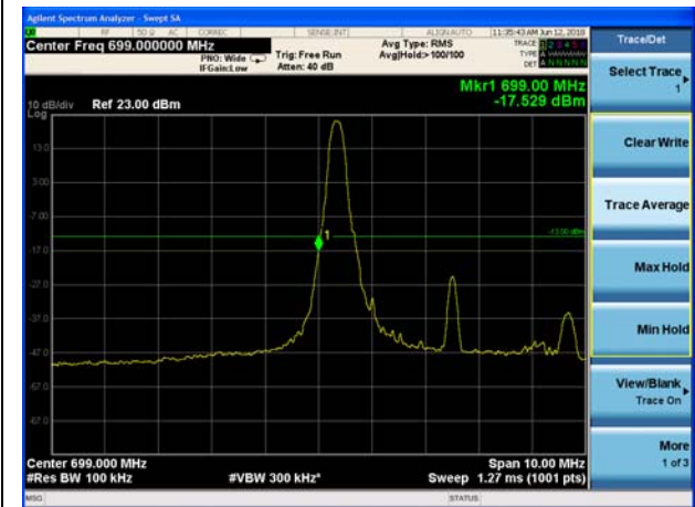
LTE Band 12 QPSK 5MHz CH-Low, 100%RB
