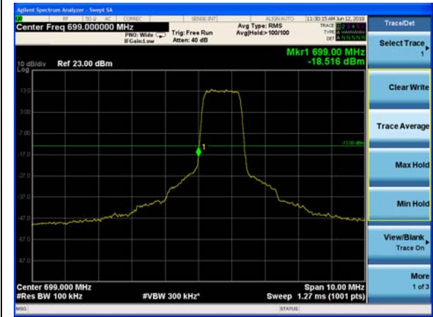
LTE Band 12 QPSK 1.4MHz CH-Low, 100%RB
