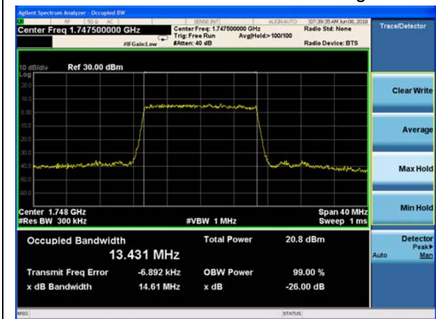
LTE Band 4 QPSK 15MHz CH-High
