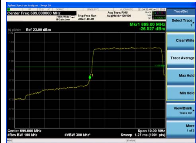
LTE Band 12 QPSK 10MHz CH-Low, 1 RB
