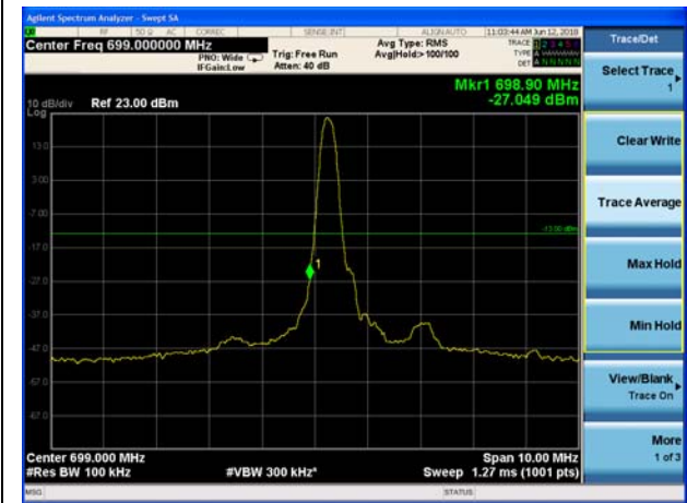
LTE Band 12 QPSK 1.4MHz CH-Low, 1 RB 698MHz~699MHz
