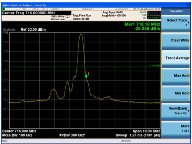
LTE Band 12 QPSK 1.4MHz CH-High, 1 RB 716MHz~717MHz
