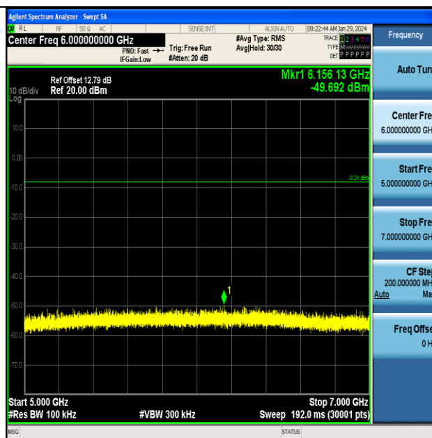
BLE_1M-Ant1-2402-5000~7000-PASS
