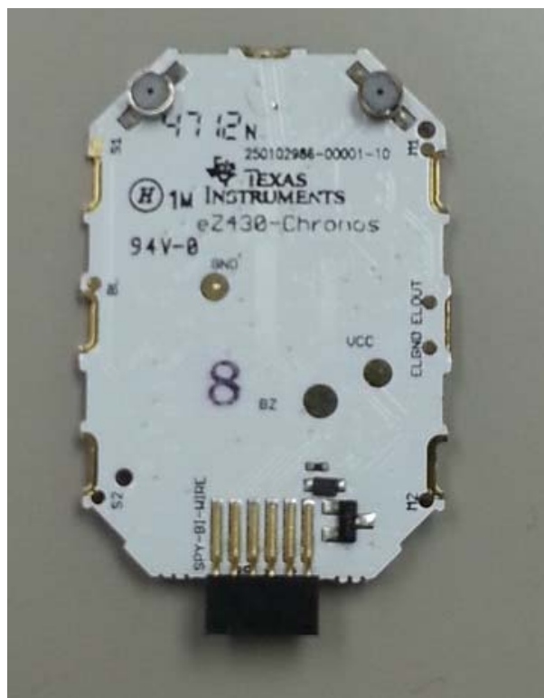
IrriGreen Programmer Printed Circuit Board Bottom
