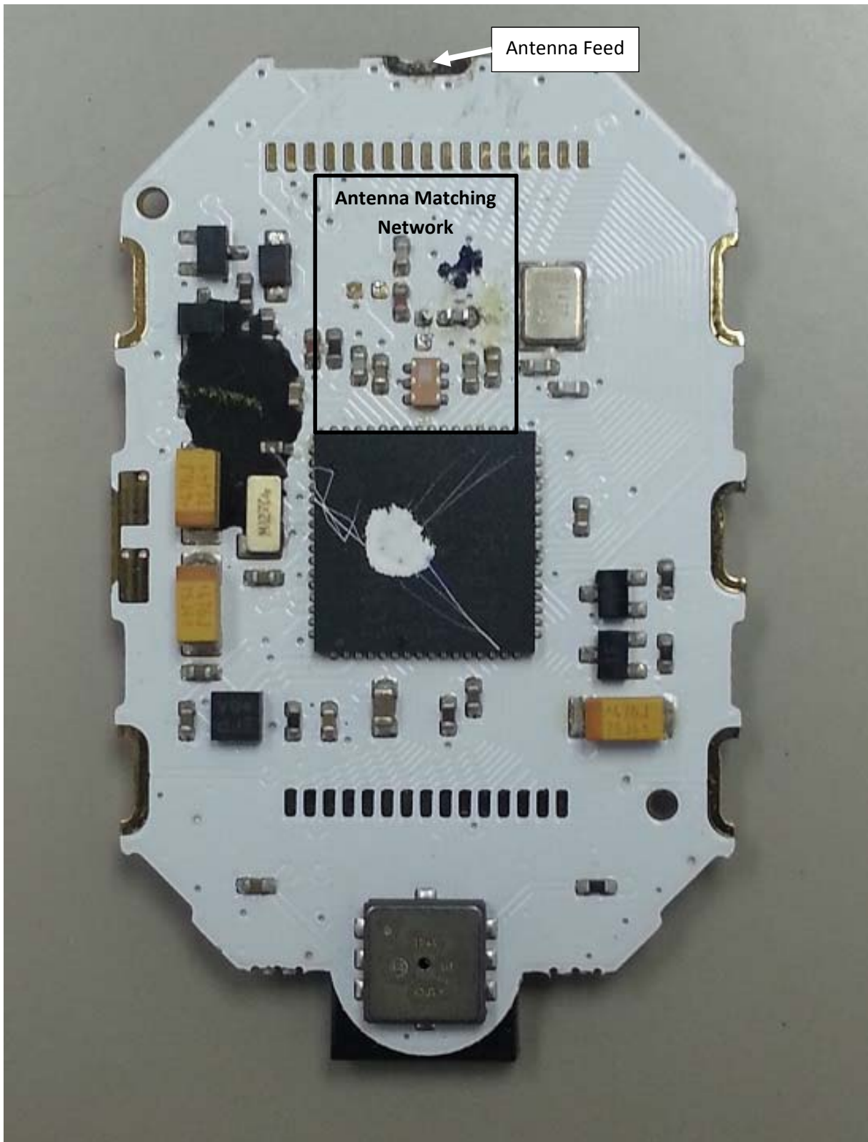
IrriGreen Programmer Printed Circuit Board Top
