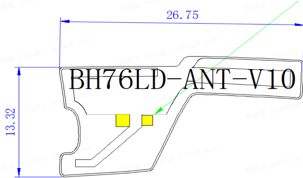
Antenna Dimensions
