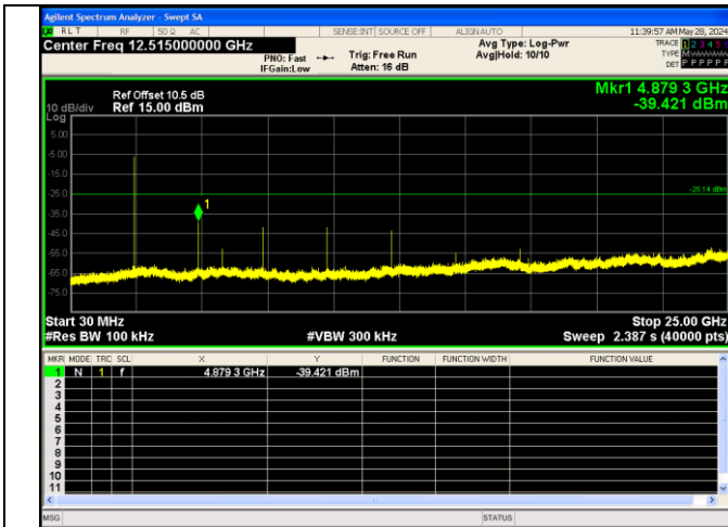
30.0 MHz - 25000.0 MHz LE_Channel 19
