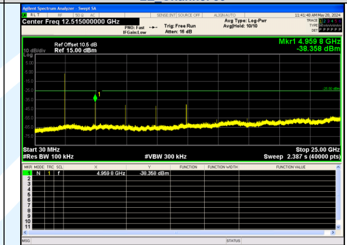
30.0 MHz - 25000.0 MHz LE_Channel 39
