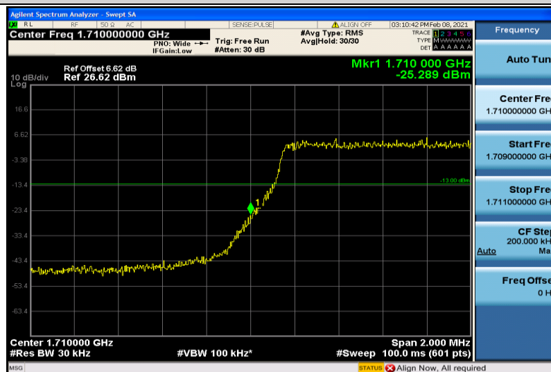
Band4-3MHz-16QAM-19965-6RB#0
