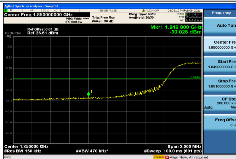
Band2-15MHz-16QAM-18675-6RB#0
