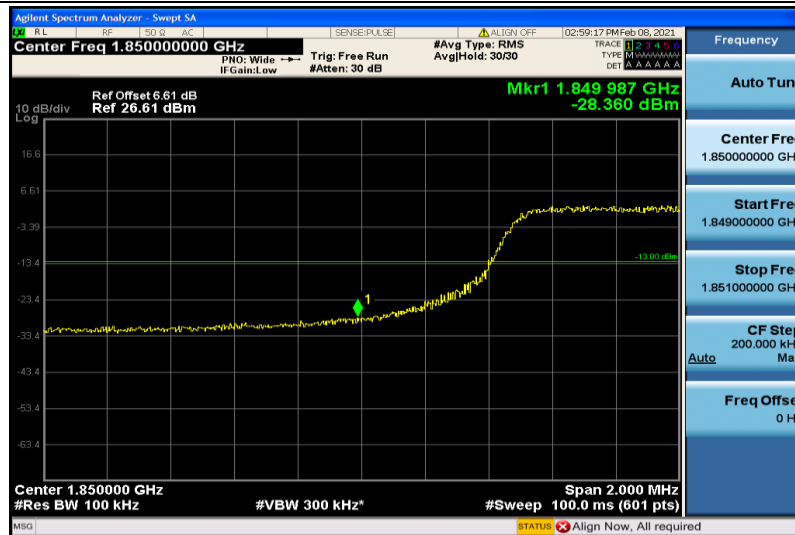
Band2-10MHz-16QAM-18650-6RB#0
