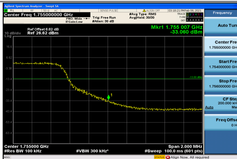
Band4-10MHz-16QAM-20350-6RB#0
