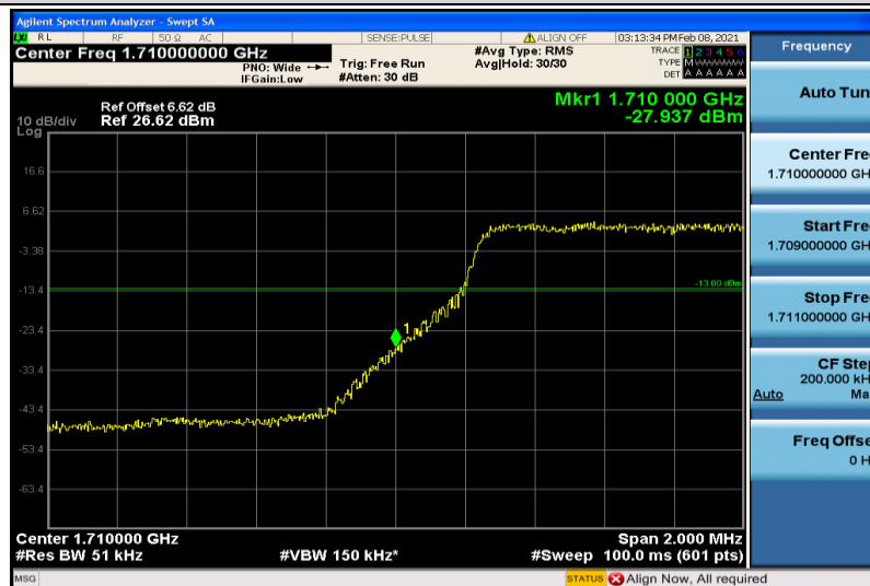
Band4-5MHz-16QAM-19975-6RB#0
