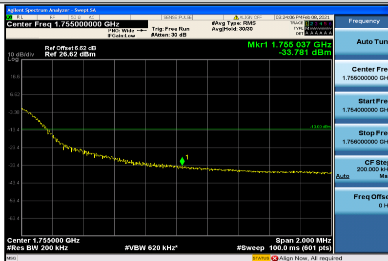
Band4-20MHz-QPSK-20300-6RB#0
