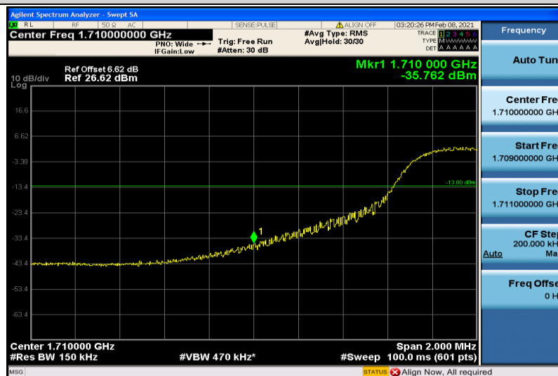
Band4-15MHz-16QAM-20025-6RB#0
