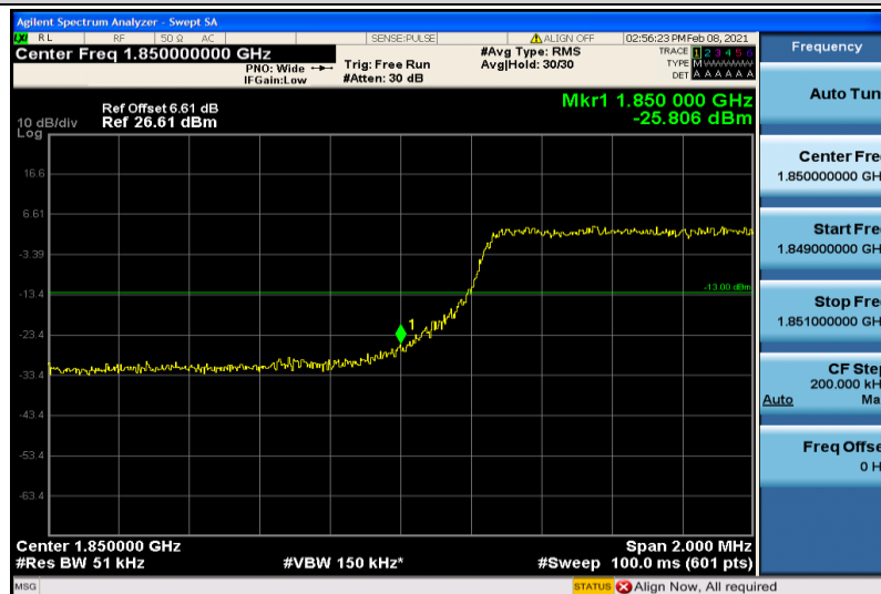
Band2-5MHz-16QAM-18625-6RB#0
