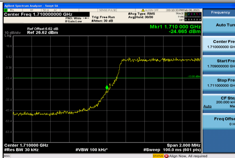
Band4-3MHz-QPSK-19965-6RB#0
