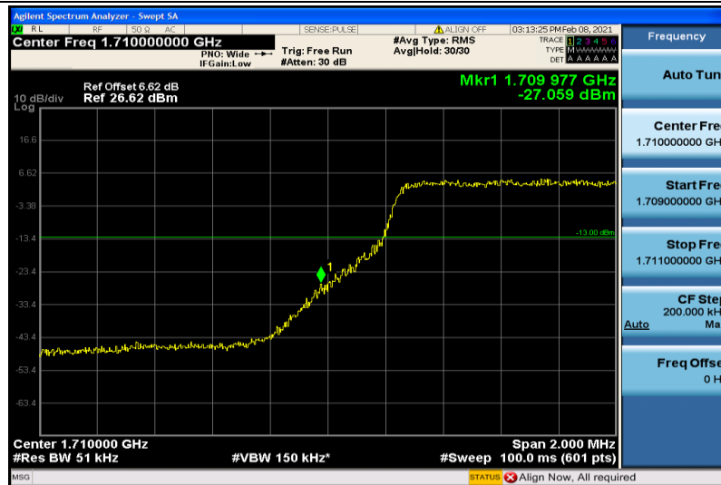
Band4-5MHz-QPSK-19975-6RB#0
