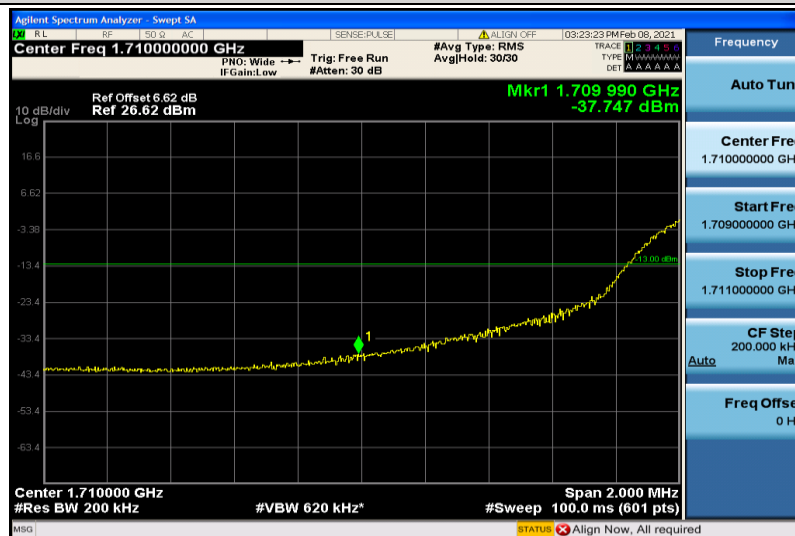
Band4-20MHz-16QAM-20050-6RB#0
