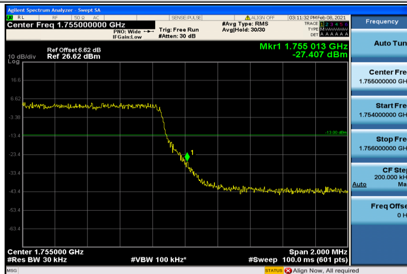
Band4-3MHz-16QAM-20385-6RB#0
