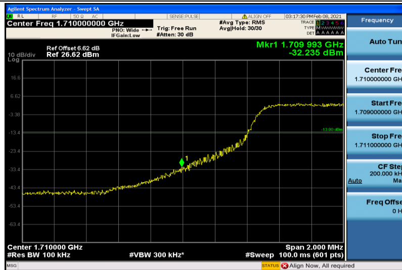
Band4-10MHz-16QAM-20000-6RB#0
