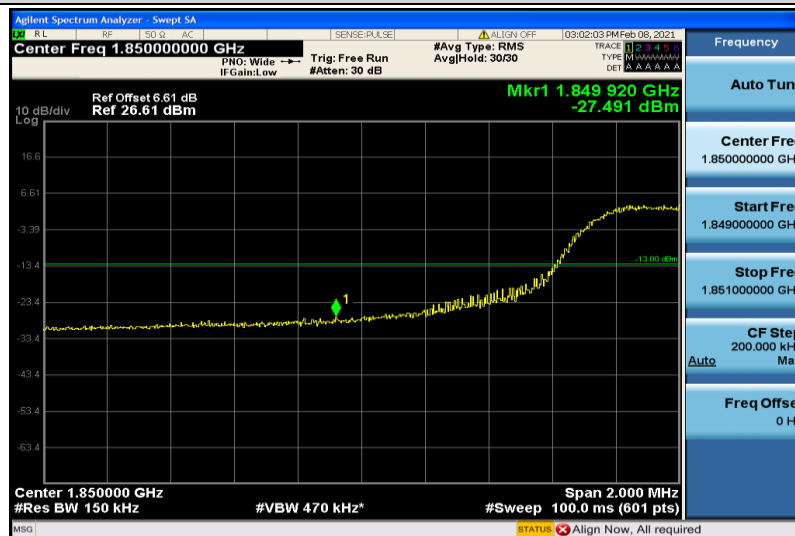
Band2-15MHz-QPSK-18675-6RB#0
