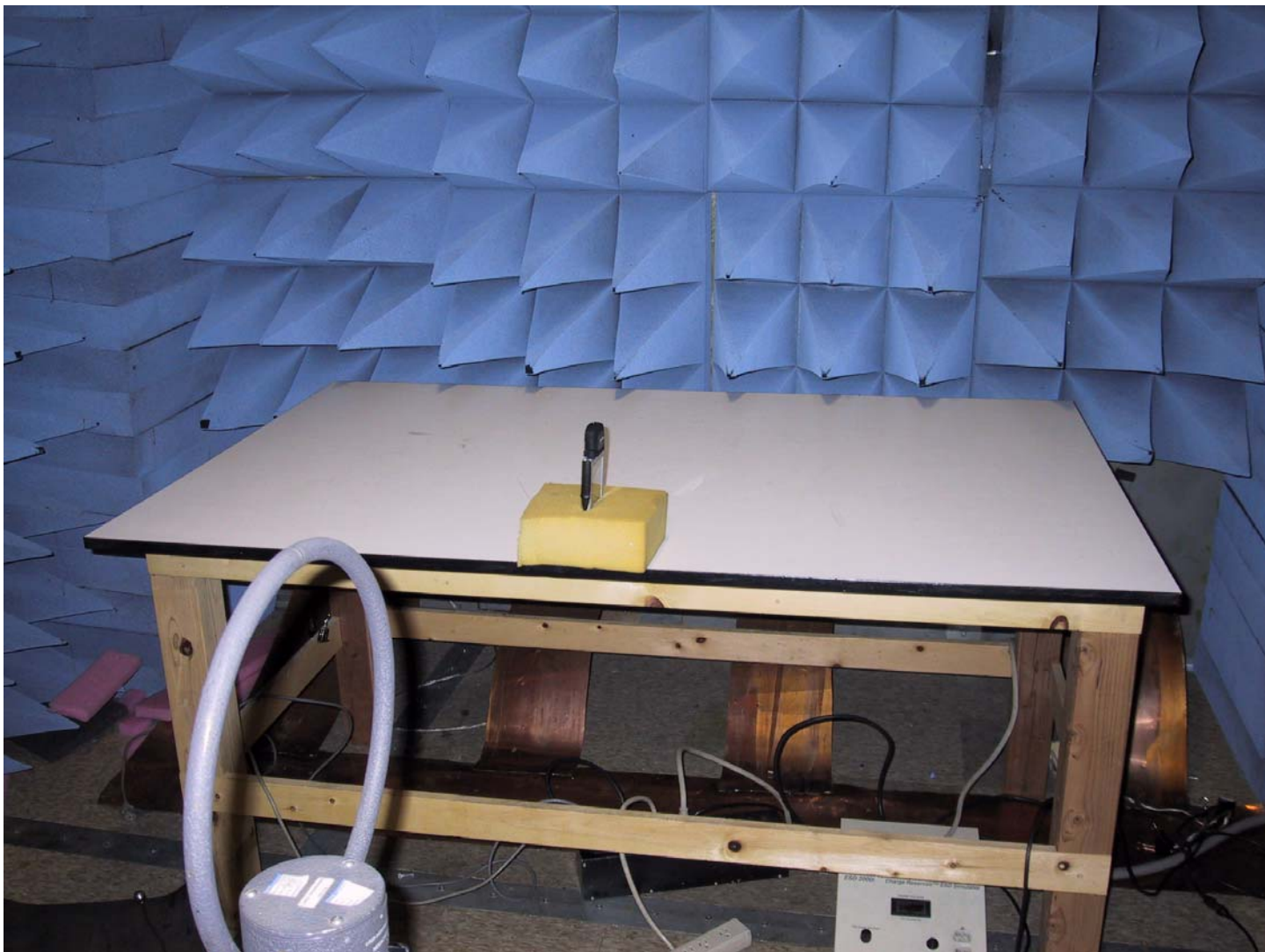
Intentional Radiator Emissions Test Setup
